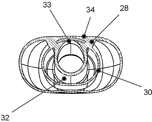
Figure 13 Section C-C
