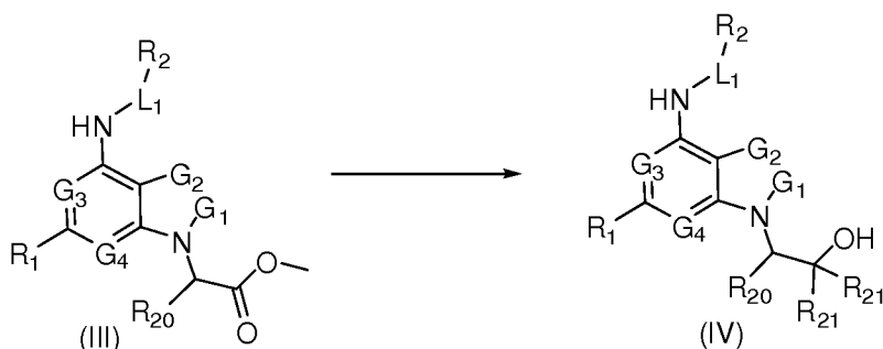
Reaction Scheme 5
