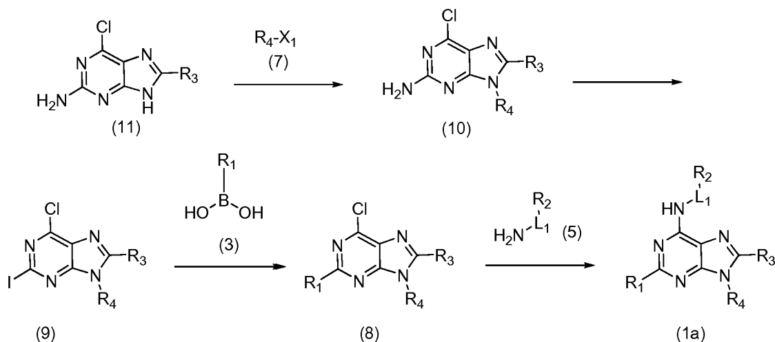
Reaction Scheme 2
