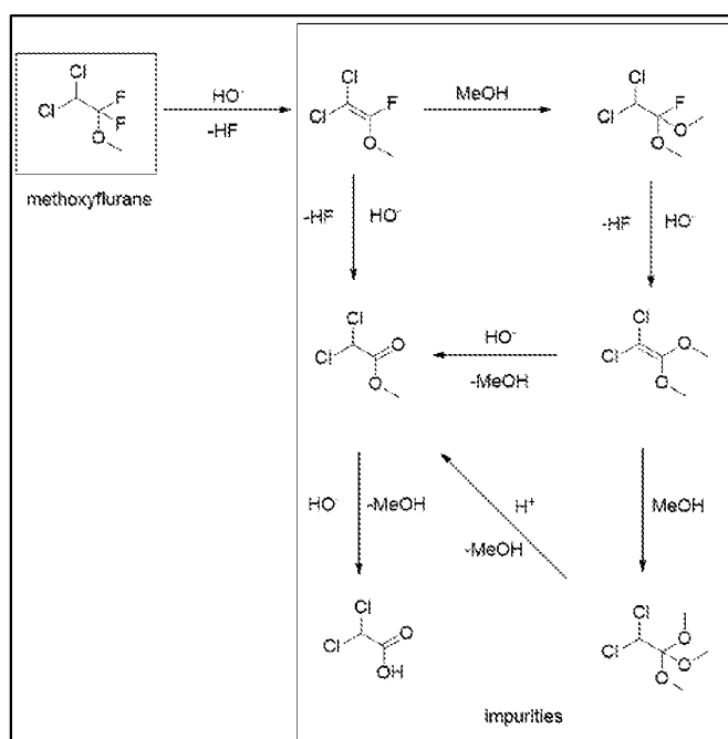
Scheme 2 Postulated mechanism of formation of impurities from methoxyflurane
