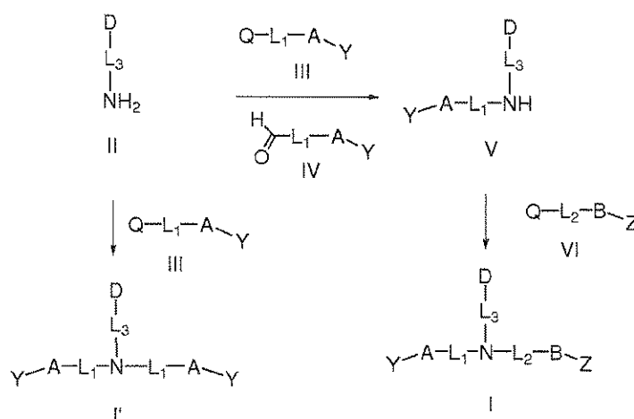
Scheme I
