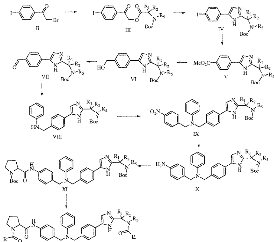
Scheme IV
