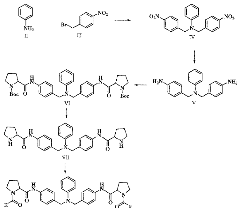
Scheme II
