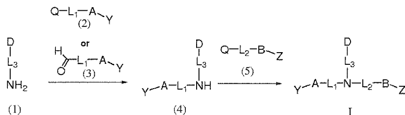
Scheme I'
