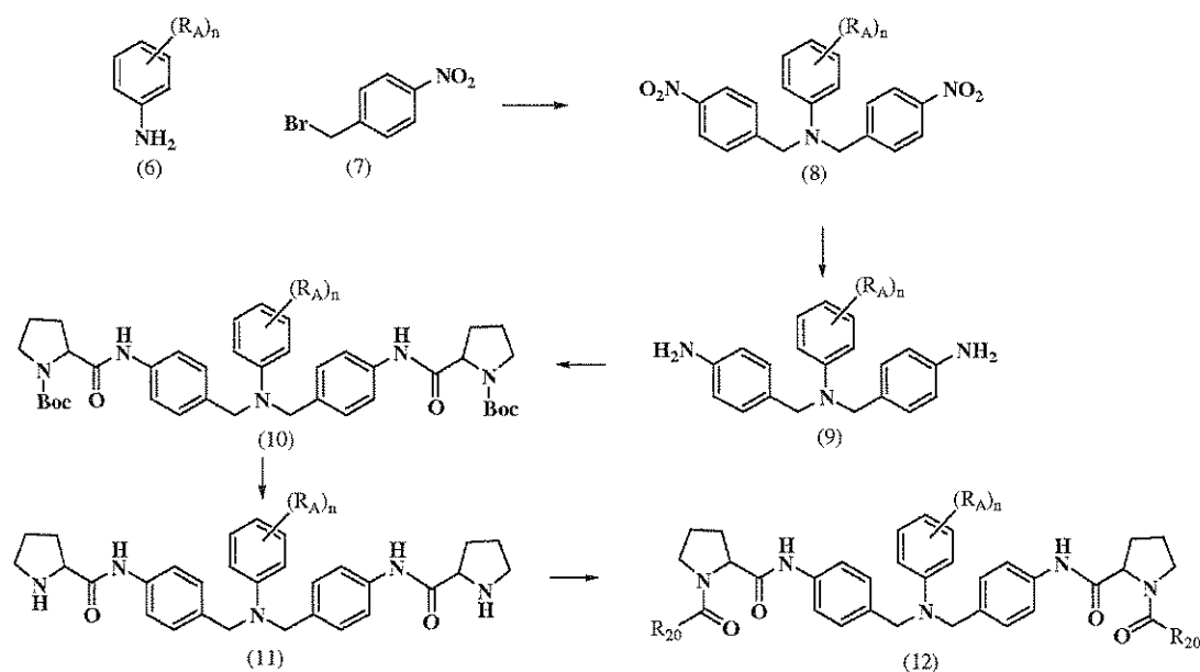
Scheme II'
