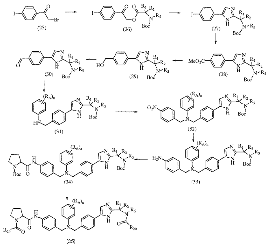
Scheme IV'
