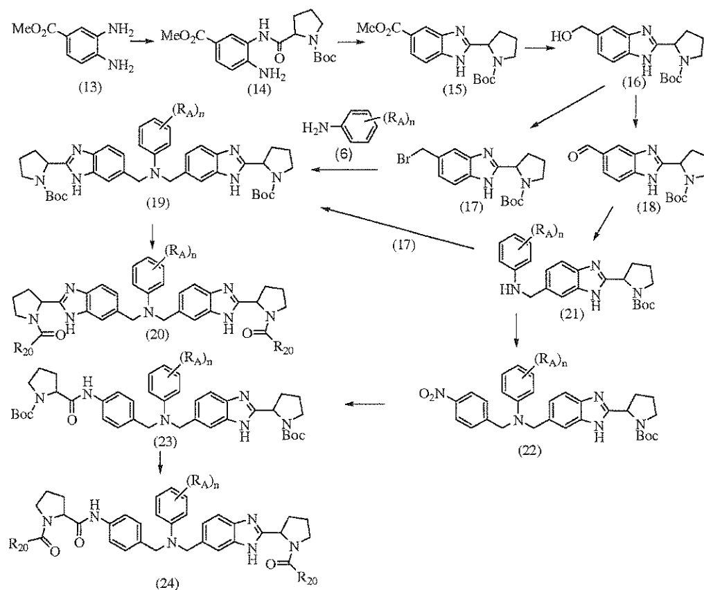
Scheme III'
