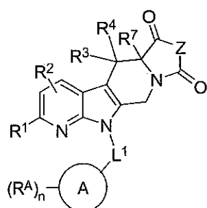
Formula (IV)
