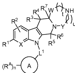
Formula (Ib)
