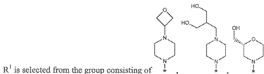
Formula I
