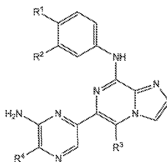
Formula I
