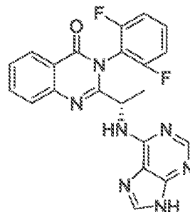
Compound C
