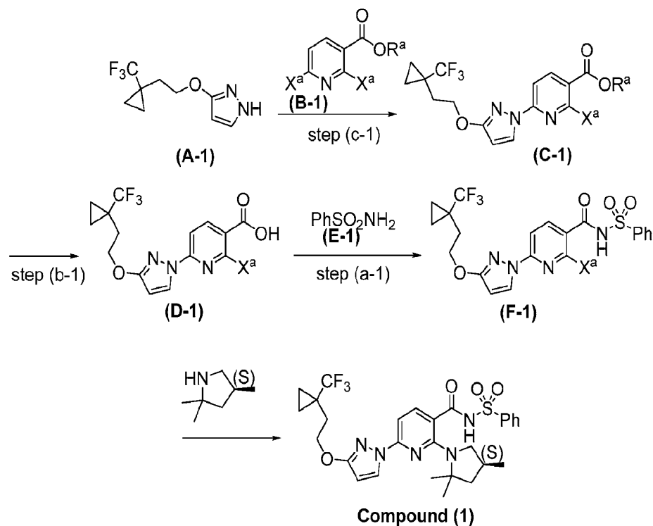
Scheme 4
