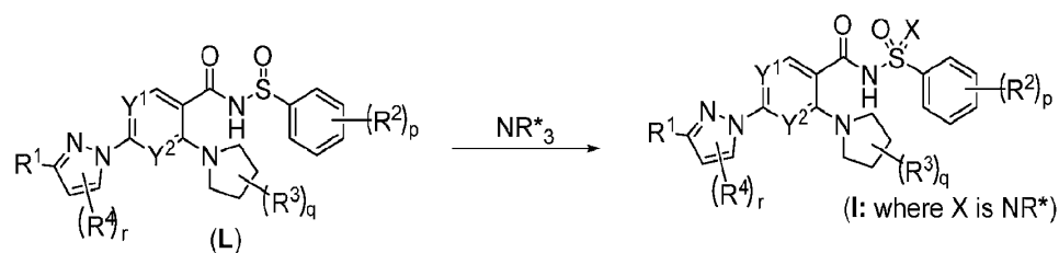
Scheme 5
