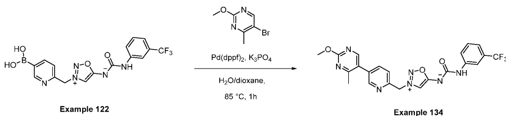
Scheme 23
