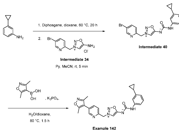
Scheme 27
