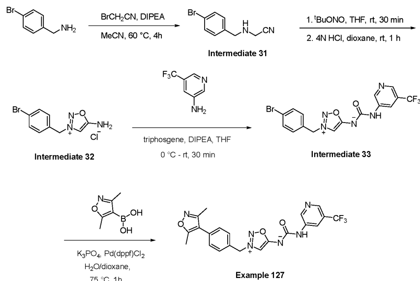
Scheme 21
