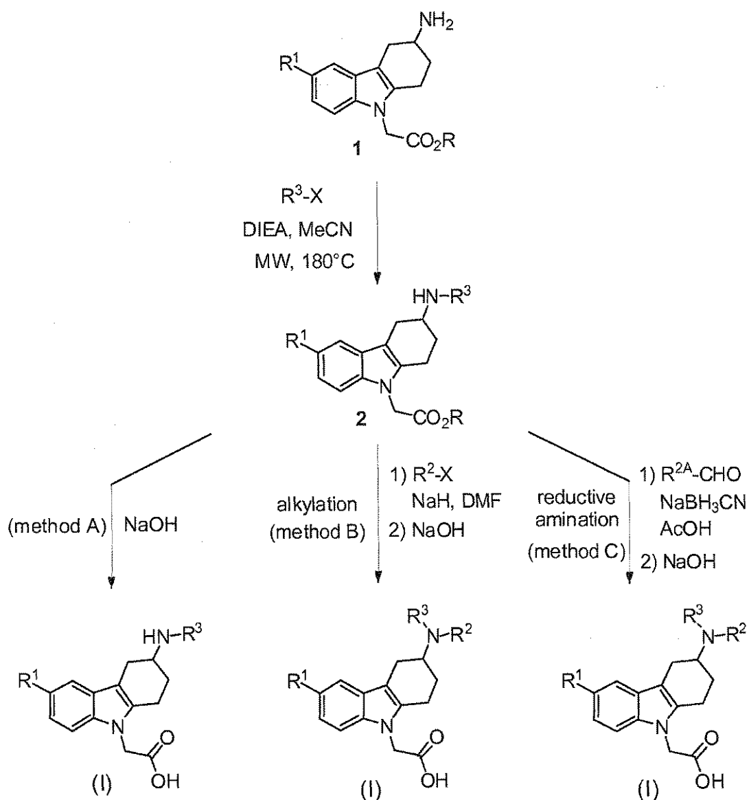
Scheme 1 (R represents (C 1 -C 4 )alkyl)
