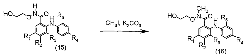
Scheme 8: Representative Preparation of Tertiary Benzamides by N-Alkylation
