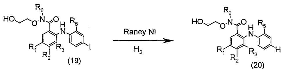
Scheme 10: Representative Hydrogenolysis of Aryl Iodides
