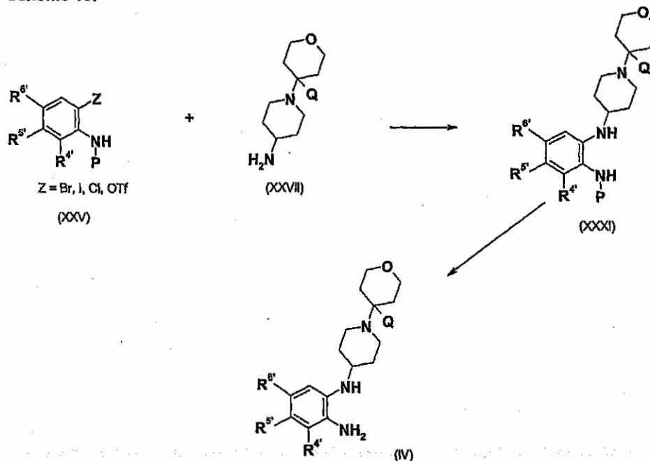
Scheme 10.
