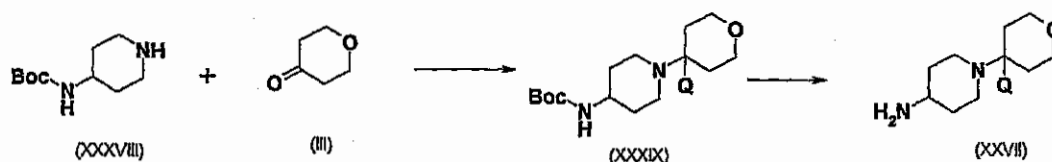
Scheme 15.
