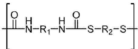
(Formula 12)
