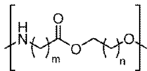
(Formula 14)
