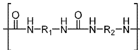
(Formula 11)
