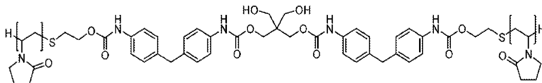
(Formula 9)
