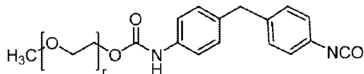
(Formula 4)
