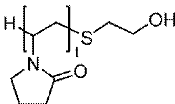
(Formula 5)
