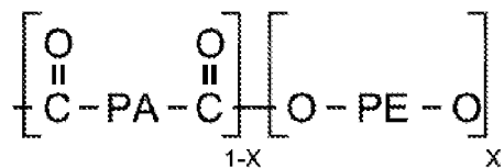
(Formula 16)
