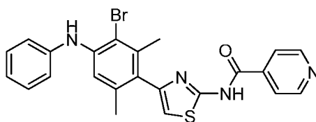
N -(4-(3-Bromo-2,6-dimethyl-4-(phenylamino)phenyl)thiazol-2-yl)isonicotinamide compound 123
