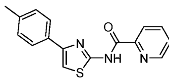
N -(4- p -Tolylthiazol-2-yl)picolinamide compound 28
