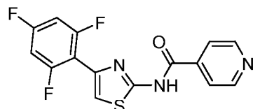
N-(4-(2,4,6-Trifluorophenyl)thiazol-2-yl)isonicotinamide compound 76
