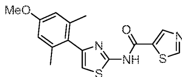
N-(4-(4-Methoxy-2,6-dimethylphenyl)thiazol-2-yl)thiazole-5-carboxamide compound 75
