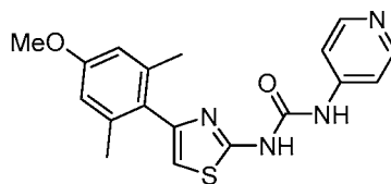
1-(4-(4-Methoxy-2,6-dimethylphenyl)thiazol-2-yl)-3-(pyridin-4-yl)urea compound 67
