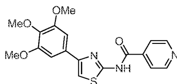
N -(4-(3,4,5-Trimethoxyphenyl)thiazol-2-yl)isonicotinamide compound 27
