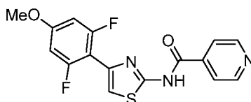
N -(4-(2,6-Difluoro-4-methoxyphenyl)thiazol-2-yl)isonicotinamide compound 78
