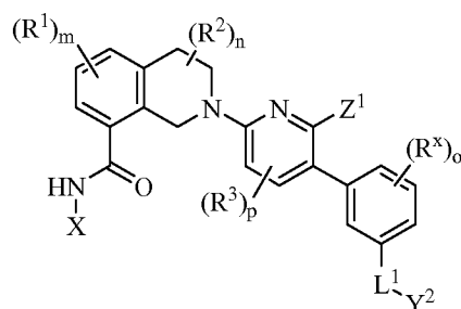
Formula (V),
