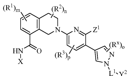
10 Formula (III)
