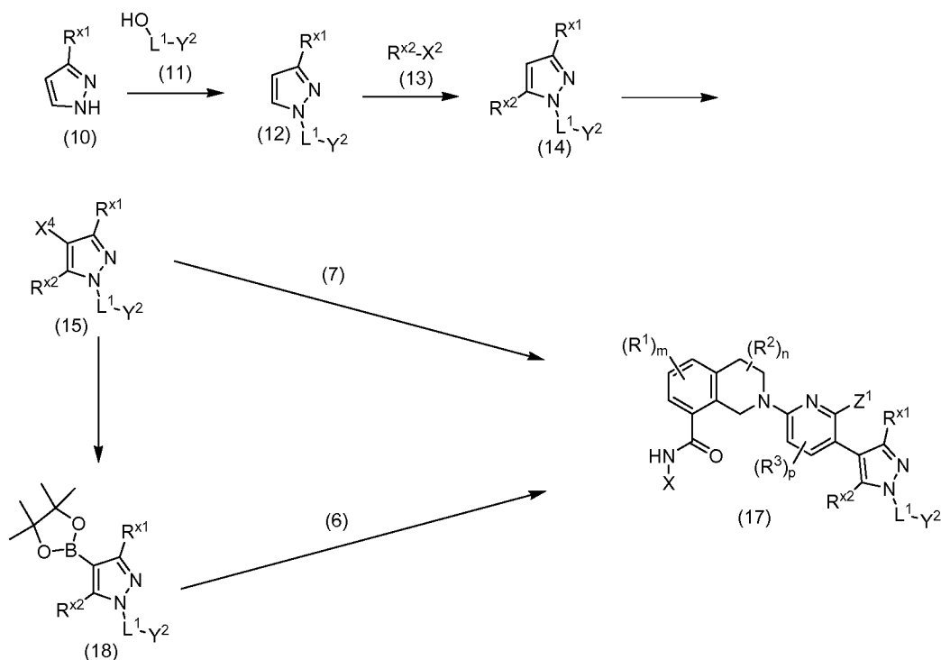
Scheme 3
