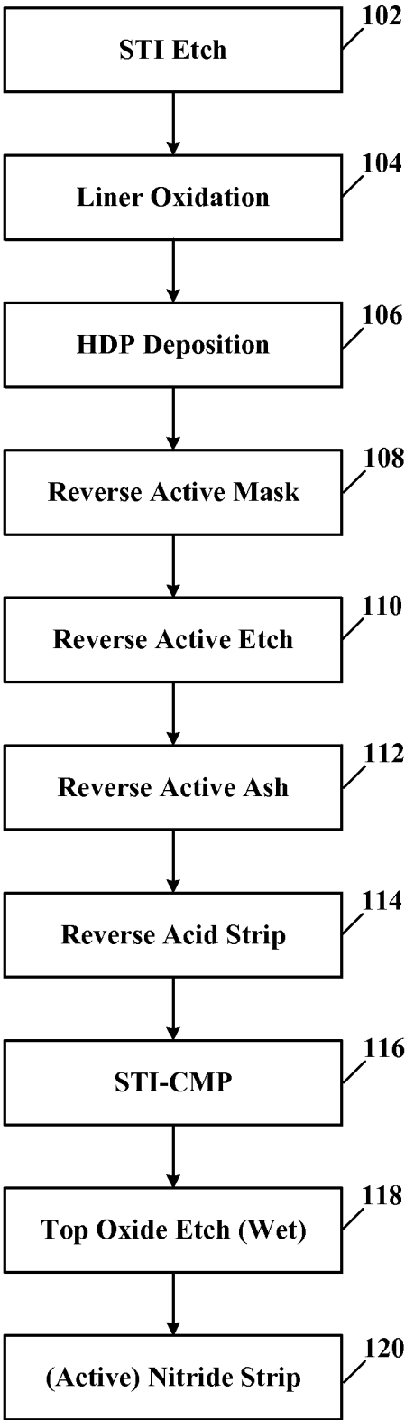
Figure 1 (Prior Art)
