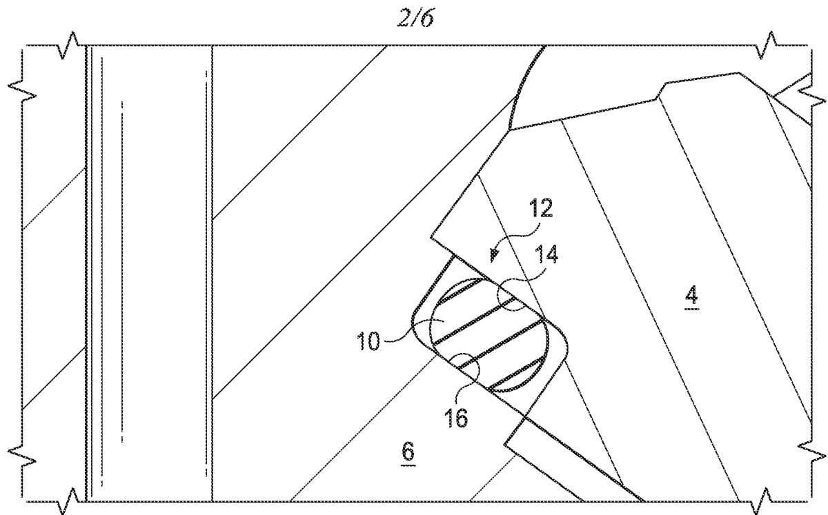
FIG. 2 (PRIOR ART)
