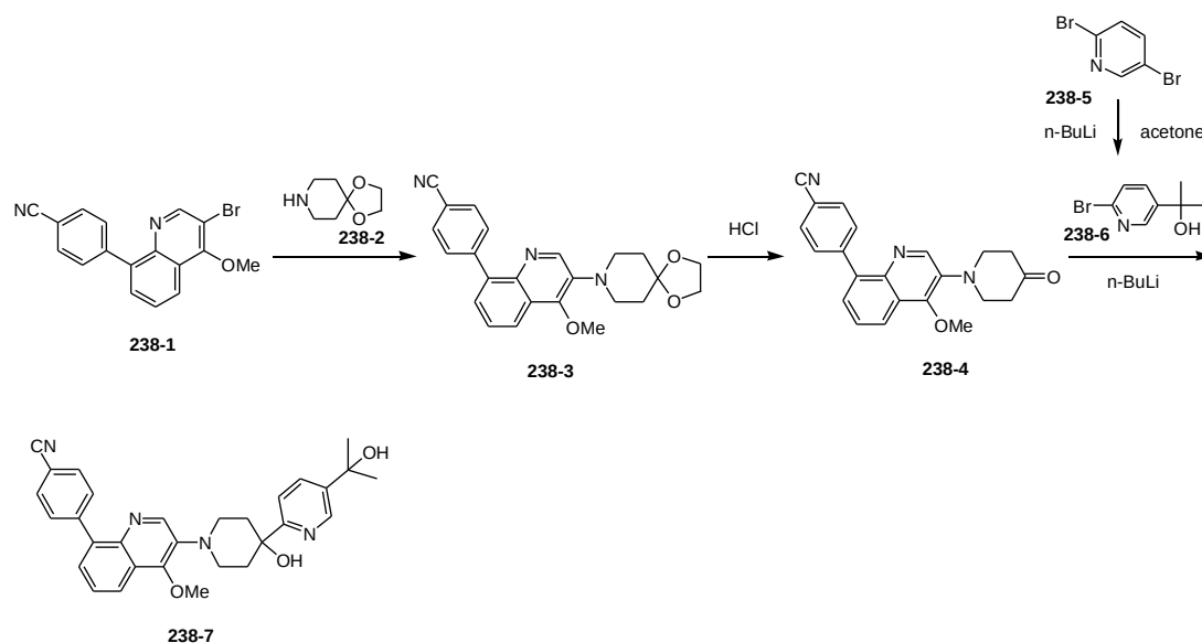
4-(3-(4-hydroxy-4-(5-(2-hydroxypropan-2-yl)pyridin-2-yl)piperidin-1-yl)-4-methoxyquinolin-8-yl)benzonitrile
