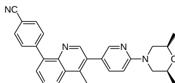
4-(3-(6-((2S,6R)-2,6-dimethylmorpholino)pyridin-3-yl)-4-methylquinolin-8-yl)benzonitrile
