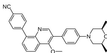
4-(3-(4-((2S,6R)-2,6-dimethylmorpholino)phenyl)-4-methoxyquinolin-8-yl)benzonitrile
