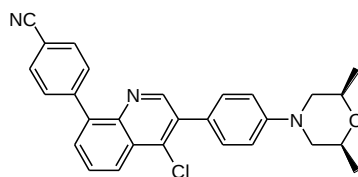
4-(4-chloro-3-(4-((2S,6R)-2,6-dimethylmorpholino)phenyl)quinolin-8-yl)benzonitrile
