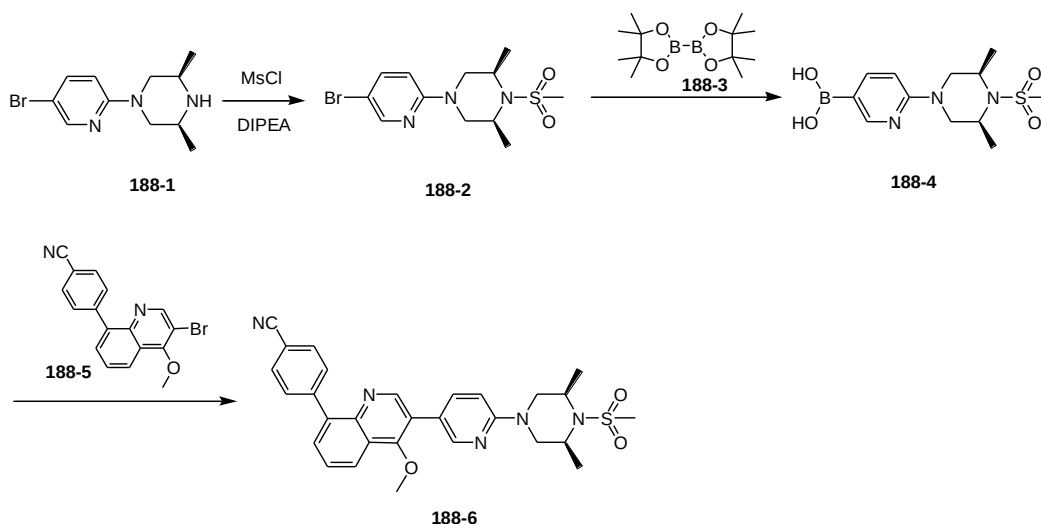
4-(3-(6-(4-methylsulfonyl-3,5-dimethylpiperazin-1-yl)pyridin-3-yl)-4-methoxyquinolin-8-yl)benzonitrile
