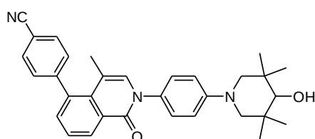
4-(2-(4-(4-hydroxy-3,3,5,5-tetramethylpiperidin-1-yl)phenyl)-4-methyl-1-oxo-1,2-dihydroisoquinolin-5-yl)benzonitrile
