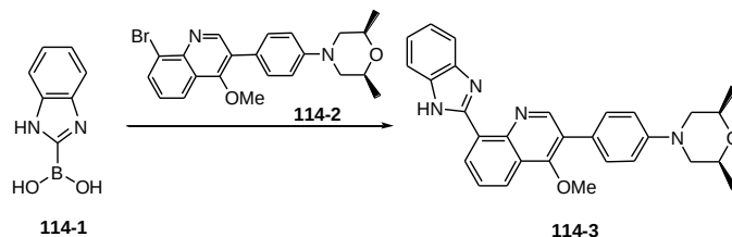
(2S,6R)-4-(4-(8-(1H-benzo[d]imidazol-2-yl)-4-methoxyquinolin-3-yl)phenyl)-2,6-dimethylmorpholine
