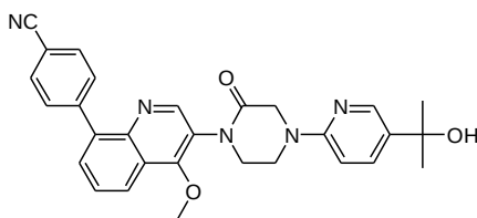
4-(3-(4-(5-(2-hydroxypropan-2-yl)pyridin-2-yl)-2-oxopiperazin-1-yl)-4-methoxyquinolin-8-yl)benzonitrile
