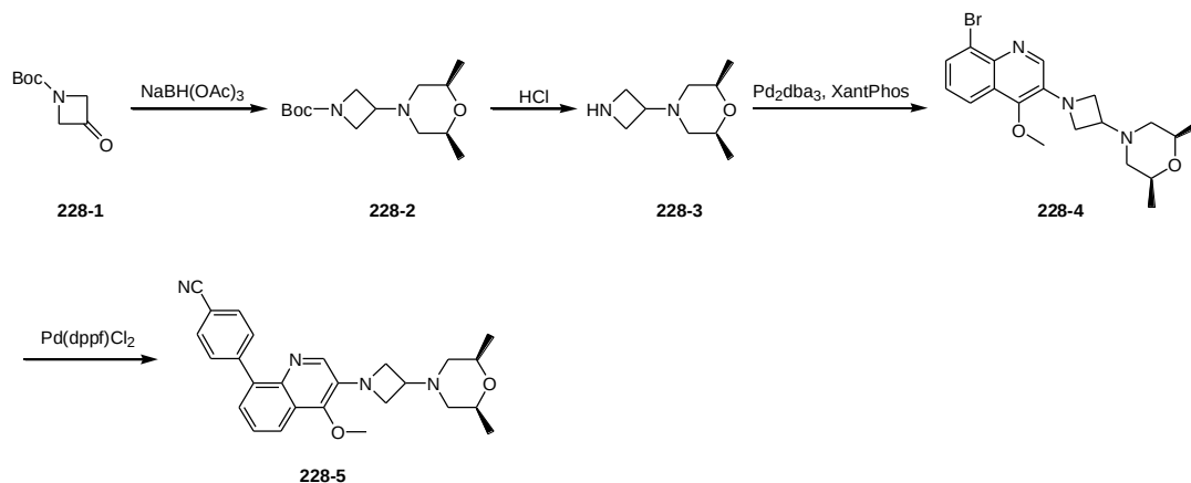
4-(3-(3-(2,6-dimethylmorpholino-4-yl)azetidin-1-yl)-4-methoxyquinolin-8-yl)benzonitrile
