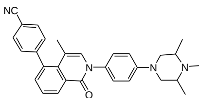
4-(4-methyl-1-oxo-2-(4-(3,4,5-trimethylpiperazin-1-yl)phenyl)-1,2-dihydroisoquinolin-5-yl)benzonitrile
