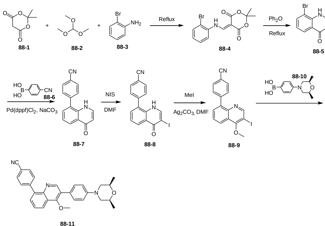
4-(3-(4-((2S,6R)-2,6-dimethylmorpholino)phenyl)-4-methoxyquinolin-8-yl)benzonitrile
