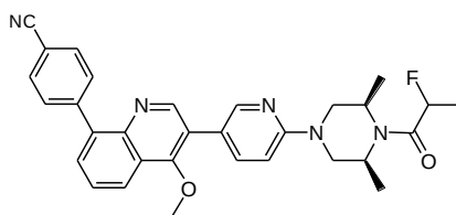
4-(3-(6-((3S, 5R)-4-(2-fluoropropanoyl)-3,5-dimethylpiperazin-1-yl)pyridin-3-yl)-4-methoxyquinolin-8-yl)benzonitrile
