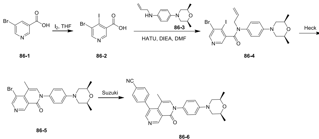
4-(7-(4-((2S,6R)-2,6-dimethylmorpholino)phenyl)-5-methyl-8-oxo-7,8-dihydro-2,7-naphthyridin-4-yl)benzonitrile
