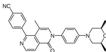
4-(6-(4-((2S,6R)-2,6-dimethylmorpholino)phenyl)-8-methyl-5-oxo-5,6-dihydro-2,6-naphthyridin-1-yl)benzonitrile
