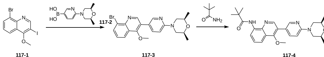
N-(3-(6-((2S,6R)-2,6-dimethylmorpholino)pyridin-3-yl)-4-methoxyquinolin-8-yl) pivalamide
