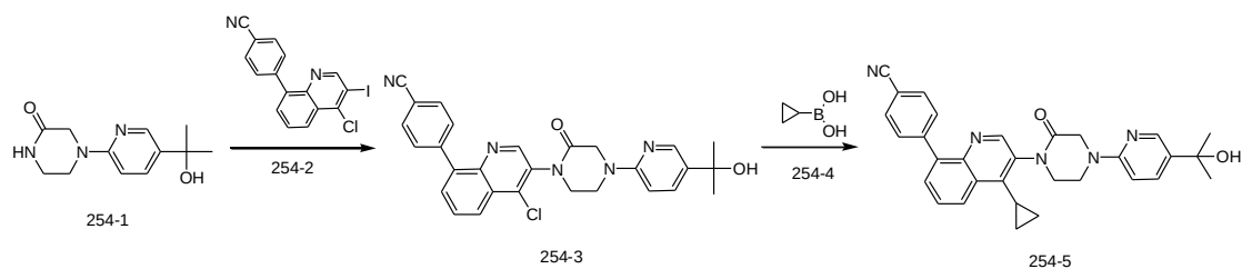
4-(4-cyclopropyl-3-(4-(5-(2-hydroxypropan-2-yl)pyridin-2-yl)-2-oxopiperazin-1-yl)quinolin-8-yl)benzonitrile
