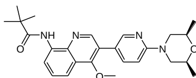
N-(3-(6-((2S,6R)-2,6-dimethylmorpholino)pyridin-3-yl)-4-methoxyquinolin-8-yl) pivalamide
