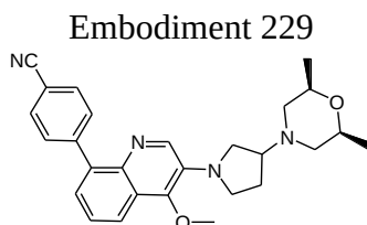
4-(3-(3-(2,6-dimethylmorpholino)pyrrolidin-1-yl)-4-methoxyquinolin-8-yl) benzonitrile
