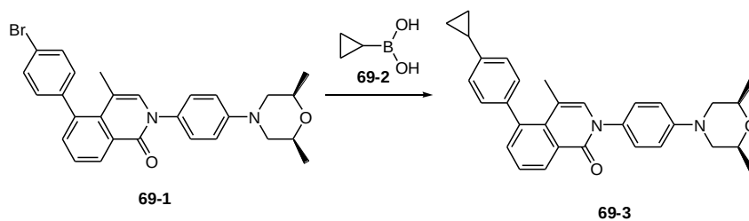
5-(4-cyclopropylphenyl)-2-(4-((2R,6S)-2,6-dimethylmorpholino)phenyl)-4-methylisoquinolin-1(2H)-one
