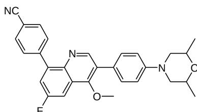
4-(3-(4-(2,6-dimethylmorpholino)phenyl)-6-fluoro-4-methoxyquinolin-8-yl) benzonitrile
