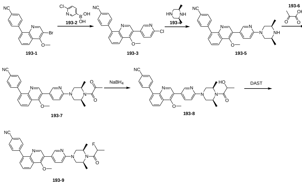
4-(3-(6-((3S, 5R)-4-(2-fluoropropanoyl)-3,5-dimethylpiperazin-1-yl)pyridin-3-yl)-4-methoxyquinolin-8-yl)benzonitrile
