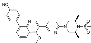
4-(3-(6-(4-methylsulfonyl-3,5-dimethylpiperazin-1-yl)pyridin-3-yl)-4-methoxyquinolin-8-yl)benzonitrile
