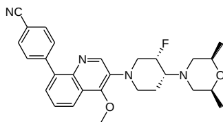
4-(3-(4-(2,6-dimethylmorpholino-4-yl)-3-fluoropiperidin-1-yl)-4-methoxyquinolin-8-yl)benzonitrile
