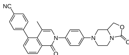
4-(4-methyl-1-oxo-2-(4-(3-oxotetrahydro-1H-oxazolo[3,4-a]pyrazin-7(3H)-yl)phenyl)-1,2-dihydroisoquinolin-5-yl)benzonitrile
