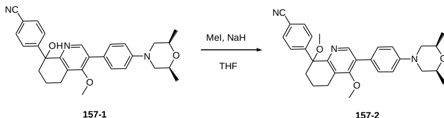
4-(3-(4-((2S,6R)-2,6-dimethylmorpholino)phenyl)-4,8-dimethoxy-5,6,7,8-tetrahydroquinolin-8-yl)benzonitrile
