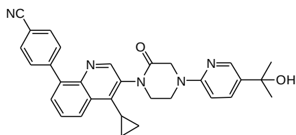
4-(4-cyclopropyl-3-(4-(5-(2-hydroxypropan-2-yl)pyridin-2-yl)-2-oxopiperazin-1-yl)quinolin-8-yl)benzonitrile
