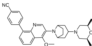
4-(3-(3-(2,6-dimethylmorpholino-4-yl)-8-azabicyclo[3.2.1]octan-8-yl)-4-methoxyquinolin-8-yl)benzonitrile
