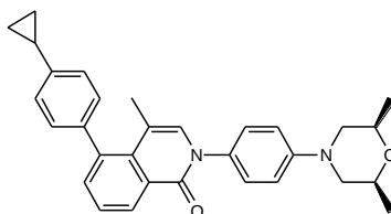
5-(4-cyclopropylphenyl)-2-(4-((2R,6S)-2,6-dimethylmorpholino)phenyl)-4-methylisoquinolin-1(2H)-one
