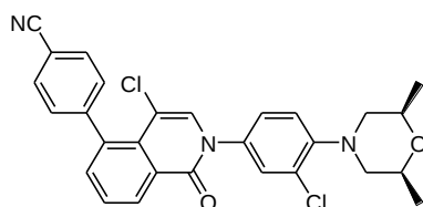
4-(4-chloro-2-(3-chloro-4-((2S,6R)-2,6-dimethylmorpholino)phenyl)-1-oxo-1,2-dihydroisoquinolin-5-yl)benzonitrile
