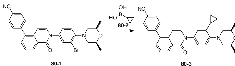
4-(2-(3-cyclopropyl-4-((2S,6R)-2,6-dimethylmorpholino)phenyl)-1-oxo-1,2-dihydroisoquinolin-5-yl)benzonitrile
