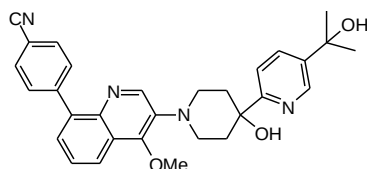
4-(3-(4-hydroxy-4-(5-(2-hydroxypropan-2-yl)pyridin-2-yl)piperidin-1-yl)-4-methoxyquinolin-8-yl)benzonitrile
