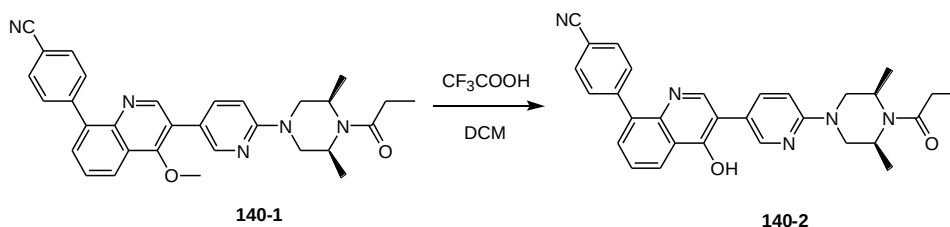
4-(3-(6-((3S,5R)-3,5-dimethyl-4-propionylpiperazin-1-yl)pyridin-3-yl)-4-hydroxyquinolin-8-yl)benzonitrile
