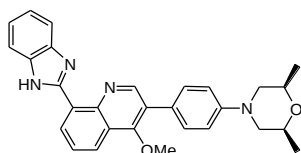
(2S,6R)-4-(4-(8-(1H-benzo[d]imidazol-2-yl)-4-methoxyquinolin-3-yl)phenyl)-2,6-dimethylmorpholine
