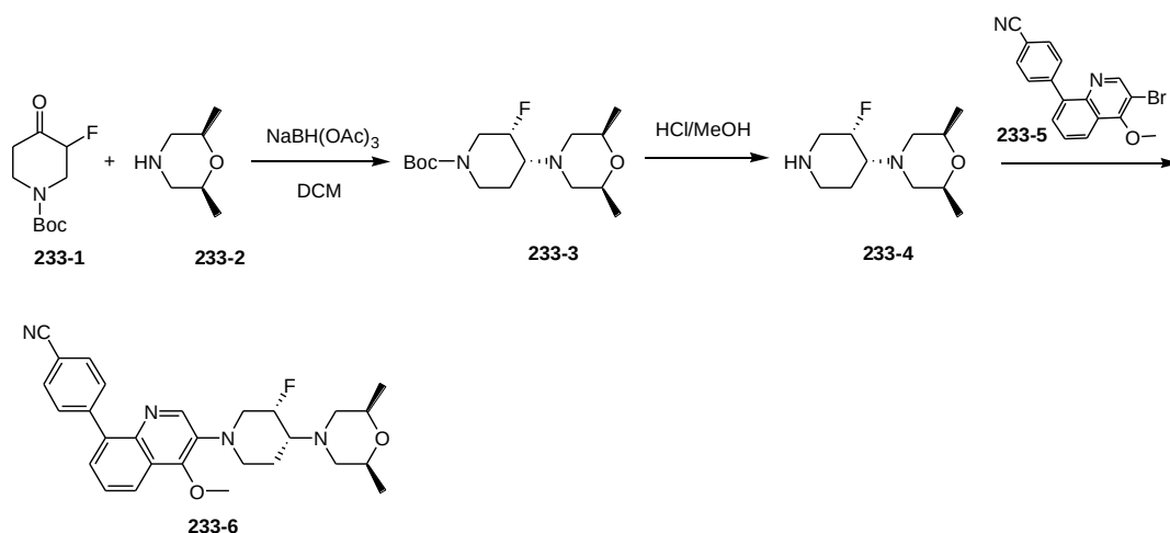
4-(3-(4-(2,6-dimethylmorpholino-4-yl)-3-fluoropiperidin-1-yl)-4-methoxyquinolin-8-yl)benzonitrile
