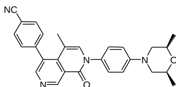
4-(7-(4-((2S,6R)-2,6-dimethylmorpholino)phenyl)-5-methyl-8-oxo-7,8-dihydro-2,7-naphthyridin-4-yl)benzonitrile
