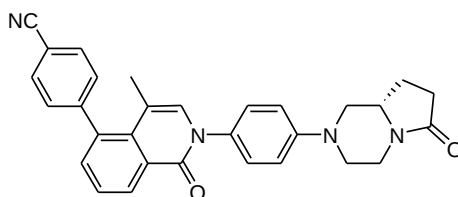
(S)-4-(4-methyl-1-oxo-2-(4-(6-oxo-hexahydropyrrolo[1,2-a]pyrazin-2(1H)-yl)phenyl)-1,2-dihydroisoquinolin-5-yl)benzonitrile
