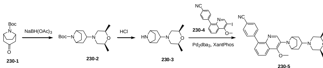
4-(3-(3-(2,6-dimethylmorpholino-4-yl)-8-azabicyclo[3.2.1]octan-8-yl)-4-methoxyquinolin-8-yl)benzonitrile
