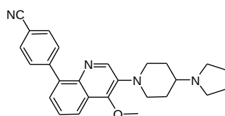
4-(4-methoxy-3-(4-(pyrrolidin-1-yl)piperidin-1-yl)quinolin-8-yl)benzonitrile
