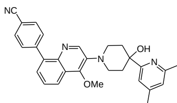
4-(3-(4'-hydroxy-4,6-dimethyl-3',4',5',6'-tetrahydro-2'H-[2,4'] bipyridyl-1'-yl)-4-methoxyquinolin-8-yl)benzonitrile
