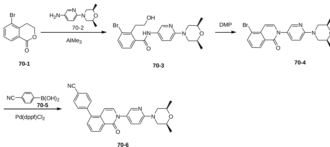
4-(2-(6-(2,6-dimethylmorpholino-4-yl)pyridin-3-yl)-1-oxo-1,2-dihydroisoquinolin-5-yl)benzonitrile
