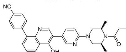
4-(3-(6-((3S,5R)-3,5-dimethyl-4-propionylpiperazin-1-yl)pyridin-3-yl)-4-hydroxyquinolin-8-yl)benzonitrile
