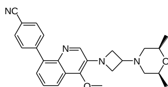
4-(3-(3-(2,6-dimethylmorpholino-4-yl)azetidin-1-yl)-4-methoxyquinolin-8-yl)benzonitrile
