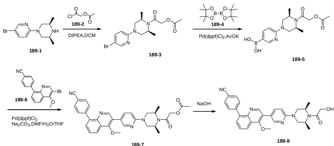
4-(3-(6-(4-(2-hydroxyacetyl)-3,5-dimethylpiperazin-1-yl)pyridin-3-yl)-4-methoxyquinolin-8-yl)benzonitrile
