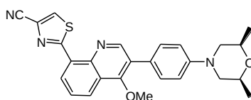
2-(3-(4-((2S,6R)-2,6-dimethylmorpholino)phenyl)-4-methoxyquinolin-8-yl)thiazole-4-carbonitrile
