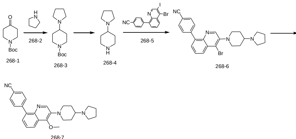
4-(4-methoxy-3-(4-(pyrrolidin-1-yl)piperidin-1-yl)quinolin-8-yl)benzonitrile
