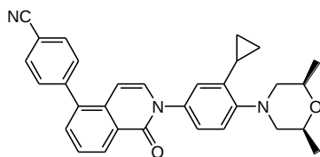
4-(2-(3-cyclopropyl-4-((2S,6R)-2,6-dimethylmorpholino)phenyl)-1-oxo-1,2-dihydroisoquinolin-5-yl)benzonitrile
