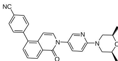
4-(2-(6-(2,6-dimethylmorpholino-4-yl)pyridin-3-yl)-1-oxo-1,2-dihydroisoquinolin-5-yl)benzonitrile
