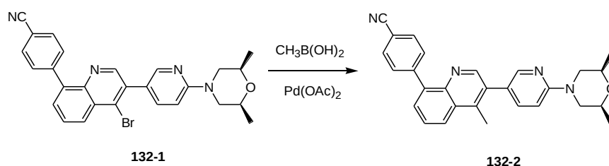
4-(3-(6-((2S,6R)-2,6-dimethylmorpholino)pyridin-3-yl)-4-methylquinolin-8-yl)benzonitrile
