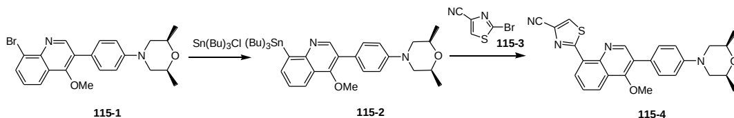
2-(3-(4-((2S,6R)-2,6-dimethylmorpholino)phenyl)-4-methoxyquinolin-8-yl)thiazole-4-carbonitrile
