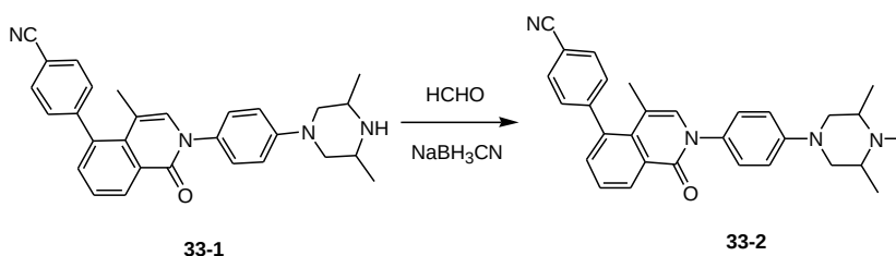
4-(4-methyl-1-oxo-2-(4-(3,4,5-trimethylpiperazin-1-yl)phenyl)-1,2-dihydroisoquinolin-5-yl)benzonitrile
