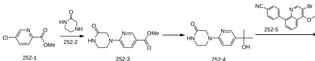
4-(3-(4-(5-(2-hydroxypropan-2-yl)pyridin-2-yl)-2-oxopiperazin-1-yl)-4-methoxyquinolin-8-yl)benzonitrile
