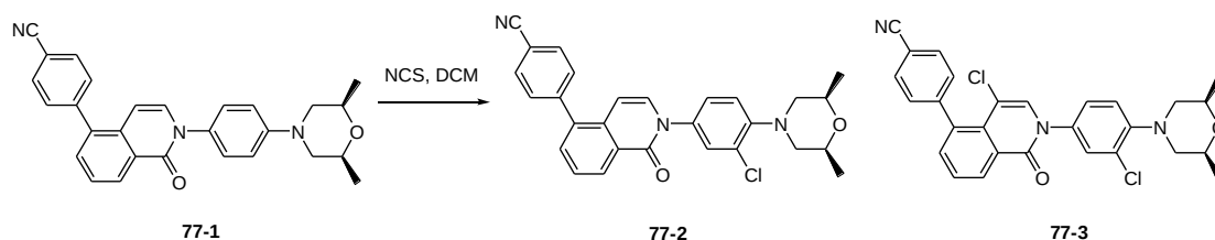
4-(4-chloro-2-(3-chloro-4-((2S,6R)-2,6-dimethylmorpholino)phenyl)-1-oxo-1,2-dihydroisoquinolin-5-yl)benzonitrile
