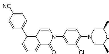
4-(2-(3-chloro-4-((2S,6R)-2,6-dimethylmorpholino)phenyl)-1-oxo-1,2-dihydroisoquinolin-5-yl)benzonitrile
