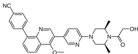
4-(3-(6-(4-(2-hydroxyacetyl)-3,5-dimethylpiperazin-1-yl)pyridin-3-yl)-4-methoxyquinolin-8-yl)benzonitrile
