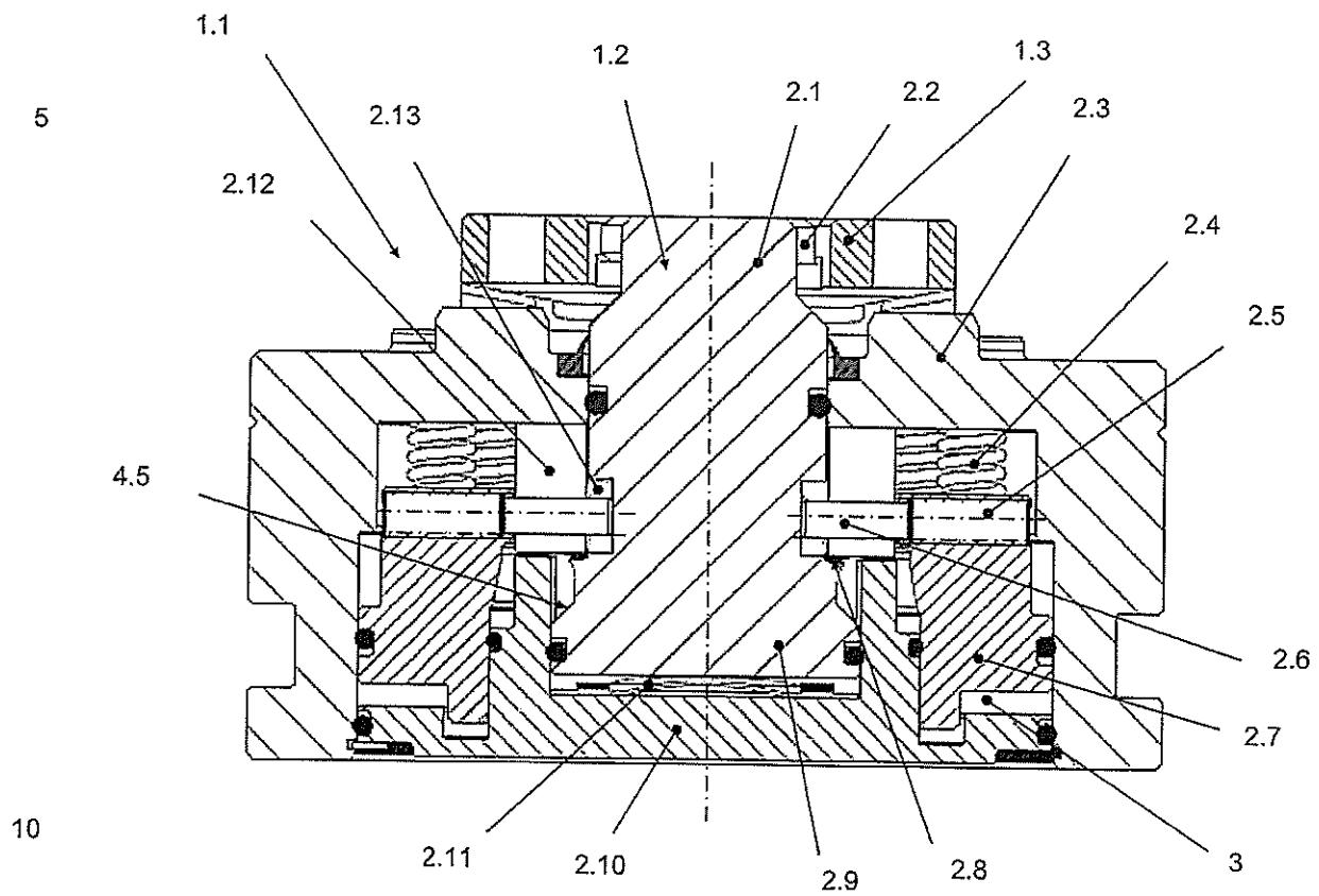
Fig 2. Cross-section of the clamping chuck and pallet
