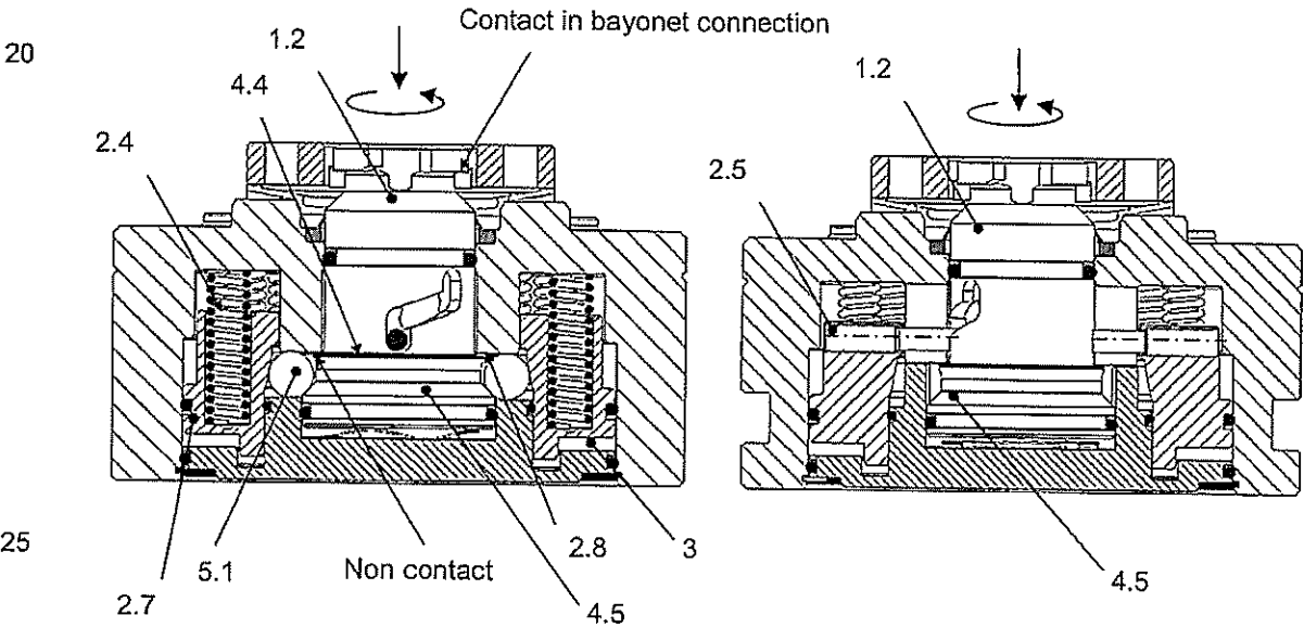
30 Fig 6b. Clamping chuck with drawbar in clamped position, cross section in 0 degree and 90 degree view
