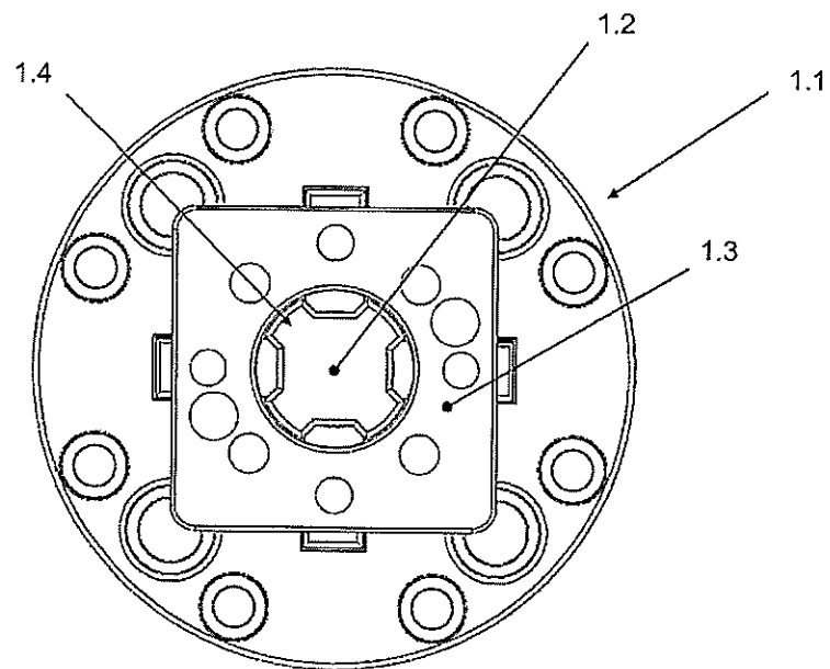
20 Fig 1b. Top-view of the clamping chuck and pallet, drawbar in locked position
