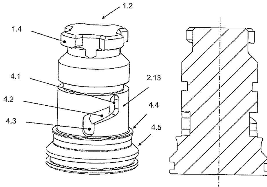
Fig 4a. Drawbar with S-shaped spiral guiding grooves
