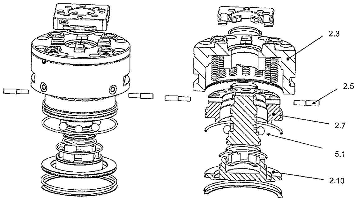
15 Fig 5. Clamping chuck complete, "exploded" view and cross-section for visualization
