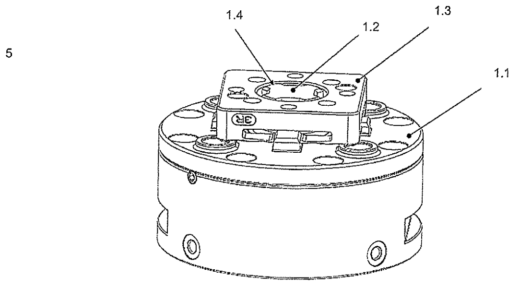
10 Fig 1a. 3D-view of the clamping chuck and pallet
