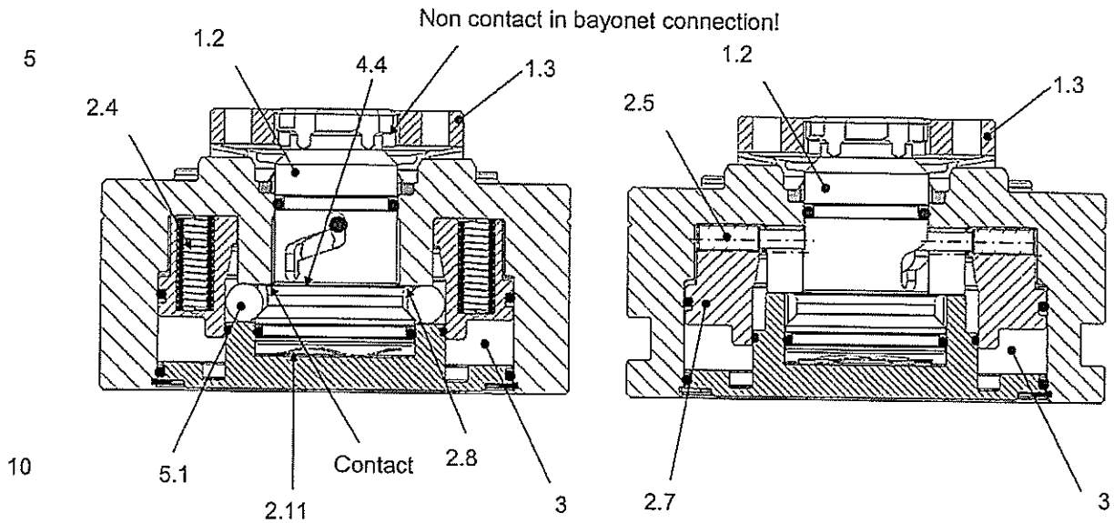
15 Fig 6a. Clamping chuck with drawbar in open position, cross section in 0 degree and 90 degree
