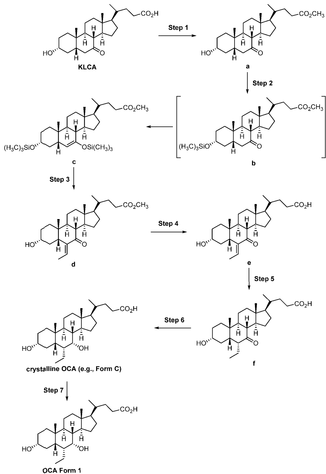
Scheme 1
