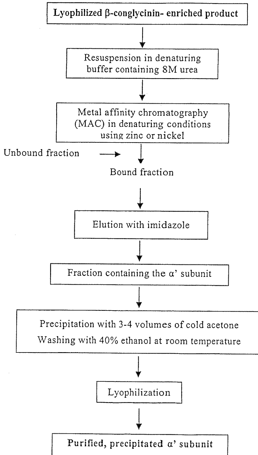
Figure 2 \alpha' SUBUNIT
