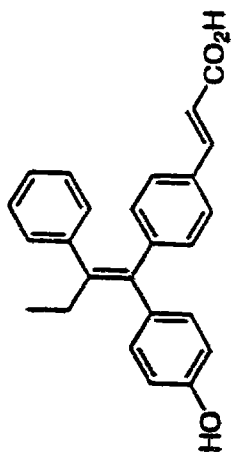
GW 7604
