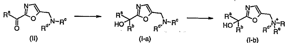
Scheme 5
