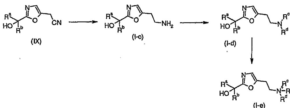
20 Scheme 7
