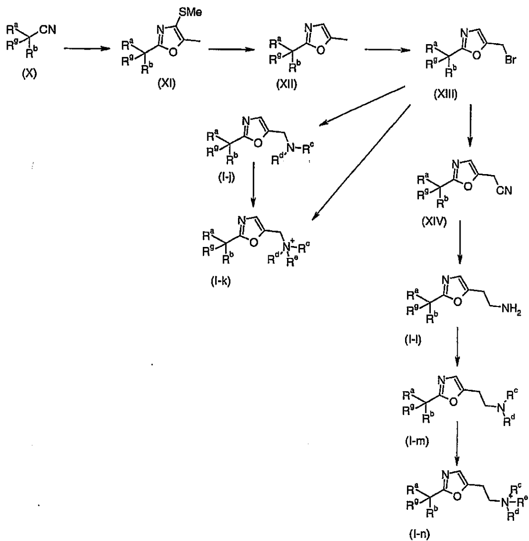
Scheme 2
