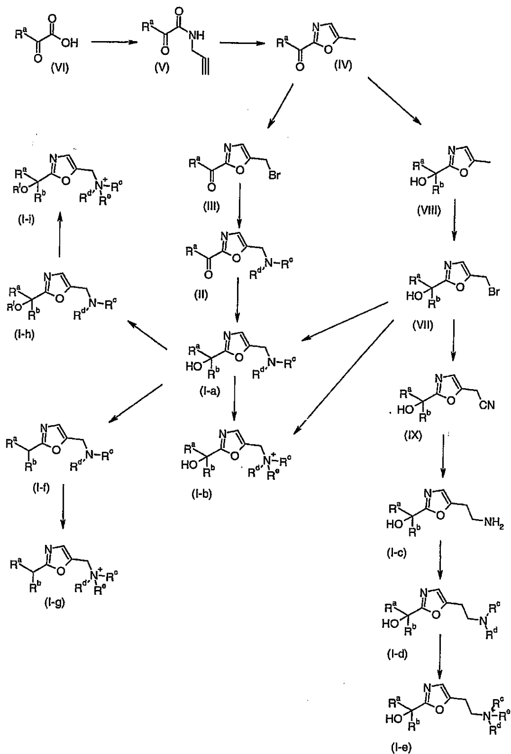
Scheme 1
