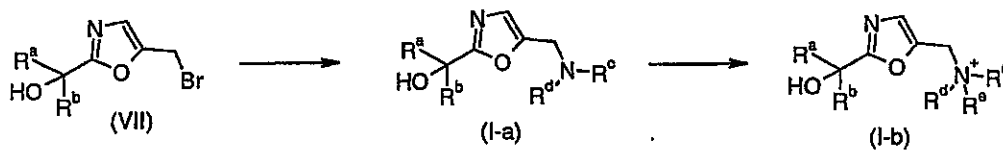
10 Scheme 6
