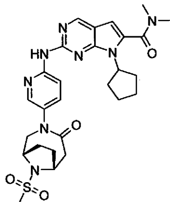
7-cyclopentyl-N,N-dimethyl-2-(5-((1S,6R)-9-(methylsulfonyl)-4-oxo-3,9-diazabicyclo[4.2.1]nonan-3-yl)pyridin-2-ylamino)-7H-pyrrolo[2,3-d]pyrimidine-6-carboxamide
