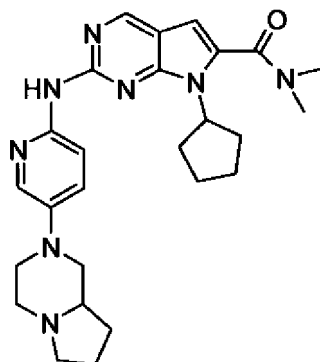
7-cyclopentyl-2-(5-(hexahydropyrrolo[1,2-a]pyrazin-2(1H)-yl)pyridin-2-ylamino)-N,N-dimethyl-7H-pyrrolo[2,3-d]pyrimidine-6-carboxamide
