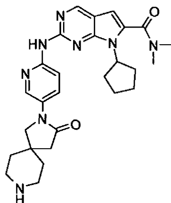
7-cyclopentyl-N,N-dimethyl-2-(5-(1-oxo-2,8-diazaspiro[4.5]decan-2-yl)pyridin-2-ylamino)-7H-pyrrolo[2,3-d]pyrimidine-6-carboxamide
