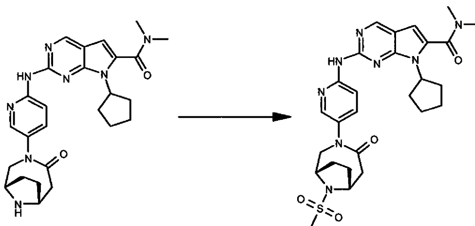
7-cyclopentyl-N,N-dimethyl-2-(5-((1S,6R)-9-(methylsulfonyl)-4-oxo-3,9-diazabicyclo[4.2.1]nonan-3-yl)pyridin-2-ylamino)-7H-pyrrolo[2,3-d]pyrimidine-6-carboxamide
