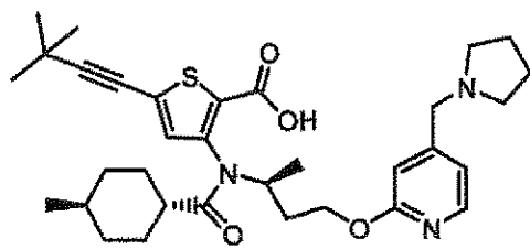
Compound 62
