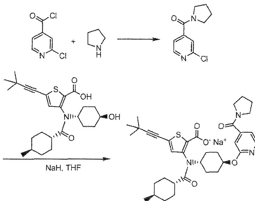
Compound 166
