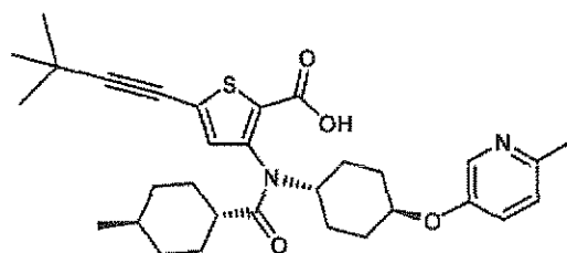
Compound 7
