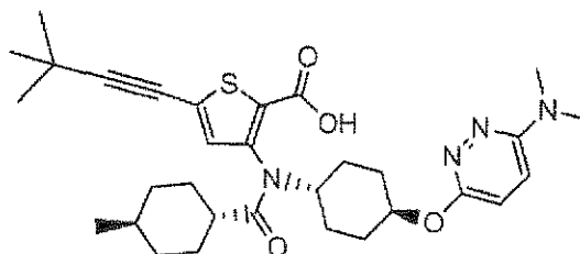
Compound 160
