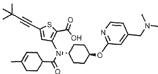
Compound 337
