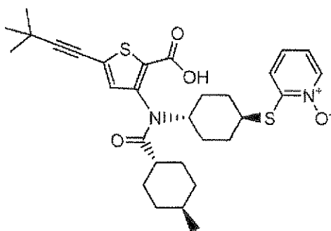
Compound 88
