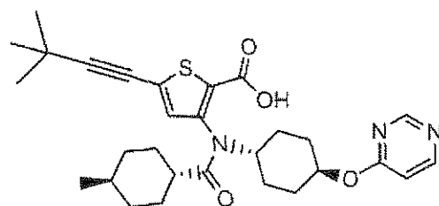
Compound 163
