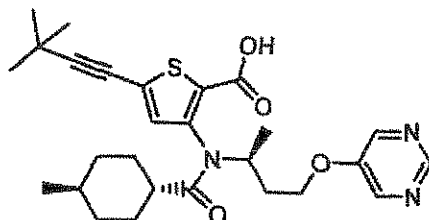
Compound 143
