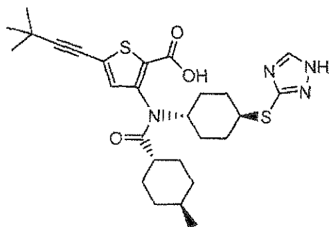
Compound 97
