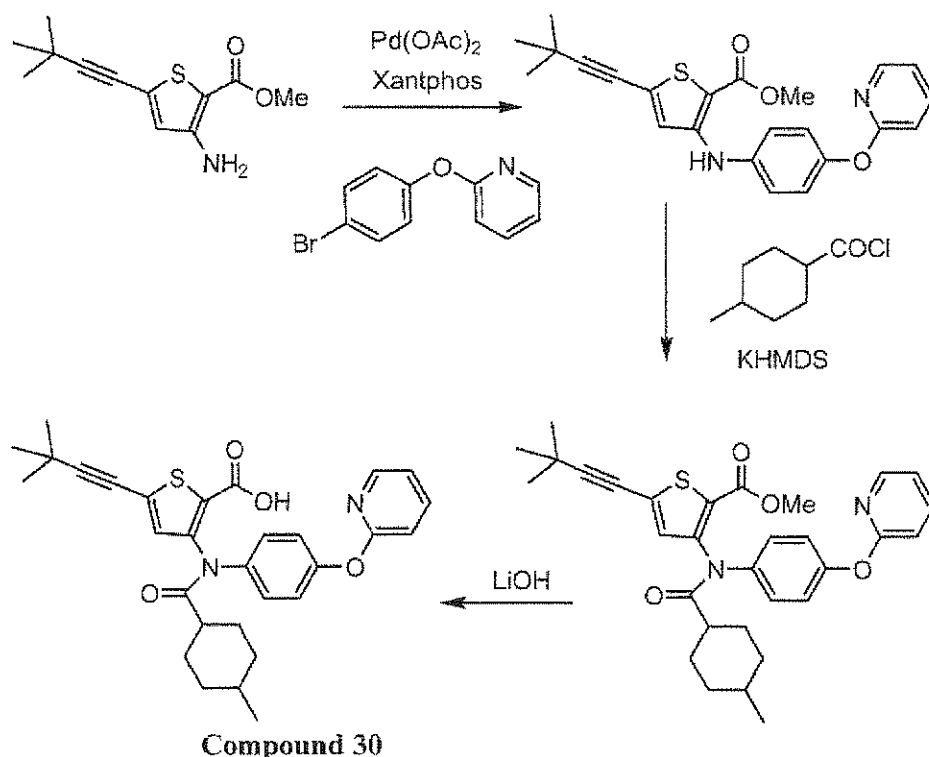
Scheme 5
