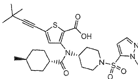
Compound 203
