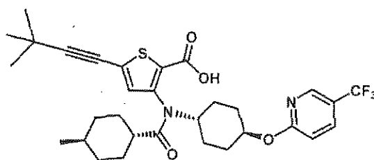
Compound 10
