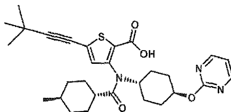
Compound 4
