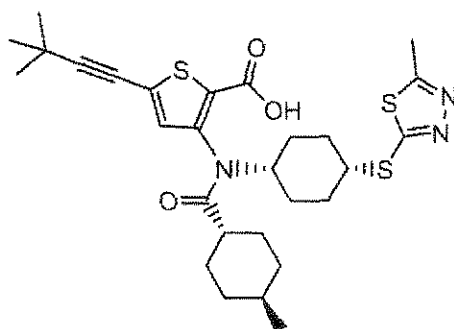
Compound 103
