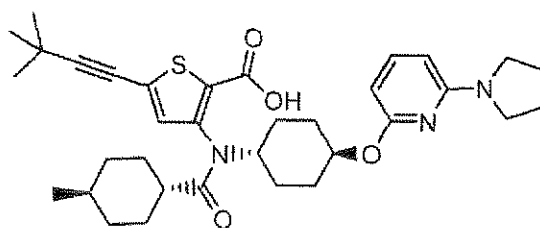
Compound 152
