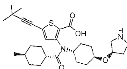
Compound 231
