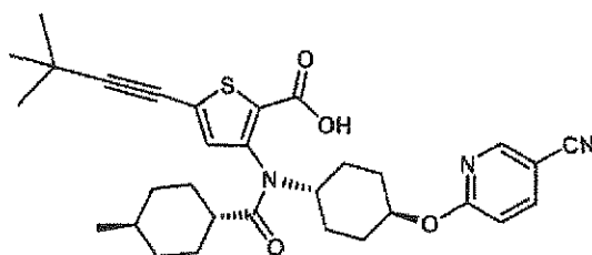
Compound 9
