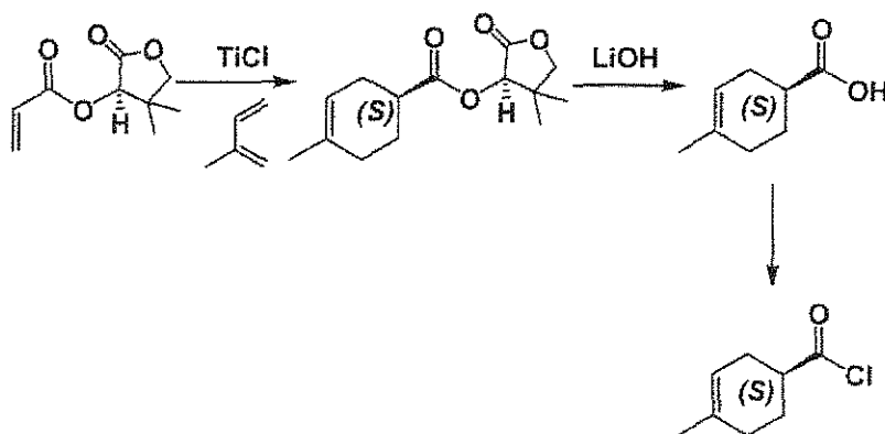
Scheme 15
