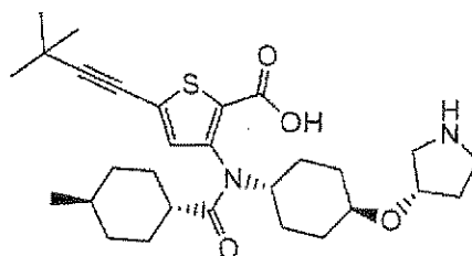
Compound 226
