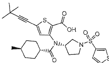
Compound 211
