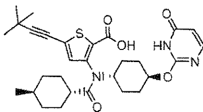
Compound 326
