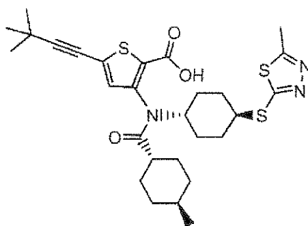
Compound 102
