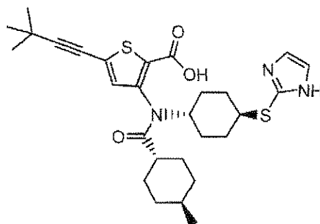
Compound 94
