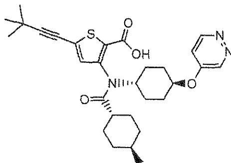
Compound 185
