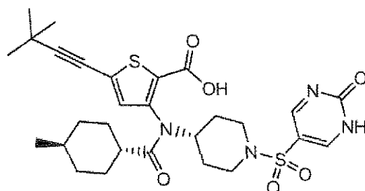
Compound 208
