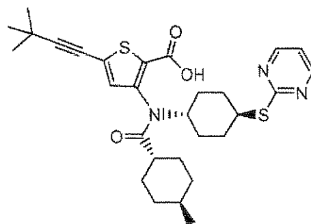
Compound 100
