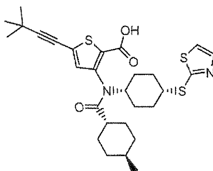
Compound 107
