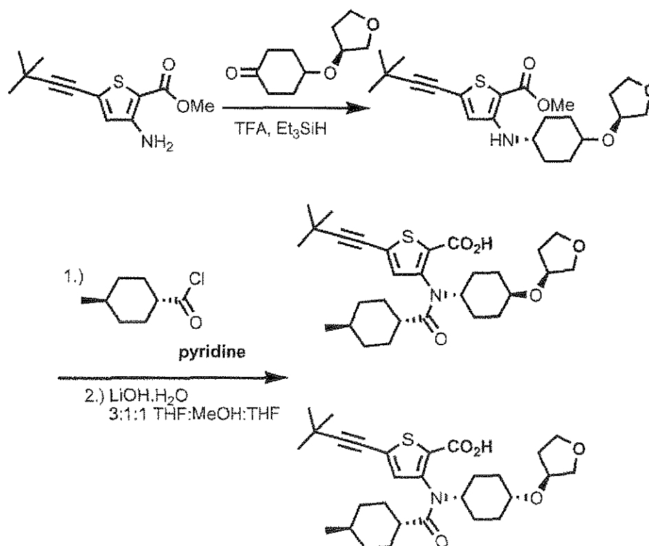
Scheme 17
