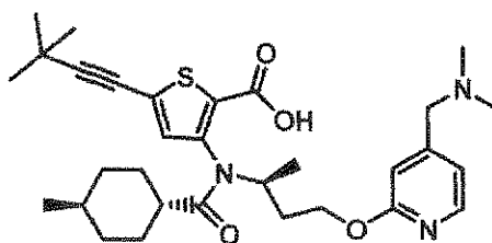
Compound 61
