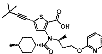
Compound 60
