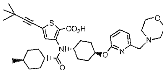
Compound 188
