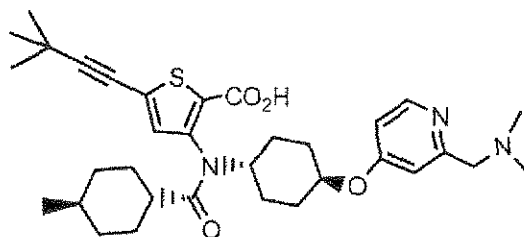
Compound 200
