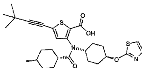
Compound 15
