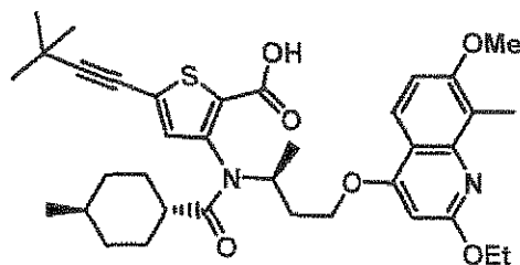
Compound 144
