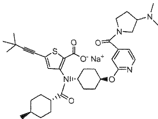
Compound 169
