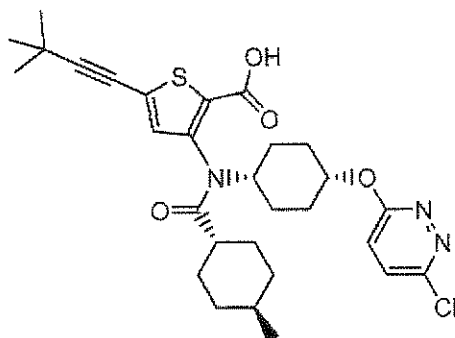
Compound 177
