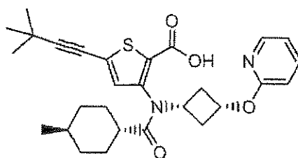
Compound 146
