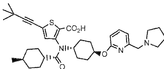
Compound 187
