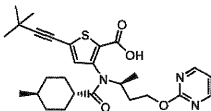
Compound 59
