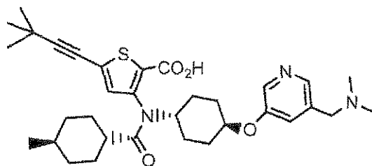
Compound 192
