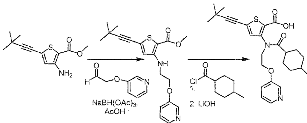
Compound 138
