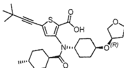
Compound 322
