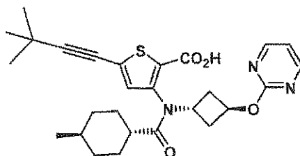
Compound 23
