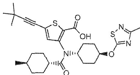
Compound 154
