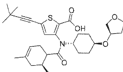
Compound 308
