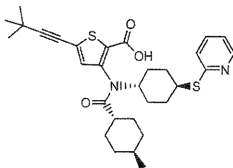
Compound 99
