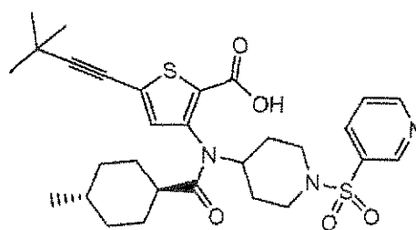
Compound 210
