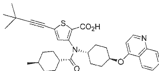
Compound 25
