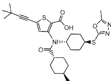
Compound 98
