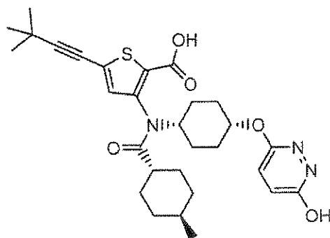
Compound 178
