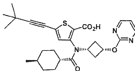
Compound 22
