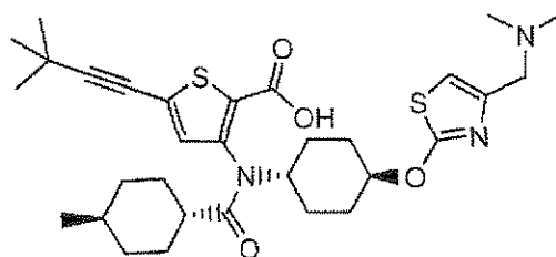
Compound 156
