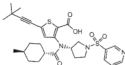
Compound 216
