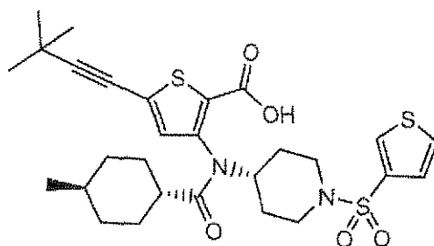
Compound 205
