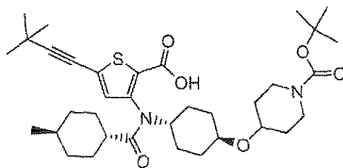
Compound 222
