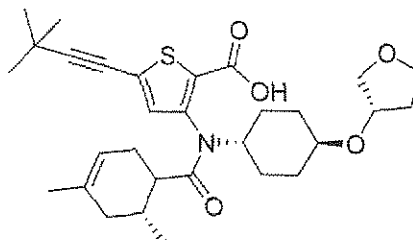
Compound 303
