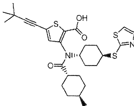
Compound 106
