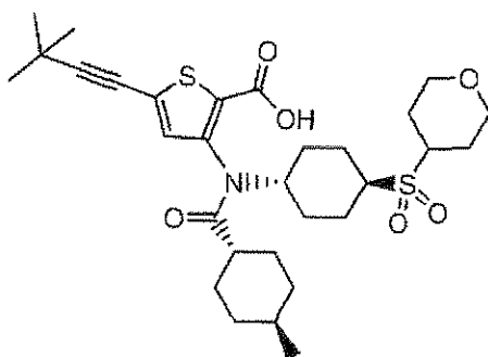
Compound 109
