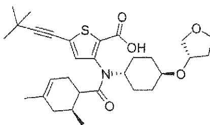
Compound 302
