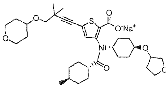
Compound 355
