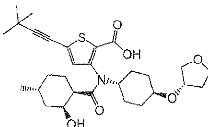
Compound 309
