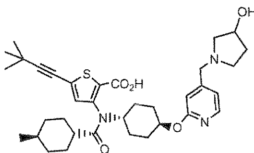
Compound 190
