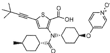
Compound 157
