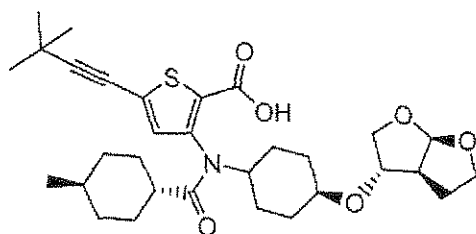
Compound 221
