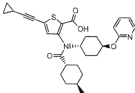
Compound 229
