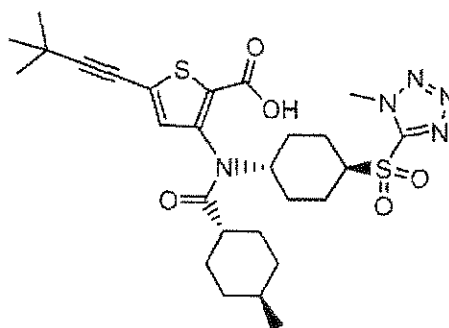
Compound 110
