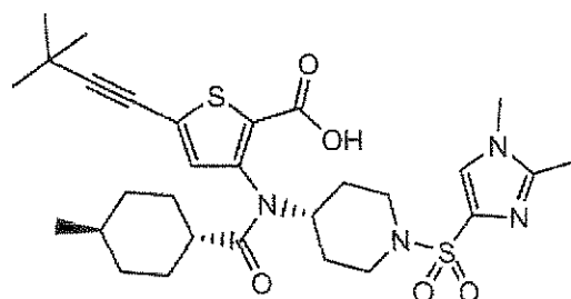
Compound 206
