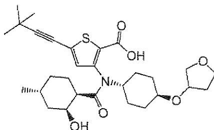
Compound 227
