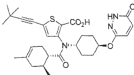
Compound 356
