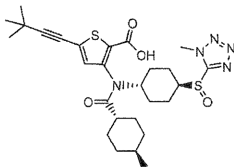
Compound 111
