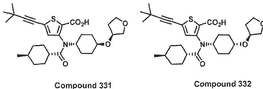
Scheme 17
