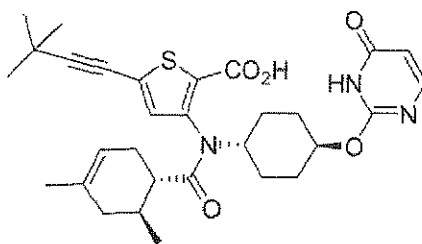
Compound 357
