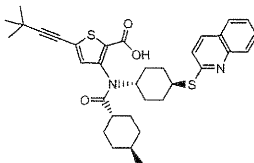
Compound 91
