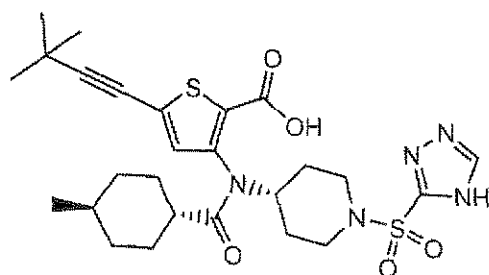
Compound 202
