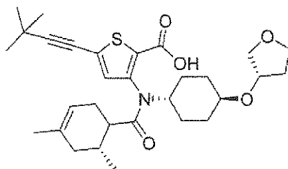
Compound 304
