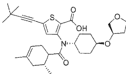
Compound 306
