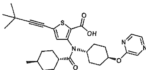
Compound 2
