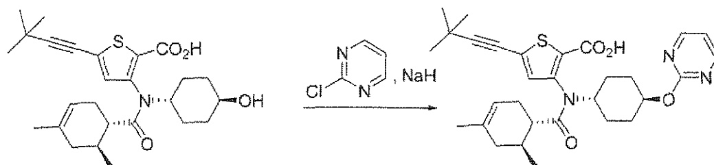
Compound 349
