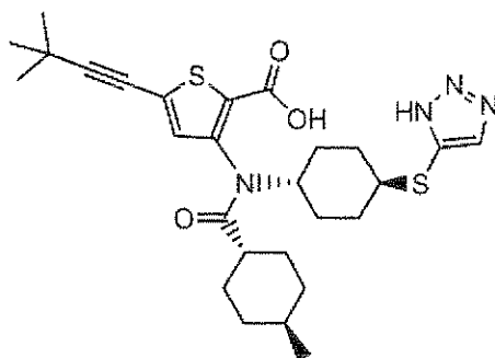
Compound 96
