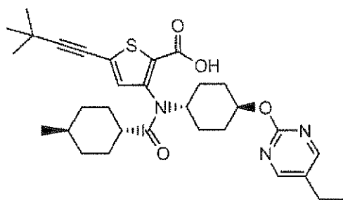
Compound 148
