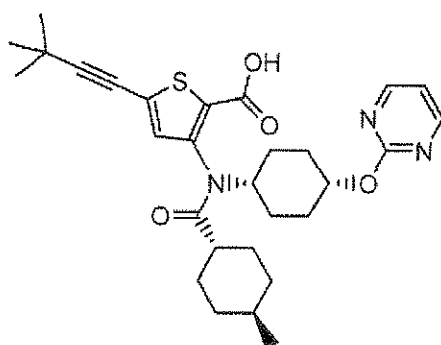
Compound 181
