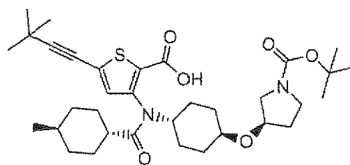
Compound 230
