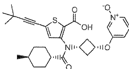
Compound 145
