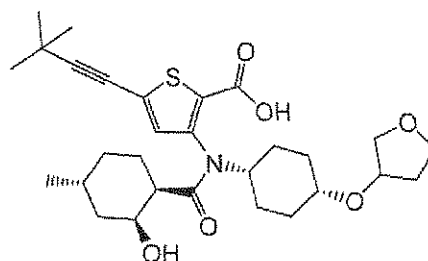
Compound 228
