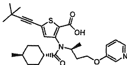
Compound 58
