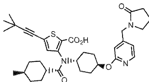
Compound 189
