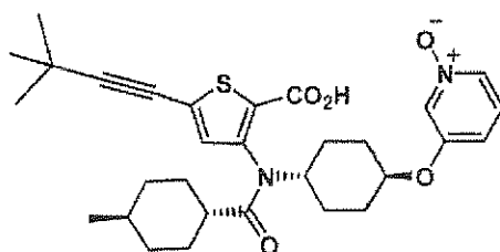
Compound 24
