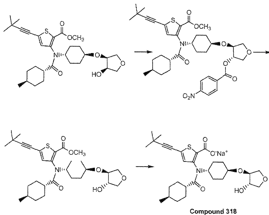
Scheme 9
