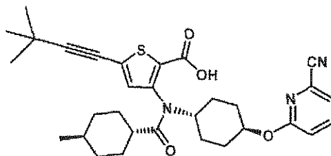
Compound 13
