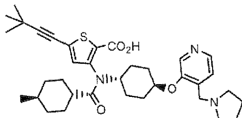
Compound 196
