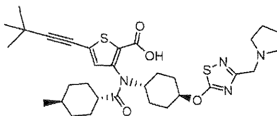
Compound 161
