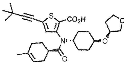
Compound 336
