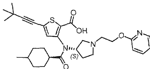
Compound 321
