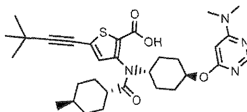
Compound 158
