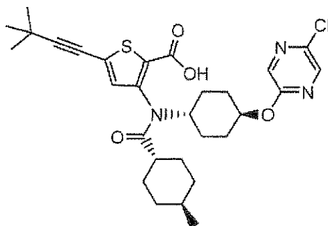
Compound 184
