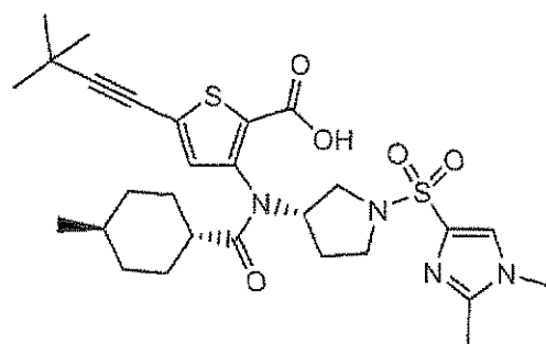
Compound 212
