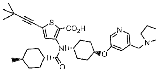
Compound 193
