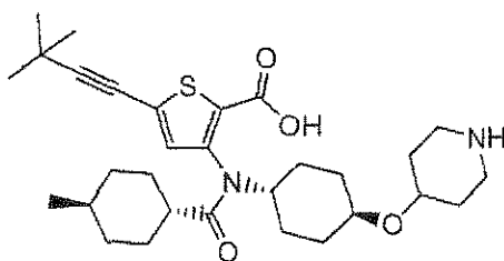
Compound 223
