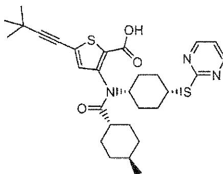
Compound 108
