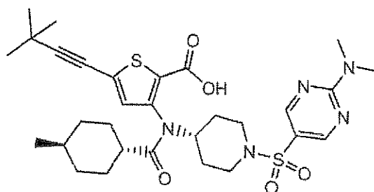
Compound 204
