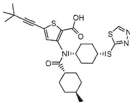
Compound 105
