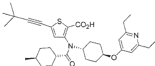
Compound 26
