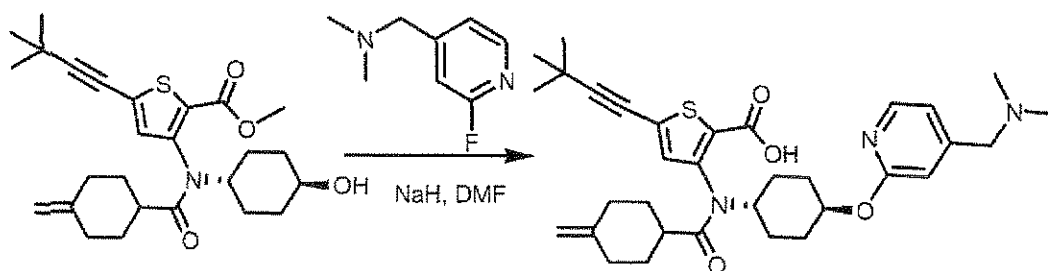
Compound 325
