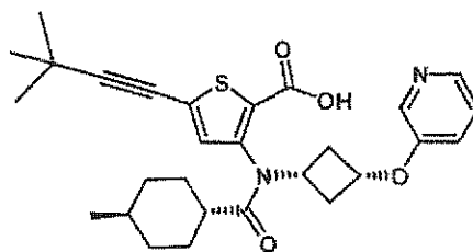
Compound 20
