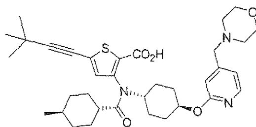
Compound 28
