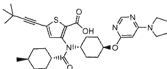
Compound 150
