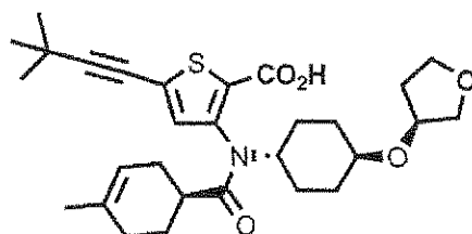
Compound 333
