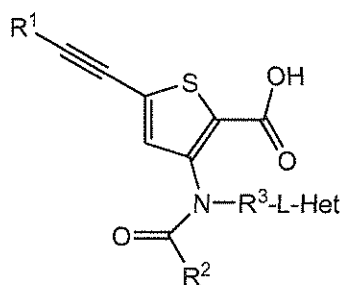
Formula (I),
