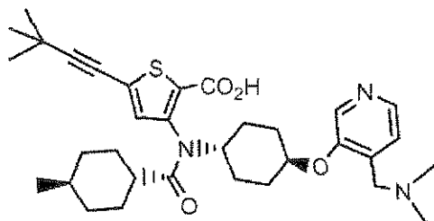
Compound 198
