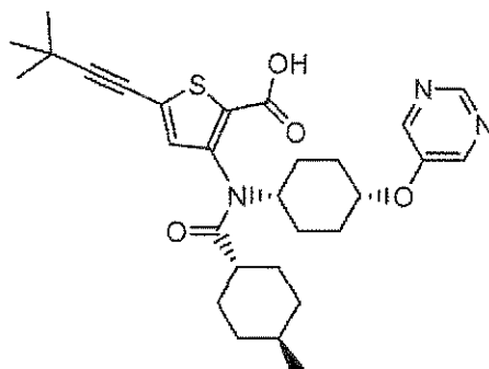
Compound 179
