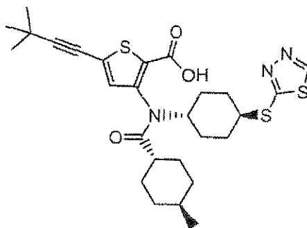
Compound 86
