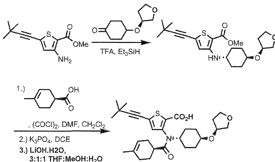
Scheme 18
