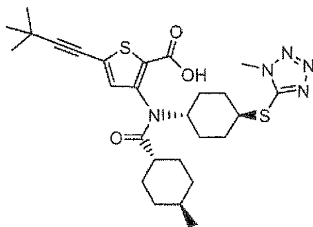
Compound 101
