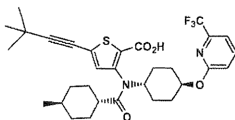
Compound 17
