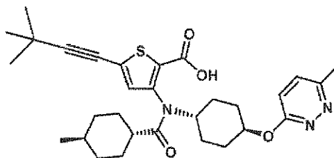
Compound 3
