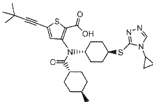
Compound 90
