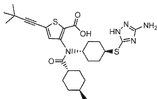
Compound 95
