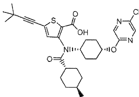
Compound 182
