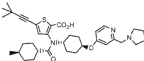
Compound 199
