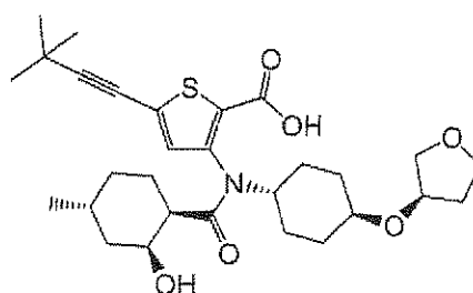
Compound 310
