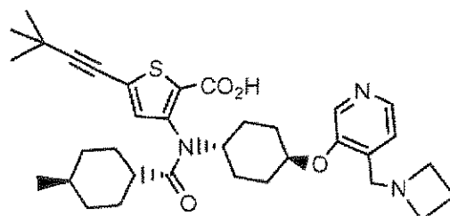
Compound 197
