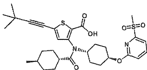
Compound 6
