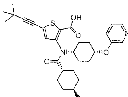
Compound 180
