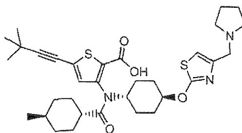
Compound 155
