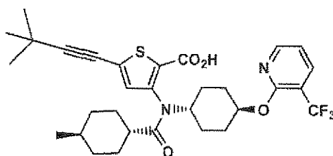
Compound 16
