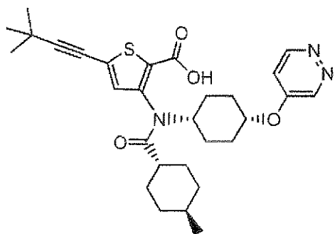
Compound 183
