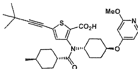
Compound 19
