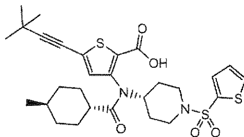
Compound 207
