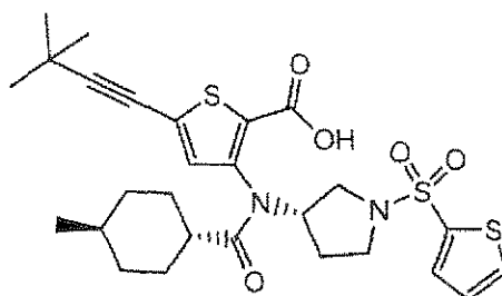
Compound 213
