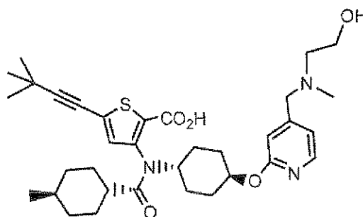
Compound 191
