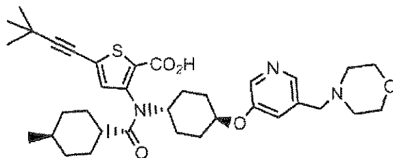
Compound 194
