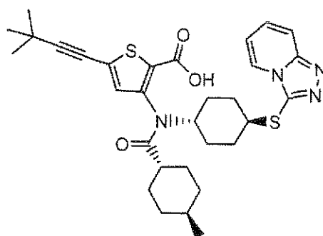
Compound 92
