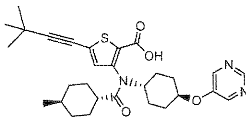
Compound 162
