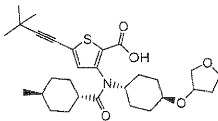
Compound 224
