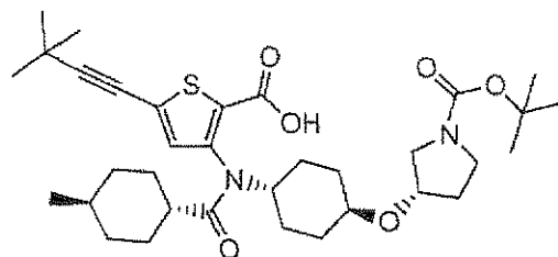
Compound 225
