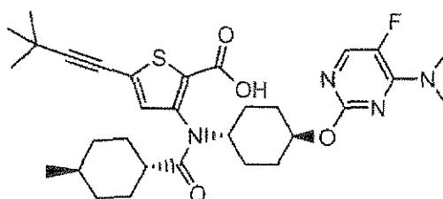
Compound 151
