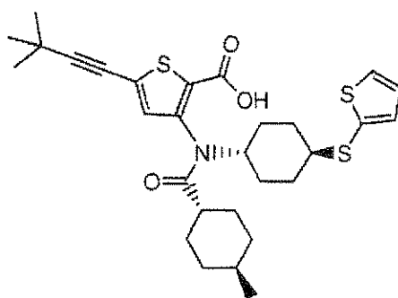
Compound 93
