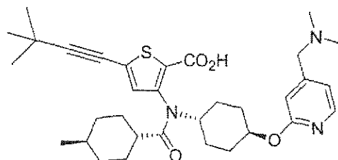
Compound 29
