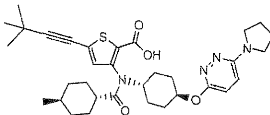
Compound 159
