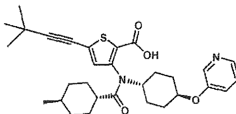
Compound 5
