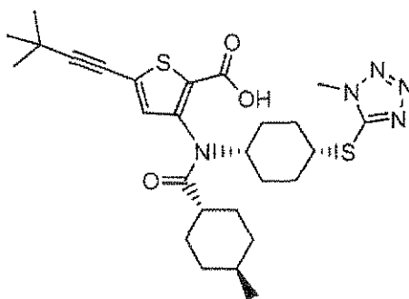
Compound 104
