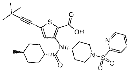
Compound 209
