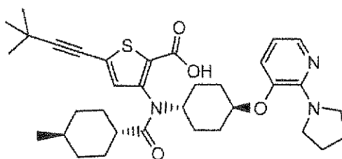
Compound 149
