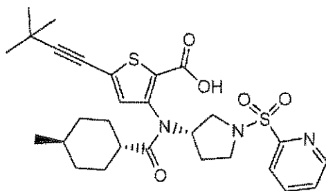
Compound 215
