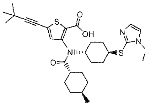
Compound 89
