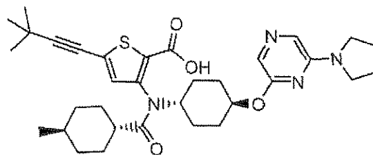
Compound 153
