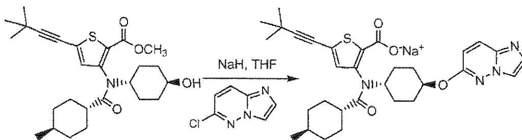
Compound 176
