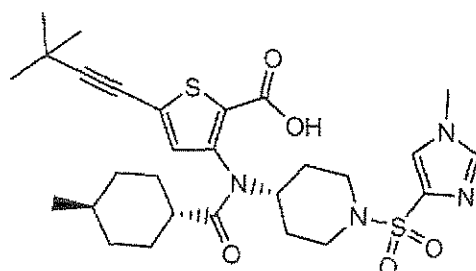
Compound 201
