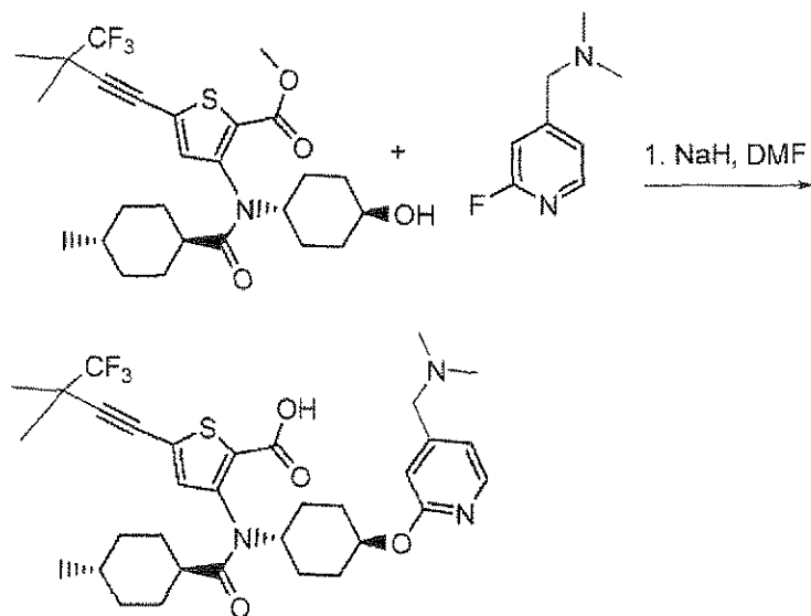
Compound 341
