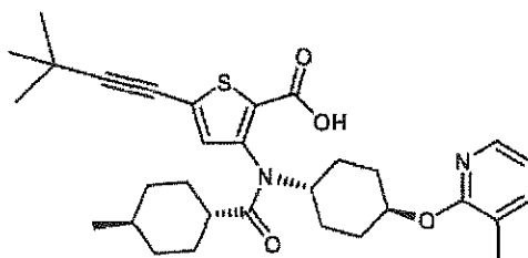
Compound 12
