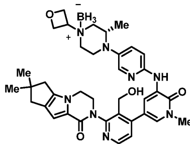
Borane adduct 2
