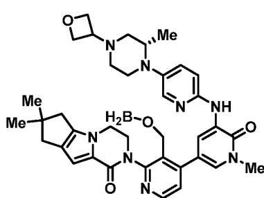
Borane adduct 1
