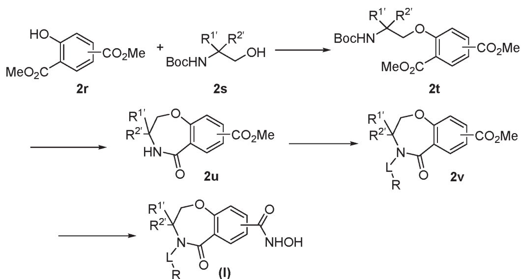
Scheme 4. General synthesis of amides described in the disclosure.
