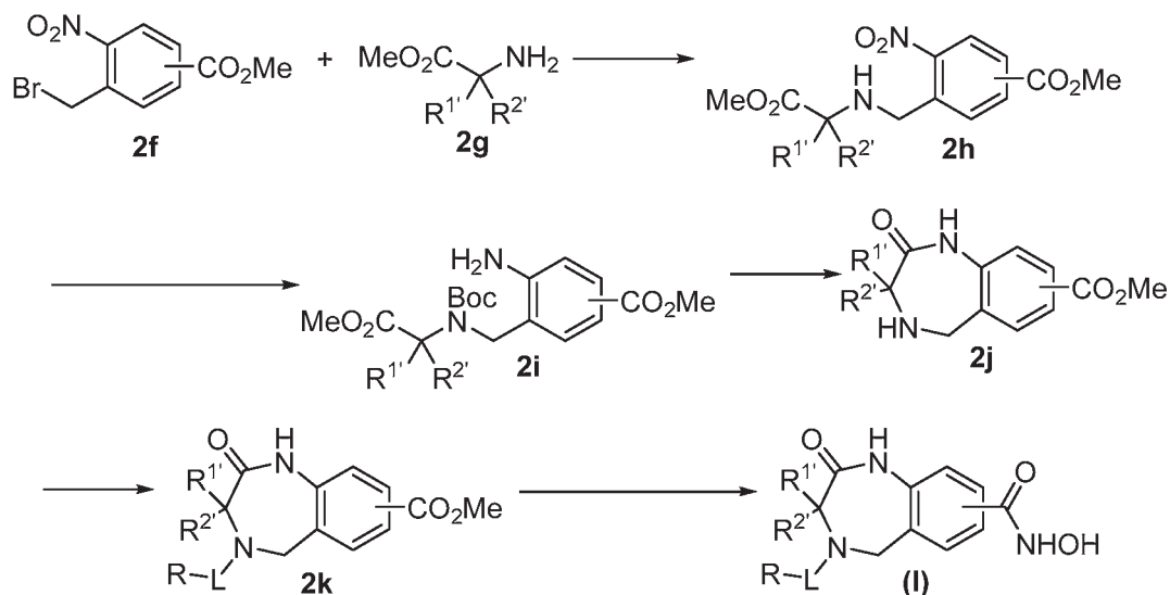
Scheme 2. General synthesis of amides described in the disclosure.
