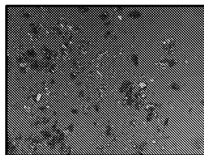
L-lactate salt, Lot 6044-160-6
