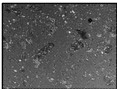
HCl salt, Lot 6044-161-1
