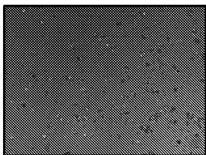
L-tartrate salt, Lot 6044-160-4
