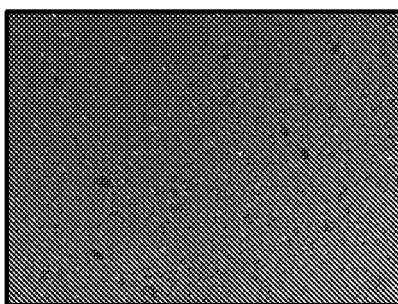
L-malate salt, Lot 6044-161-2
