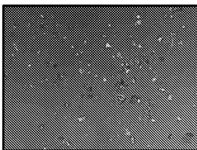
Free base, Lot S00L06
