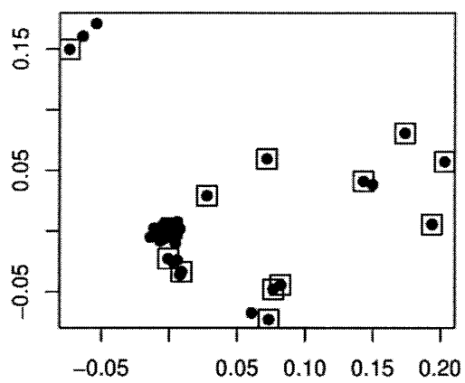
Centroids of OTUs picked by Qiime
