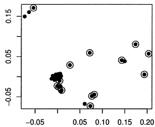
Centroids of OTUs picked by Mothur
