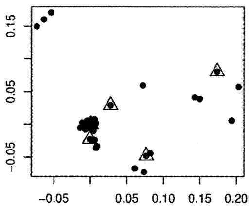
Centroids of OTUs picked by Usearch
