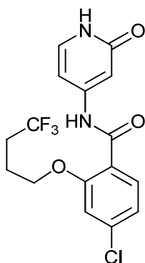
4-chloro-N-(2-oxo-1,2-dihydropyridin-4-yl)-2-(4,4,4-trifluorobutoxy)benzamide;
