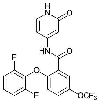
2-(2,6-difluorophenoxy)-N-(2-oxo-1,2-dihydropyridin-4-yl)-5-(trifluoromethoxy)benzamide;
