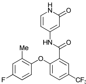
2-(4-fluoro-2-methylphenoxy)-N-(2-oxo-1,2-dihydropyridin-4-yl)-5-(trifluoromethyl)benzamide;
