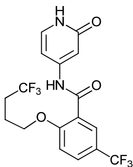
N-(2-oxo-1,2-dihydropyridin-4-yl)-2-(4,4,4-trifluorobutoxy)-5-(trifluoromethyl)benzamide;
