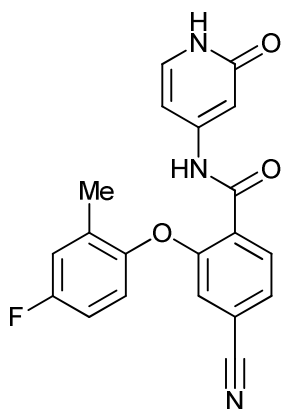
4-cyano-2-(4-fluoro-2-methylphenoxy)-N-(2-oxo-1,2-dihydropyridin-4-yl)benzamide;
