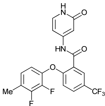
2-(2,3-difluoro-4-methylphenoxy)-N-(2-oxo-1,2-dihydropyridin-4-yl)-5-(trifluoromethyl)benzamide;
