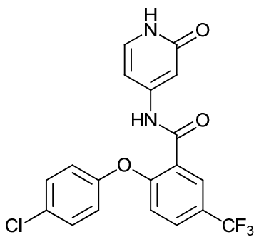
2-(4-chlorophenoxy)-N-(2-oxo-1,2-dihydropyridin-4-yl)-5-(trifluoromethyl)benzamide;
