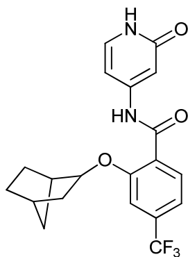
2-(bicyclo[2.2.1]heptan-2-yloxy)-N-(2-oxo-1,2-dihydropyridin-4-yl)-4-(trifluoromethyl)benzamide;
