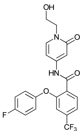
2-(4-fluorophenoxy)-N-(1-(2-hydroxyethyl)-2-oxo-1,2-dihydropyridin-4-yl)-4-(trifluoromethyl)benzamide;
