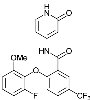
2-(2-fluoro-6-methoxyphenoxy)-N-(2-oxo-1,2-dihydropyridin-4-yl)-5-(trifluoromethyl)benzamide;
