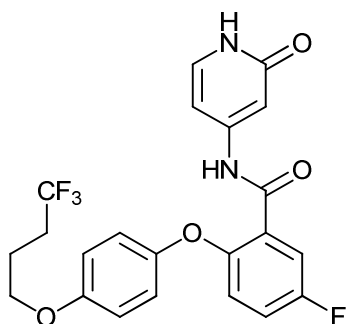
5-fluoro-N-(2-oxo-1,2-dihydropyridin-4-yl)-2-(4-(4,4,4-trifluorobutoxy)phenoxy)benzamide;
