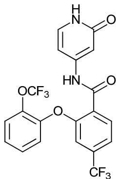
N-(2-oxo-1,2-dihydropyridin-4-yl)-2-(2-(trifluoromethoxy)phenoxy)-4-(trifluoromethyl)benzamide;
