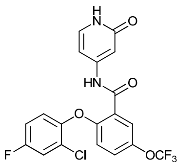
2-(2-chloro-4-fluorophenoxy)-N-(2-oxo-1,2-dihydropyridin-4-yl)-5-(trifluoromethoxy)benzamide;
