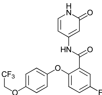
5-fluoro-N-(2-oxo-1,2-dihydropyridin-4-yl)-2-(4-(2,2,2-trifluoroethoxy)phenoxy)benzamide;
