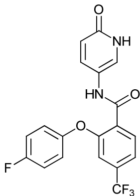
2-(4-fluorophenoxy)-N-(6-oxo-1,6-dihydropyridin-3-yl)-4-(trifluoromethyl)benzamide;
