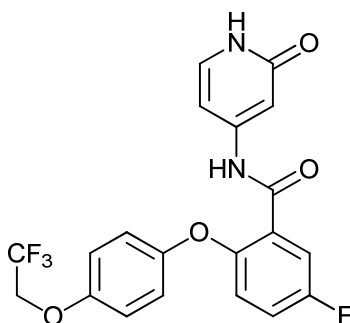
5-fluoro-N-(2-oxo-1,2-dihydropyridin-4-yl)-2-(4-(2,2,2-trifluoroethoxy)phenoxy)benzamide;
