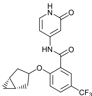
2-((1R,5S)-bicyclo[3.1.0]hexan-3-yloxy)-N-(2-oxo-1,2-dihydropyridin-4-yl)-5-(trifluoromethyl)benzamide;
