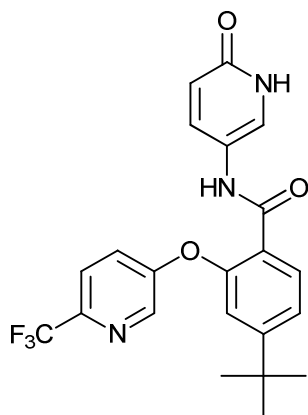
4-(tert-butyl)-N-(6-oxo-1,6-dihydropyridin-3-yl)-2-(((6-(trifluoromethyl)pyridin-3-yl)oxy)benzamide;
