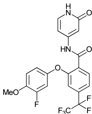
2-(3-fluoro-4-methoxyphenoxy)-N-(2-oxo-1,2-dihydropyridin-4-yl)-4-(perfluoroethyl)benzamide;
