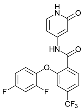
2-(2,4-difluorophenoxy)-N-(2-oxo-1,2-dihydropyridin-4-yl)-4-(trifluoromethyl)benzamide;
