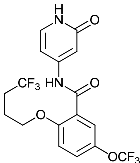
N-(2-oxo-1,2-dihydropyridin-4-yl)-2-(4,4,4-trifluorobutoxy)-5-(trifluoromethoxy)benzamide;
