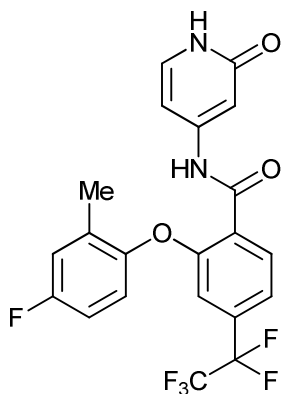
2-(4-fluoro-2-methylphenoxy)-N-(2-oxo-1,2-dihydropyridin-4-yl)-4-(perfluoroethyl)benzamide;
