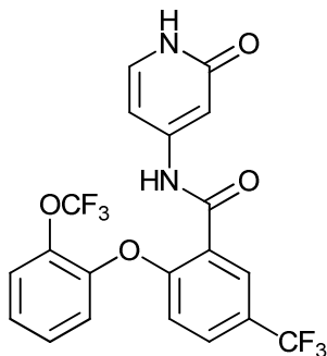
N-(2-oxo-1,2-dihydropyridin-4-yl)-2-(2-(trifluoromethoxy)phenoxy)-5-(trifluoromethyl)benzamide;
