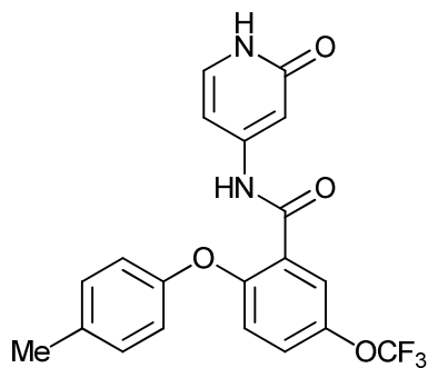
N-(2-oxo-1,2-dihydropyridin-4-yl)-2-(p-tolxyloxy)-5-(trifluoromethoxy)benzamide;
