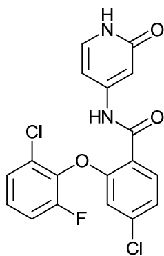
4-chloro-2-(2-chloro-6-fluorophenoxy)-N-(2-oxo-1,2-dihydropyridin-4-yl)benzamide;
