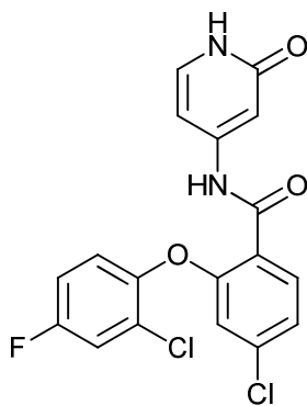
4-chloro-2-(2-chloro-4-fluorophenoxy)-N-(2-oxo-1,2-dihydropyridin-4-yl)benzamide;
