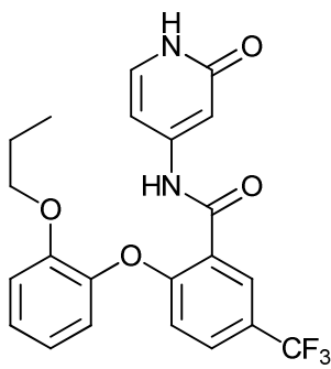
N-(2-oxo-1,2-dihydropyridin-4-yl)-2-(2-propoxyphenoxy)-5-(trifluoromethyl)benzamide;
