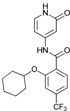
2-(cyclohexyloxy)-N-(2-oxo-1,2-dihydropyridin-4-yl)-4-(trifluoromethyl)benzamide;
