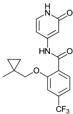
2-((1-methylcyclopropyl)methoxy)-N-(2-oxo-1,2-dihydropyridin-4-yl)-4-(trifluoromethyl)benzamide;
