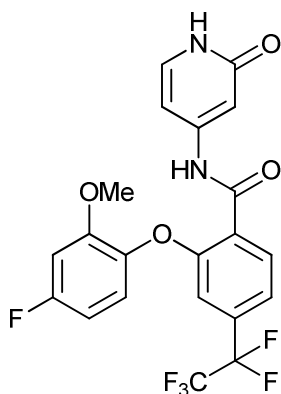
2-(4-fluoro-2-methoxyphenoxy)-N-(2-oxo-1,2-dihydropyridin-4-yl)-4-(perfluoroethyl)benzamide;
