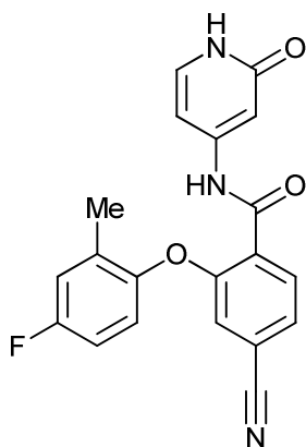
4-cyano-2-(4-fluoro-2-methylphenoxy)-N-(2-oxo-1,2-dihydropyridin-4-yl)benzamide;
