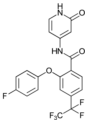
2-(4-fluorophenoxy)-N-(2-oxo-1,2-dihydropyridin-4-yl)-4-(perfluoroethyl)benzamide;
