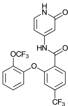
N-(2-oxo-1,2-dihydropyridin-4-yl)-2-(2-(trifluoromethoxy)phenoxy)-4-(trifluoromethyl)benzamide;
