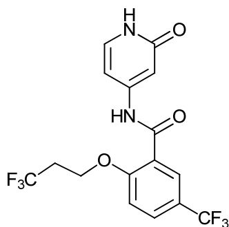
N-(2-oxo-1,2-dihydropyridin-4-yl)-5-(trifluoromethyl)-2-(3,3,3-trifluoropropoxy)benzamide;
