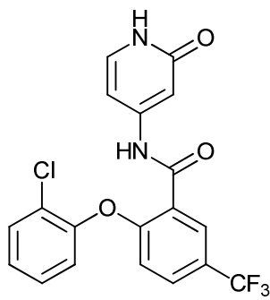
2-(2-chlorophenoxy)-N-(2-oxo-1,2-dihydropyridin-4-yl)-5-(trifluoromethyl)benzamide;
