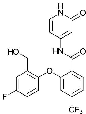
2-(4-fluoro-2-(hydroxymethyl)phenoxy)-N-(2-oxo-1,2-dihydropyridin-4-yl)-4-(trifluoromethyl)benzamide;
