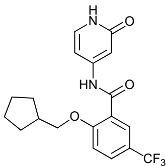
2-(cyclopentylmethoxy)-N-(2-oxo-1,2-dihydropyridin-4-yl)-5-(trifluoromethyl)benzamide;
