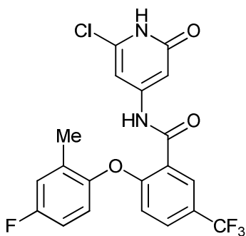
N-(6-chloro-2-oxo-1,2-dihydropyridin-4-yl)-2-(4-fluoro-2-methylphenoxy)-5-(trifluoromethyl)benzamide;
