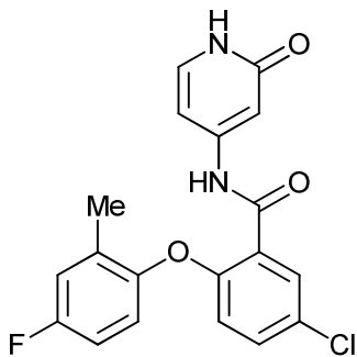
5-chloro-2-(4-fluoro-2-methylphenoxy)-N-(2-oxo-1,2-dihydropyridin-4-yl)benzamide;
