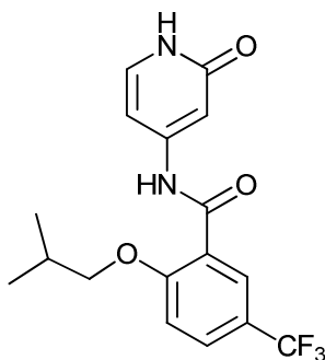
2-isobutoxy-N-(2-oxo-1,2-dihydropyridin-4-yl)-5-(trifluoromethyl)benzamide;
