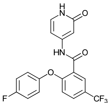
2-(4-fluorophenoxy)-N-(2-oxo-1,2-dihydropyridin-4-yl)-5-(trifluoromethyl)benzamide;
