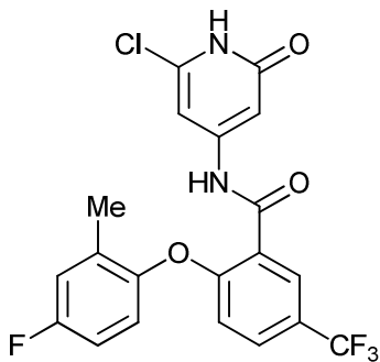
N-(6-chloro-2-oxo-1,2-dihydropyridin-4-yl)-2-(4-fluoro-2-methylphenoxy)-5-(trifluoromethyl)benzamide;
