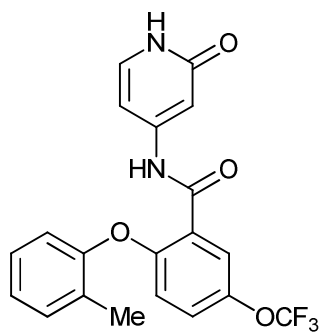
N-(2-oxo-1,2-dihydropyridin-4-yl)-2-(o-tolyloxy)-5-(trifluoromethoxy)benzamide;
