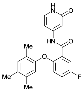
5-fluoro-N-(2-oxo-1,2-dihydropyridin-4-yl)-2-(2,4,5-trimethylphenoxy)benzamide;
