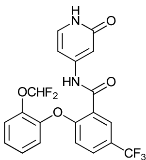
2-(2-(difluoromethoxy)phenoxy)-N-(2-oxo-1,2-dihydropyridin-4-yl)-5-(trifluoromethyl)benzamide;
