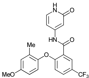
2-(4-methoxy-2-methylphenoxy)-N-(2-oxo-1,2-dihydropyridin-4-yl)-5-(trifluoromethyl)benzamide;
