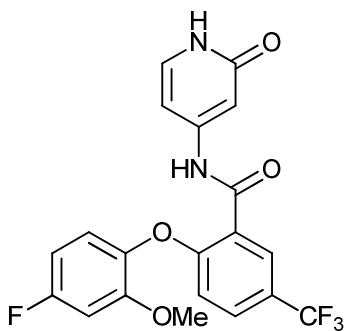
2-(4-fluoro-2-methoxyphenoxy)-N-(2-oxo-1,2-dihydropyridin-4-yl)-5-(trifluoromethyl)benzamide;
