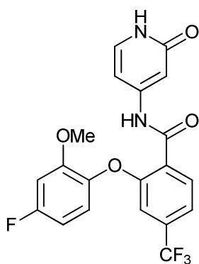
2-(4-fluoro-2-methoxyphenoxy)-N-(2-oxo-1,2-dihydropyridin-4-yl)-4-(trifluoromethyl)benzamide;
