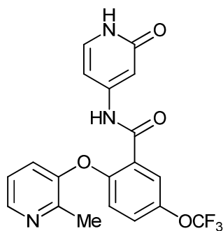
2-((2-methylpyridin-3-yl)oxy)-N-(2-oxo-1,2-dihydropyridin-4-yl)-5-(trifluoromethoxy)benzamide;
