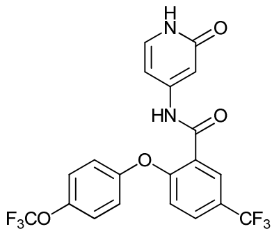
N-(2-oxo-1,2-dihydropyridin-4-yl)-2-(4-(trifluoromethoxy)phenoxy)-5-(trifluoromethyl)benzamide;
