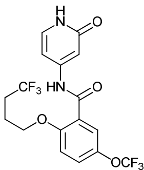
N-(2-oxo-1,2-dihydropyridin-4-yl)-2-(4,4,4-trifluorobutoxy)-5-(trifluoromethoxy)benzamide;
