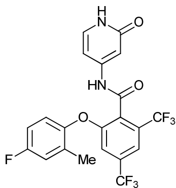
2-(4-fluoro-2-methylphenoxy)-N-(2-oxo-1,2-dihydropyridin-4-yl)-4,6-bis(trifluoromethyl)benzamide;
