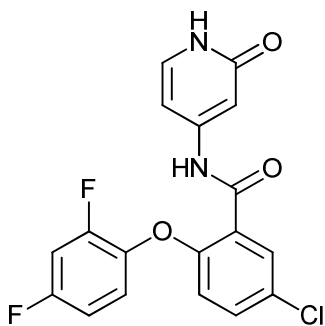
5-chloro-2-(2,4-difluorophenoxy)-N-(2-oxo-1,2-dihydropyridin-4-yl)benzamide;
