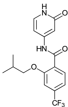
2-isobutoxy-N-(2-oxo-1,2-dihydropyridin-4-yl)-4-(trifluoromethyl)benzamide;
