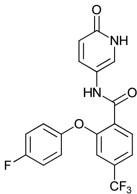
2-(4-fluorophenoxy)-N-(6-oxo-1,6-dihydropyridin-3-yl)-4-(trifluoromethyl)benzamide;
