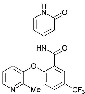
2-((2-methylpyridin-3-yl)oxy)-N-(2-oxo-1,2-dihydropyridin-4-yl)-5-(trifluoromethyl)benzamide;
