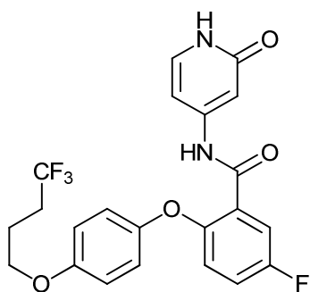
5-fluoro-N-(2-oxo-1,2-dihydropyridin-4-yl)-2-(4-(4,4,4-trifluorobutoxy)phenoxy)benzamide.
