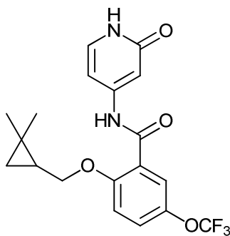
2-((2,2-dimethylcyclopropyl)methoxy)-N-(2-oxo-1,2-dihydropyridin-4-yl)-5-(trifluoromethoxy)benzamide;
