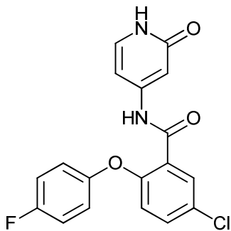
5-chloro-2-(4-fluorophenoxy)-N-(2-oxo-1,2-dihydropyridin-4-yl)benzamide;
