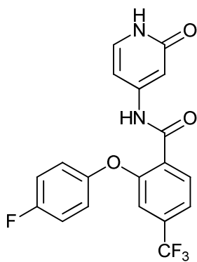
2-(4-fluorophenoxy)-N-(2-oxo-1,2-dihydropyridin-4-yl)-4-(trifluoromethyl)benzamide;
