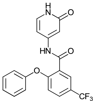
N-(2-oxo-1,2-dihydropyridin-4-yl)-2-phenoxy-5-(trifluoromethyl)benzamide;
