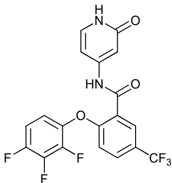
N-(2-oxo-1,2-dihydropyridin-4-yl)-5-(trifluoromethyl)-2-(2,3,4-trifluorophenoxy)benzamide;
