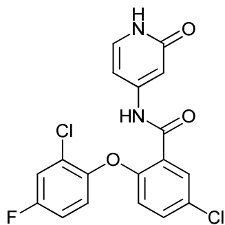
5-chloro-2-(2-chloro-4-fluorophenoxy)-N-(2-oxo-1,2-dihydropyridin-4-yl)benzamide;
