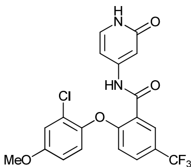
2-(2-chloro-4-methoxyphenoxy)-N-(2-oxo-1,2-dihydropyridin-4-yl)-5-(trifluoromethyl)benzamide;
