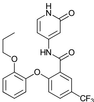
N-(2-oxo-1,2-dihydropyridin-4-yl)-2-(2-propoxyphenoxy)-5-(trifluoromethyl)benzamide;
