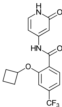
2-cyclobutoxy-N-(2-oxo-1,2-dihydropyridin-4-yl)-4-(trifluoromethyl)benzamide;
