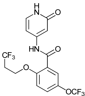
N-(2-oxo-1,2-dihydropyridin-4-yl)-5-(trifluoromethoxy)-2-(3,3,3-trifluoropropoxy)benzamide;
