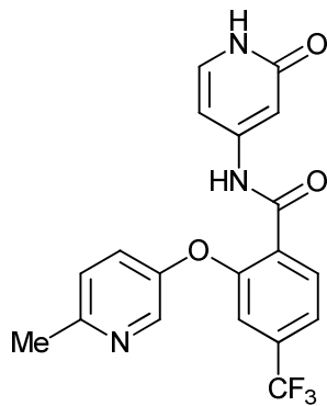
2-((6-methylpyridin-3-yl)oxy)-N-(2-oxo-1,2-dihydropyridin-4-yl)-4-(trifluoromethyl)benzamide;
