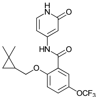
2-((2,2-dimethylcyclopropyl)methoxy)-N-(2-oxo-1,2-dihydropyridin-4-yl)-5-(trifluoromethoxy)benzamide;
