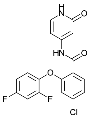
4-chloro-2-(2,4-difluorophenoxy)-N-(2-oxo-1,2-dihydropyridin-4-yl)benzamide;
