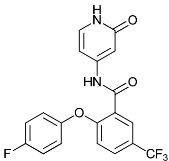
2-(4-fluorophenoxy)-N-(2-oxo-1,2-dihydropyridin-4-yl)-5-(trifluoromethyl)benzamide;
