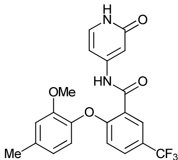
2-(2-methoxy-4-methylphenoxy)-N-(2-oxo-1,2-dihydropyridin-4-yl)-5-(trifluoromethyl)benzamide;
