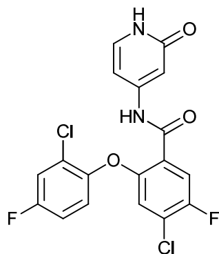
4-chloro-2-(2-chloro-4-fluorophenoxy)-5-fluoro-N-(2-oxo-1,2-dihydropyridin-4-yl)benzamide;
