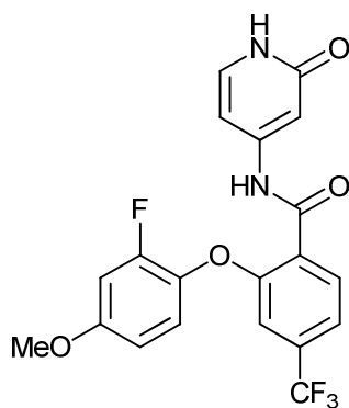
2-(2-fluoro-4-methoxyphenoxy)-N-(2-oxo-1,2-dihydropyridin-4-yl)-4-(trifluoromethyl)benzamide;
