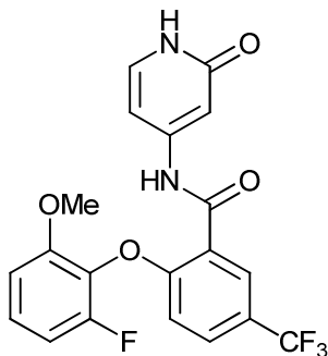
2-(2-fluoro-6-methoxyphenoxy)-N-(2-oxo-1,2-dihydropyridin-4-yl)-5-(trifluoromethyl)benzamide;
