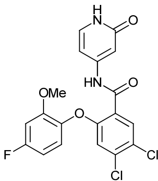
4,5-dichloro-2-(4-fluoro-2-methoxyphenoxy)-N-(2-oxo-1,2-dihydropyridin-4-yl)benzamide;
