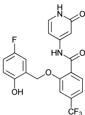
2-((5-fluoro-2-hydroxybenzyl)oxy)-N-(2-oxo-1,2-dihydropyridin-4-yl)-4-(trifluoromethyl)benzamide; and
