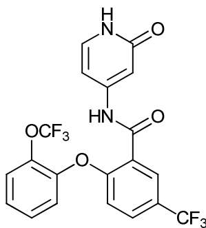
N-(2-oxo-1,2-dihydropyridin-4-yl)-2-(2-(trifluoromethoxy)phenoxy)-5-(trifluoromethyl)benzamide;
