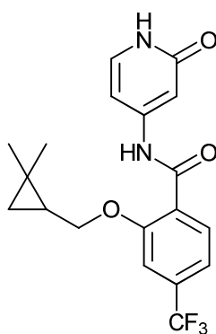
2-((2,2-dimethylcyclopropyl)methoxy)-N-(2-oxo-1,2-dihydropyridin-4-yl)-4-(trifluoromethyl)benzamide;
