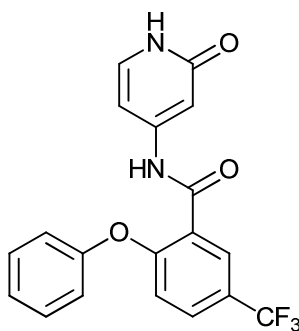
N-(2-oxo-1,2-dihydropyridin-4-yl)-2-phenoxy-5-(trifluoromethyl)benzamide;
