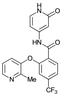
2-((2-methylpyridin-3-yl)oxy)-N-(2-oxo-1,2-dihydropyridin-4-yl)-4-(trifluoromethyl)benzamide;
