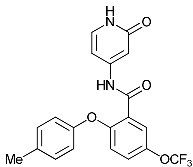
N-(2-oxo-1,2-dihydropyridin-4-yl)-2-(p-tolyloxy)-5-(trifluoromethoxy)benzamide;
