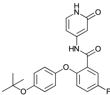
2-(4-(tert-butoxy)phenoxy)-5-fluoro-N-(2-oxo-1,2-dihydropyridin-4-yl)benzamide;
