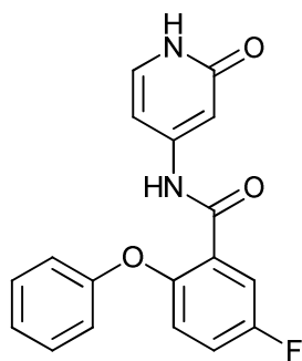
5-fluoro-N-(2-oxo-1,2-dihydropyridin-4-yl)-2-phenoxybenzamide;
