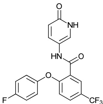
2-(4-fluorophenoxy)-N-(6-oxo-1,6-dihydropyridin-3-yl)-5-(trifluoromethyl)benzamide;
