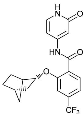
2-((2R)-bicyclo[2.2.1]heptan-2-yloxy)-N-(2-oxo-1,2-dihydropyridin-4-yl)-4-(trifluoromethyl)benzamide;
