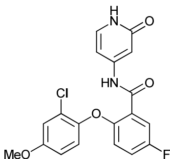
2-(2-chloro-4-methoxyphenoxy)-5-fluoro-N-(2-oxo-1,2-dihydropyridin-4-yl)benzamide;
