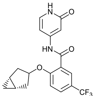
2-(((1R,5S)-bicyclo[3.1.0]hexan-3-yloxy)-N-(2-oxo-1,2-dihydropyridin-4-yl)-5-(trifluoromethyl)benzamide;
