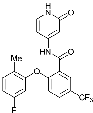
2-(5-fluoro-2-methylphenoxy)-N-(2-oxo-1,2-dihydropyridin-4-yl)-5-(trifluoromethyl)benzamide;
