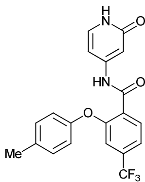
N-(2-oxo-1,2-dihydropyridin-4-yl)-2-(p-tolyloxy)-4-(trifluoromethyl)benzamide;
