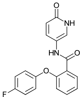
2-(4-fluorophenoxy)-N-(6-oxo-1,6-dihydropyridin-3-yl)benzamide;
