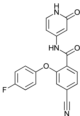
4-cyano-2-(4-fluorophenoxy)-N-(2-oxo-1,2-dihydropyridin-4-yl)benzamide;
