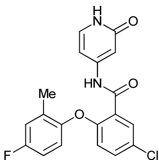
5-chloro-2-(4-fluoro-2-methylphenoxy)-N-(2-oxo-1,2-dihydropyridin-4-yl)benzamide;
