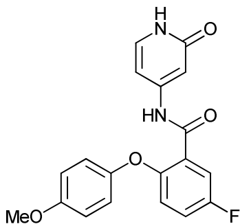
5-fluoro-2-(4-methoxyphenoxy)-N-(2-oxo-1,2-dihydropyridin-4-yl)benzamide;
