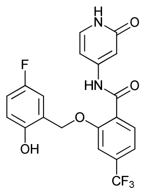
2-((5-fluoro-2-hydroxybenzyl)oxy)-N-(2-oxo-1,2-dihydropyridin-4-yl)-4-(trifluoromethyl)benzamide; and
