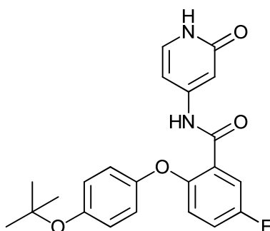
2-(4-(tert-butoxy)phenoxy)-5-fluoro-N-(2-oxo-1,2-dihydropyridin-4-yl)benzamide;
