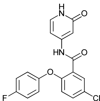
5-chloro-2-(4-fluorophenoxy)-N-(2-oxo-1,2-dihydropyridin-4-yl)benzamide;
