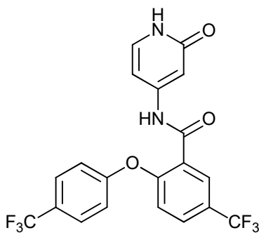
N-(2-oxo-1,2-dihydropyridin-4-yl)-5-(trifluoromethyl)-2-(4-(trifluoromethyl)phenoxy)benzamide;
