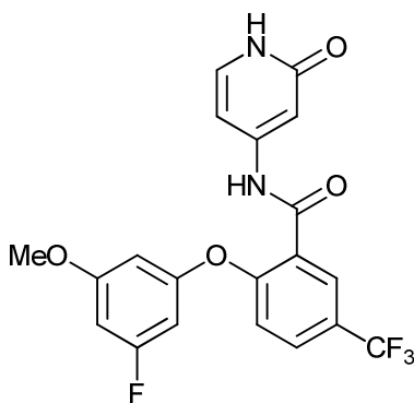
2-(3-fluoro-5-methoxyphenoxy)-N-(2-oxo-1,2-dihydropyridin-4-yl)-5-(trifluoromethyl)benzamide;
