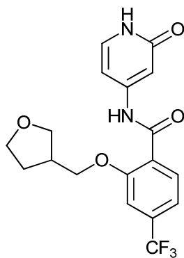
N-(2-oxo-1,2-dihydropyridin-4-yl)-2-((tetrahydrofuran-3-yl)methoxy)-4-(trifluoromethyl)benzamide;
