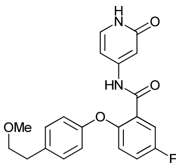
5-fluoro-2-(4-(2-methoxyethyl)phenoxy)-N-(2-oxo-1,2-dihydropyridin-4-yl)benzamide;
