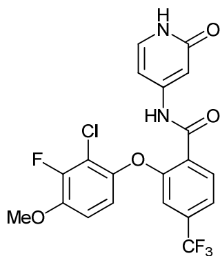
2-(2-chloro-3-fluoro-4-methoxyphenoxy)-N-(2-oxo-1,2-dihydropyridin-4-yl)-4-(trifluoromethyl)benzamide;
