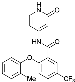
N-(2-oxo-1,2-dihydropyridin-4-yl)-2-(o-toloxo)-5-(trifluoromethyl)benzamide;
