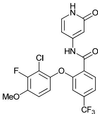
2-(2-chloro-3-fluoro-4-methoxyphenoxy)-N-(2-oxo-1,2-dihydropyridin-4-yl)-4-(trifluoromethyl)benzamide;
