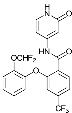
2-(2-(difluoromethoxy)phenoxy)-N-(2-oxo-1,2-dihydropyridin-4-yl)-4-(trifluoromethyl)benzamide;
