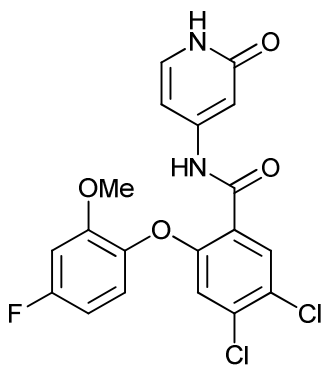
4,5-dichloro-2-(4-fluoro-2-methoxyphenoxy)-N-(2-oxo-1,2-dihydropyridin-4-yl)benzamide.
