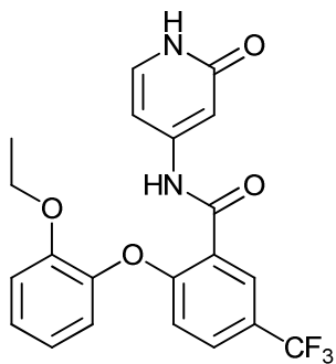
2-(2-ethoxyphenoxy)-N-(2-oxo-1,2-dihydropyridin-4-yl)-5-(trifluoromethyl)benzamide;
