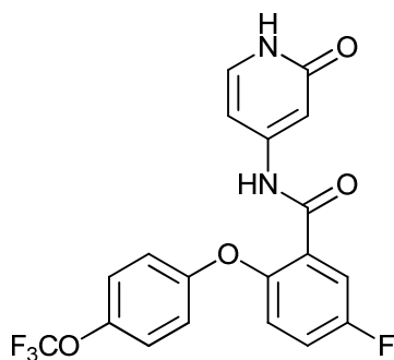
5-fluoro-N-(2-oxo-1,2-dihydropyridin-4-yl)-2-(4-(trifluoromethoxy)phenoxy)benzamide;
