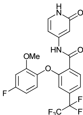
2-(4-fluoro-2-methoxyphenoxy)-N-(2-oxo-1,2-dihydropyridin-4-yl)-4-(perfluoroethyl)benzamide.
