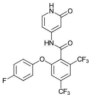
2-(4-fluorophenoxy)-N-(2-oxo-1,2-dihydropyridin-4-yl)-4,6-bis(trifluoromethyl)benzamide;
