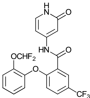
2-(2-(difluoromethoxy)phenoxy)-N-(2-oxo-1,2-dihydropyridin-4-yl)-5-(trifluoromethyl)benzamide;
