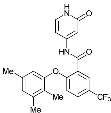
N-(2-oxo-1,2-dihydropyridin-4-yl)-5-(trifluoromethyl)-2-(2,3,5-trimethylphenoxy)benzamide;
