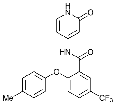
N-(2-oxo-1,2-dihydropyridin-4-yl)-2-(p-tolyloxy)-5-(trifluoromethyl)benzamide;
