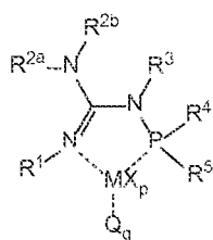
Structure MGu1
