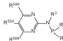
Structure Gu26
