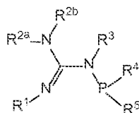
Structure Gu1
