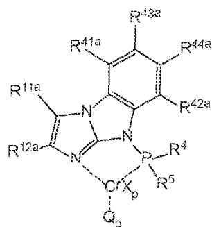
Structure CrGu24
