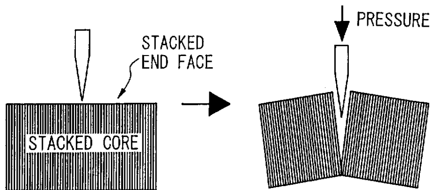
PUSH APART TEST METHOD
