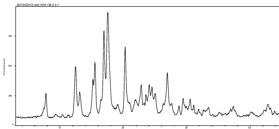
FIG. 8 XRPD Form III
