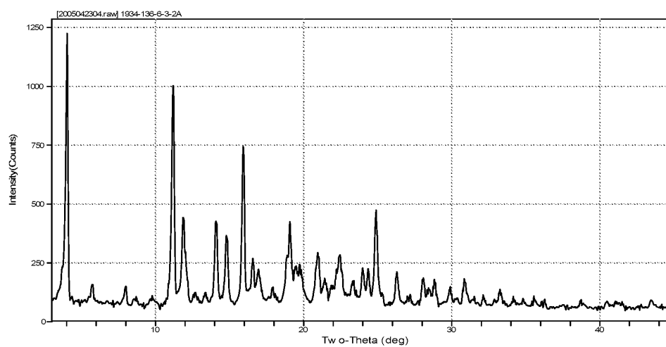
FIG. 20 XRPD Form XIV
