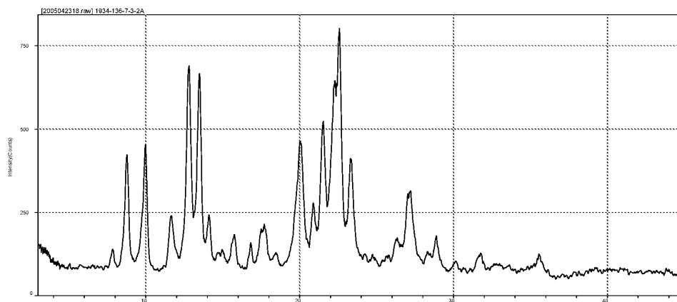
FIG. 7 XRPD Form Ia
