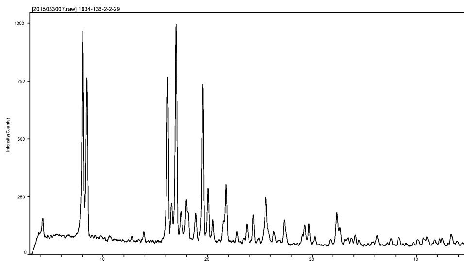
FIG. 14 XRPD Form VIII
