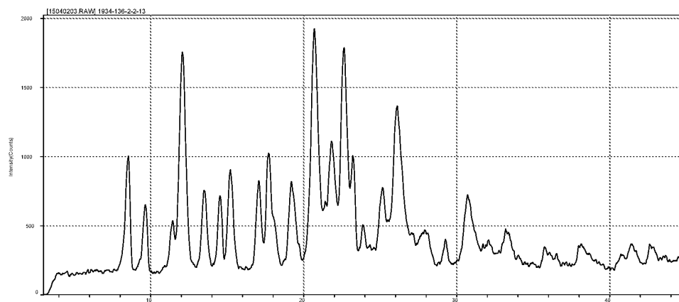
FIG. 12 XRPD Form VI
