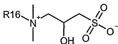
General formula 16
