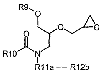
General formula 12
