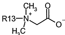
General formula 13
