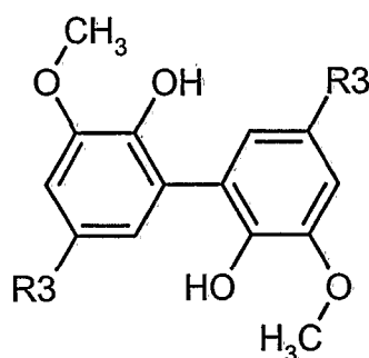
General formula 5
