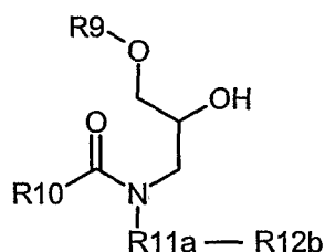
General formula 11
