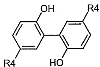
General formula 6
