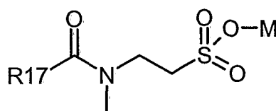
General formula 17
