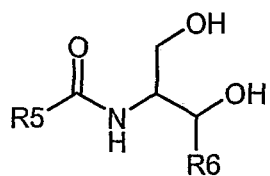
General formula 7
