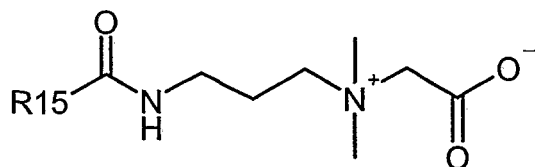
General formula 15
