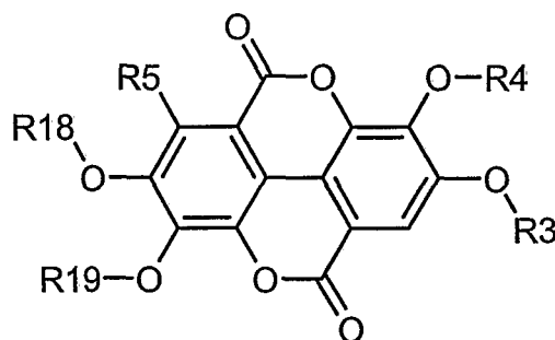
General formula 18
