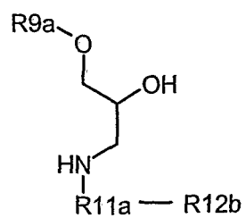
General formula 10
