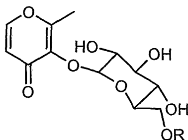
General formula 1
