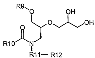
General formula 9
