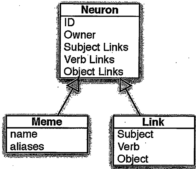
Figure 1: Class Diagram of Poseidon Architecture
