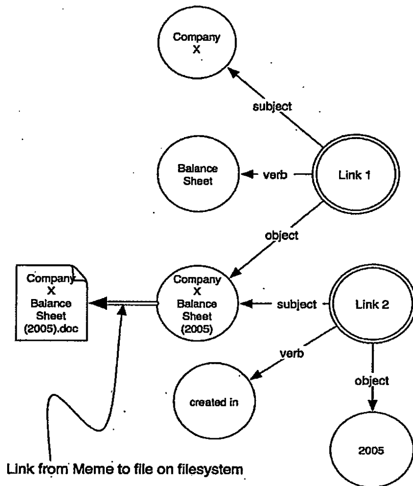
Figure 3: Filesystem Links in the Ontological Model
