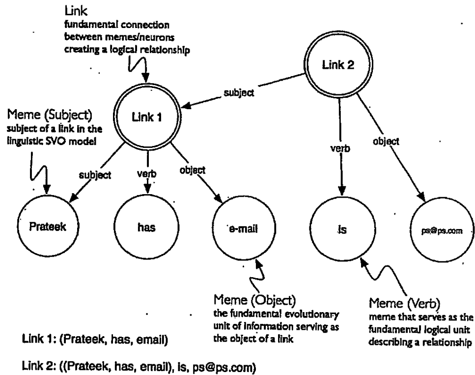
Figure 2: The Ontological Model
