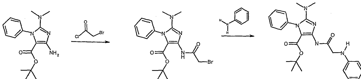
Scheme 9
