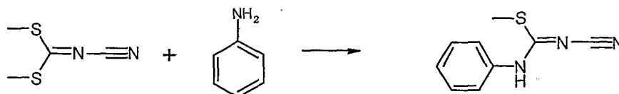
Scheme 8
