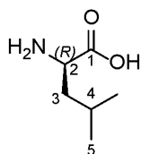
D-leucine (dl)
