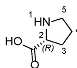
D-proline (dP)
