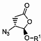
(4R,5R)- IIIa
