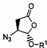
(4S,5S)- IIIb
