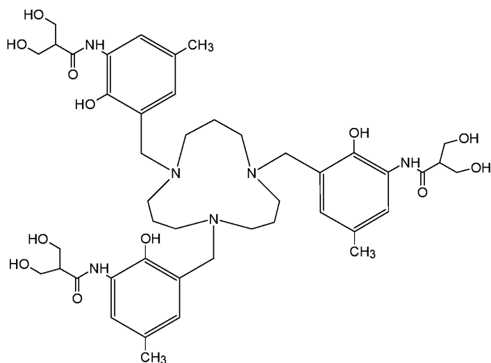
Compound 107 ( N,N,N' -{1,5,9-triazacyclododecane-1,5,9-triyltris[methylene(2-hydroxy-5-methyl-3,1-phenylene)]}tris[3-hydroxy-2-(hydroxymethyl)propanamide]),
