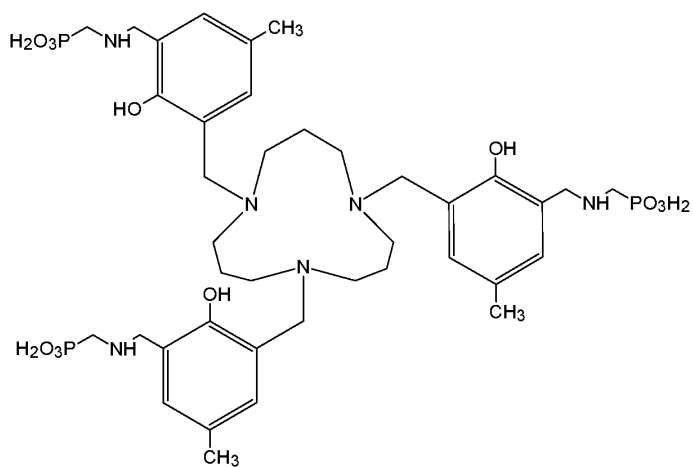
5 Compound 99 ({1,5,9-triazacyclododecane-1,5,9-triyltris[methylene(2-hydroxy-5-methyl-3,1-phenylene)methyleneazanedimethylene]}tris(phosphonic acid)),
