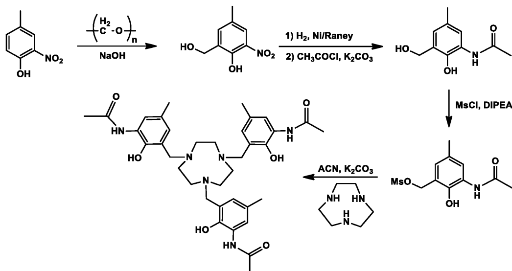
Scheme 6
