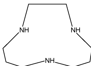
Triazacycloundecane (TACUD)
