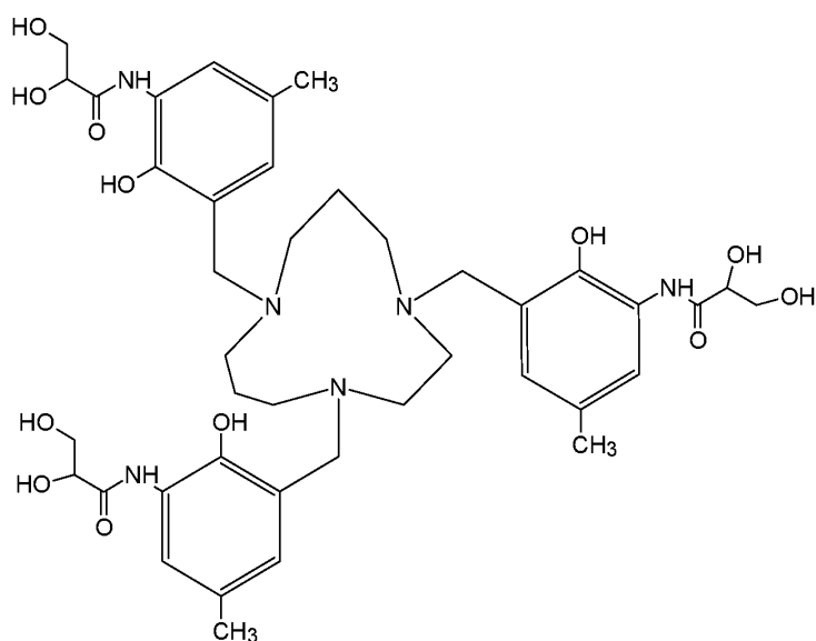
Compound 80 ( N,N',N'' -{1,4,8-triazacycloundecane-1,4,8-triyltris[methylene(2-hydroxy-5-methyl-3,1-phenylene)]}tris(2,3-dihydroxypropanamide)),
