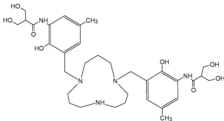
5 Compound 108 ( N,N' -{1,5,9-triazacyclododecane-1,5-diylbis[methylene(2-hydroxy-5-methyl-3,1-phenylene)]}bis[3-hydroxy-2-(hydroxymethyl)propanamide]),
