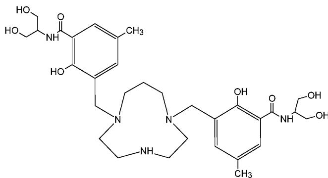
5 Compound 25 (3,3'-[1,4,7-triazecane-1,7-diylbis(methylene)]bis[ N -(1,3-dihydroxypropan-2-yl)-2-hydroxy-5-methylbenzamide]),
