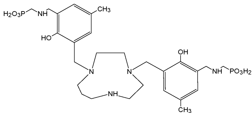
5 Compound 40 ({1,4,7-triazecane-1,4-diylbis[methylene(2-hydroxy-5-methyl-3,1-phenylene)methyleneazanediy lmethylene]}bis(phosphonic acid)),
