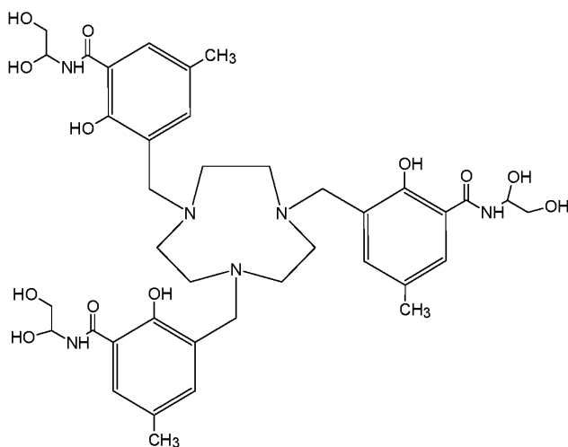
5 Compound 13 (3,3',3''-[1,4,7-triazonane-1,4,7-triyltris(methylene)]tris[ N -(1,2-dihydroxyethyl)-2-hydroxy-5-methylbenzamide]),
