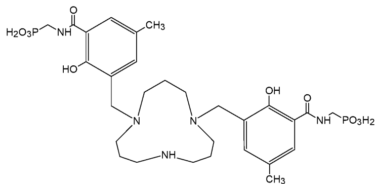
Compound 98 ({1,5,9-triazacyclododecane-1,5-diylbis[methylene(2-hydroxy-5-methyl-3,1-phenylene)carbonylazanedimethylene]}bis(phosphonic acid)),
