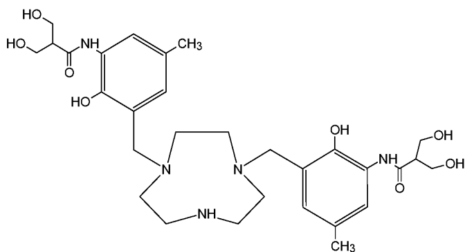
Compound 20 ( N,N' -{1,4,7-triazonane-1,4-diylbis[methylene(2-hydroxy-5-methyl-3,1-phenylene)]}bis[3-hydroxy-2-(hydroxymethyl)propanamide]),
