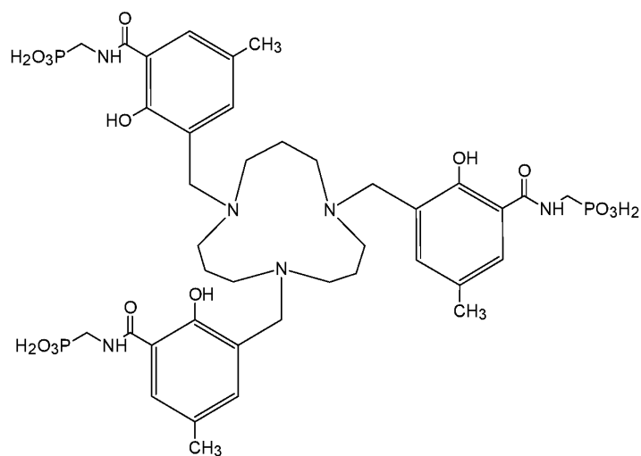
Compound 97 ({1,5,9-triazacyclododecane-1,5,9-triyltris[methylene(2-hydroxy-5-methyl-3,1-phenylene)carbonyl]azanediy[methylene]})tris(phosphonic acid)),
