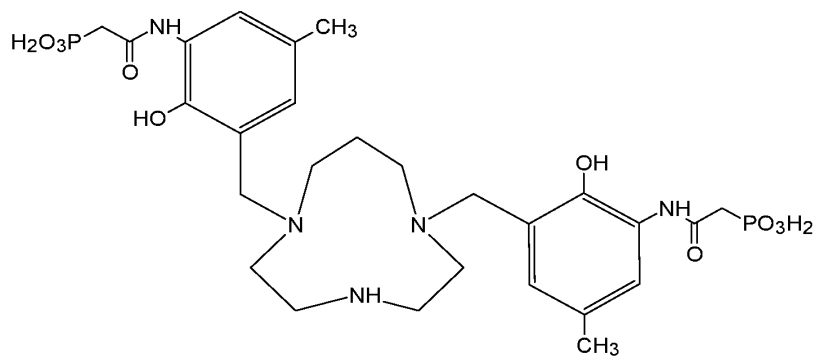
Compound 54 ({1,4,7-triazecane-1,7-diylbis[methylene(2-hydroxy-5-methyl-3,1-phenylene)azanediy](2-oxoethane-2,1-diyl)]}bis(phosphonic acid)),
