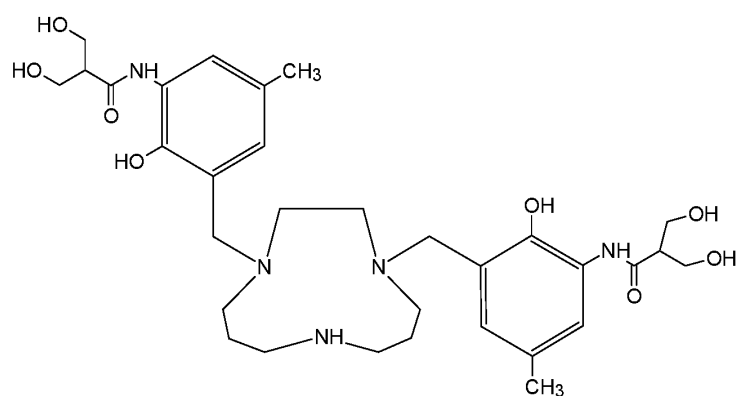
Compound 84 ( N,N' -{1,4,8-triazacycloundecane-1,8-diylbis[methylene(2-hydroxy-5-methyl-3,1-phenylene)]}bis[3-hydroxy-2-(hydroxymethyl)propanamide]),
