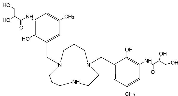
Compound 81 ( N,N' -{1,4,8-triazacycloundecane-1,8-diylbis[methylene(2-hydroxy-5-methyl-3,1-phenylene)]}bis(2,3-dihydroxypropanamide)),
