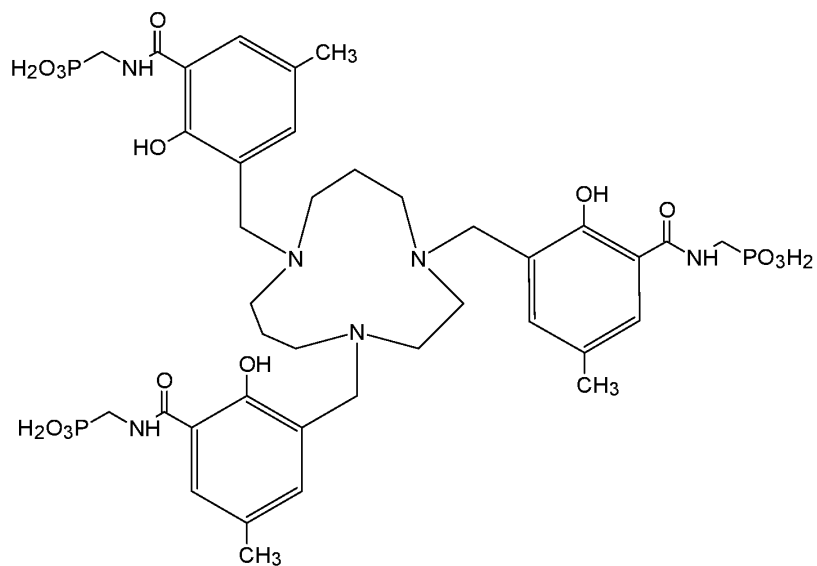
Compound 68 ({1,4,8-triazacycloundecane-1,4,8-triyltris[methylene(2-hydroxy-5-methyl-3,1-phenylene)carbonylazanedimethylene]}tris(phosphonic acid)),
