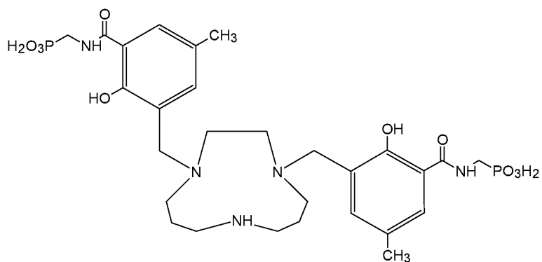
Compound 69 ({1,4,8-triazacycloundecane-1,8-diylbis[methylene(2-hydroxy-5-methyl-3,1-phenylene)carbonylazanedimethylene]}bis(phosphonic acid)),
