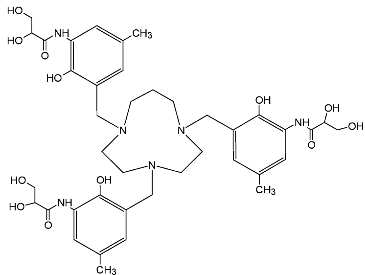
Compound 47 ( N,N',N'' -{1,4,7-triazecane-1,4,7-triyltris[methylene(2-hydroxy-5-methyl-3,1-phenylene)]}tris(2,3-dihydroxypropanamide)),
