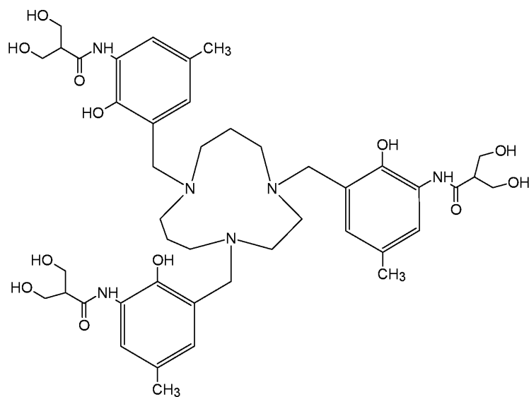
Compound 83 ( N,N',N'' -{1,4,8-triazacycloundecane-1,4,8-triyltris[methylene(2-hydroxy-5-methyl-3,1-phenylene)]}tris[3-hydroxy-2-(hydroxymethyl)propanamide]),
