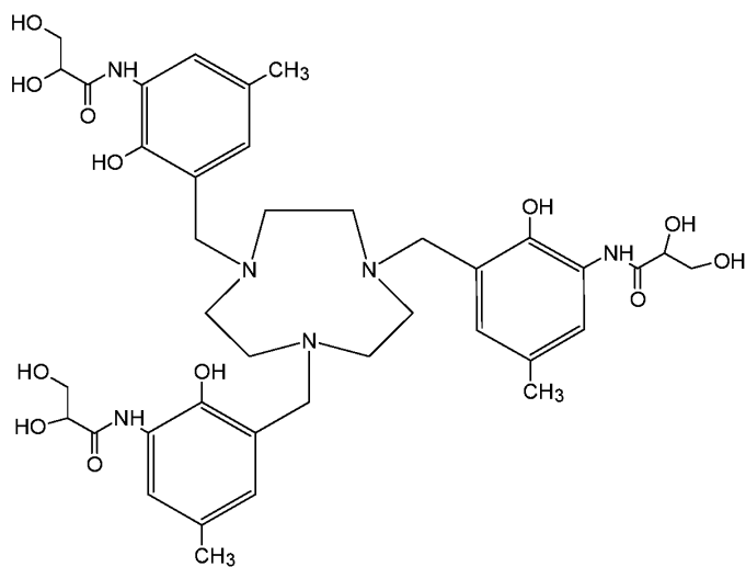
Compound 17 ( N,N,N' -{1,4,7-triazonane-1,4,7-triyltris[methylene(2-hydroxy-5-methyl-3,1-phenylene)]}tris(2,3-dihydroxypropanamide)),
