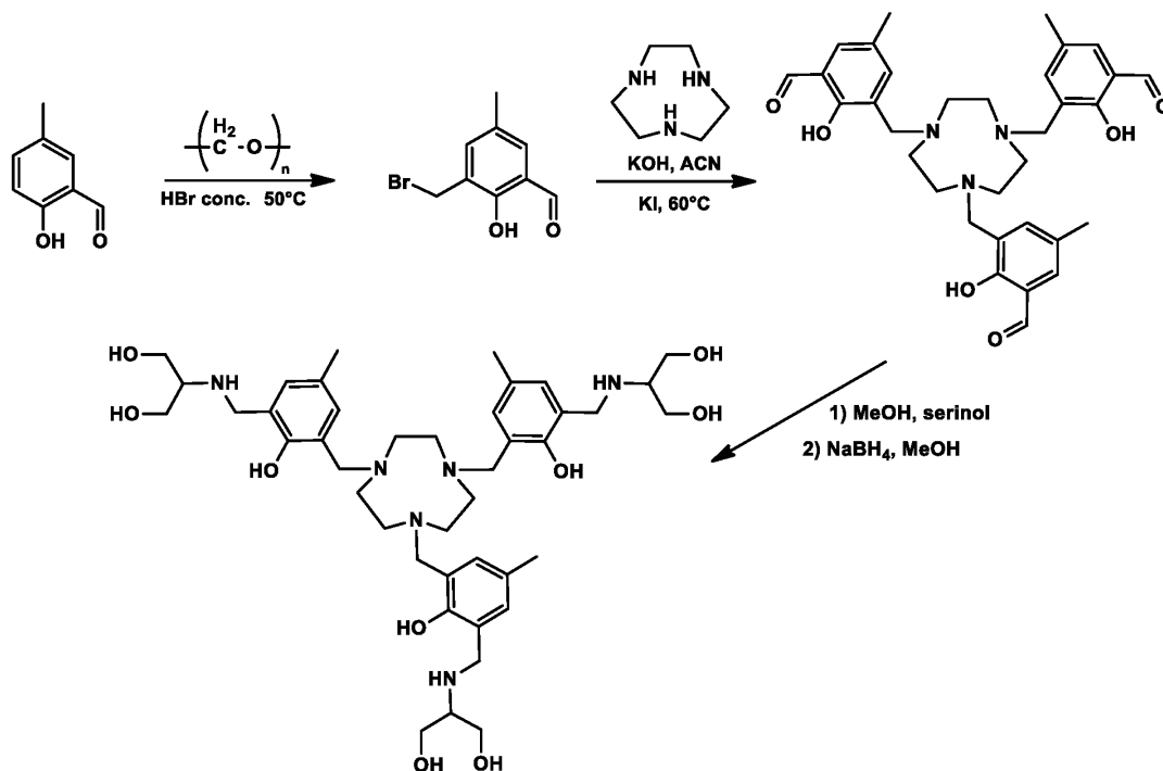
Scheme 9.
