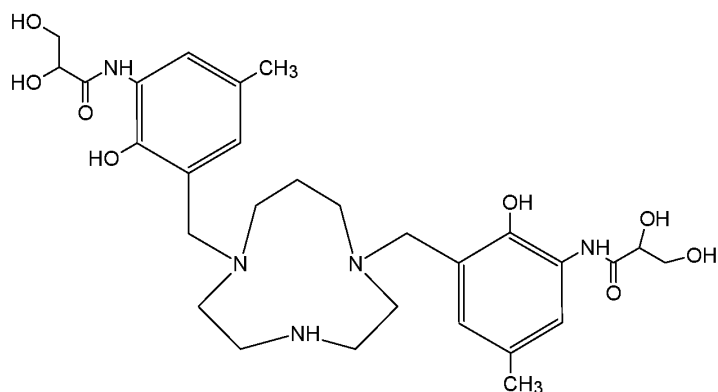
Compound 48 ( N,N' -{1,4,7-triazecane-1,7-diylbis[methylene(2-hydroxy-5-methyl-3,1-phenylene)]}bis(2,3-dihydroxypropanamide)),
