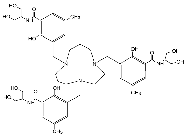
Compound 56 (3,3',3''-[1,4,8-triazacycloundecane-1,4,8-triyltris(methylene)]tris[ N -(1,3-dihydroxypropan-2-yl)-2-hydroxy-5-methylbenzamide]),
