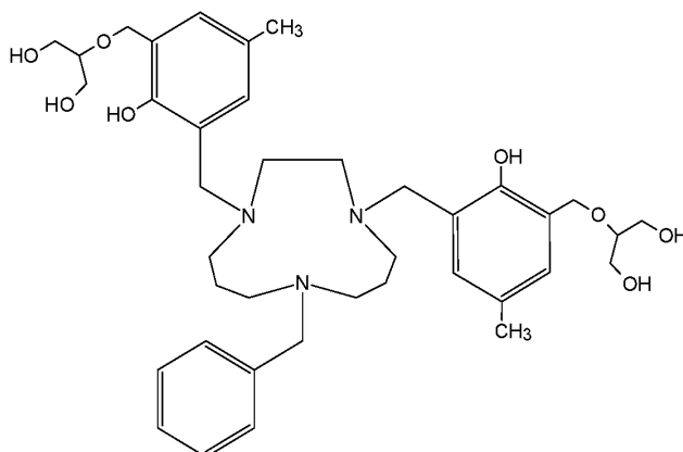
Compound 224 (2,2'-{(8-benzyl-1,4,8-triazacycloundecane-1,4-diyl)bis[methylene(2-hydroxy-5-methyl-3,1-phenylene)methyleneoxy]}di(propane-1,3-diol)), and
