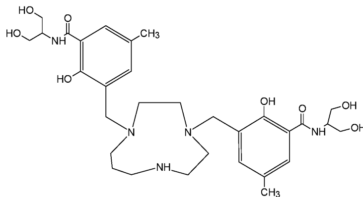
Compound 26 (3,3'-[1,4,7-triazecane-1,4-diylbis(methylene)]bis[ N -(1,3-dihydroxypropan-2-yl)-2-hydroxy-5-methylbenzamide]),
