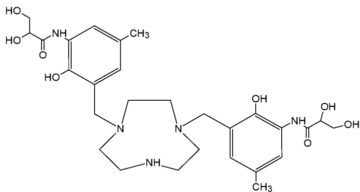
Compound 18 ( N,N' -{1,4,7-triazonane-1,4-diylbis[methylene(2-hydroxy-5-methyl-3,1-phenylene)]}bis(2,3-dihydroxypropanamide)),
