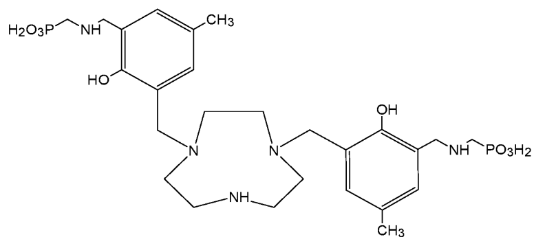
Compound 12 ({1,4,7-triazonane-1,4-diylbis[methylene(2-hydroxy-5-methyl-3,1-phenylene)methyleneazanedimethylene]}bis(phosphonic acid)),
