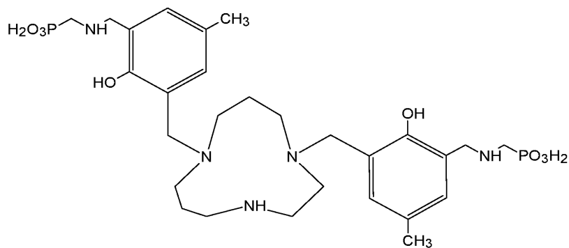
Compound 72 ({1,4,8-triazacycloundecane-1,8-diylbis[methylene(2-hydroxy-5-methyl-3,1-phenylene)methyleneazanediy(methylene)]}bis(phosphonic acid)),
