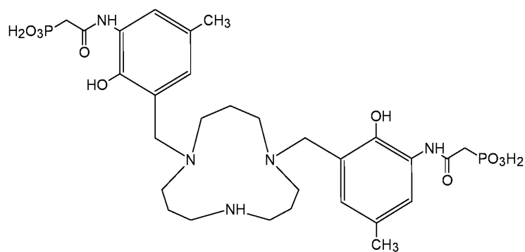
Compound 110 ({1,5,9-triazacyclododecane-1,5-diylbis[methylene(2-hydroxy-5-methyl-3,1-phenylene)azanediyl(2-oxoethane-2,1-diyl)]}bis(phosphonic acid)),
