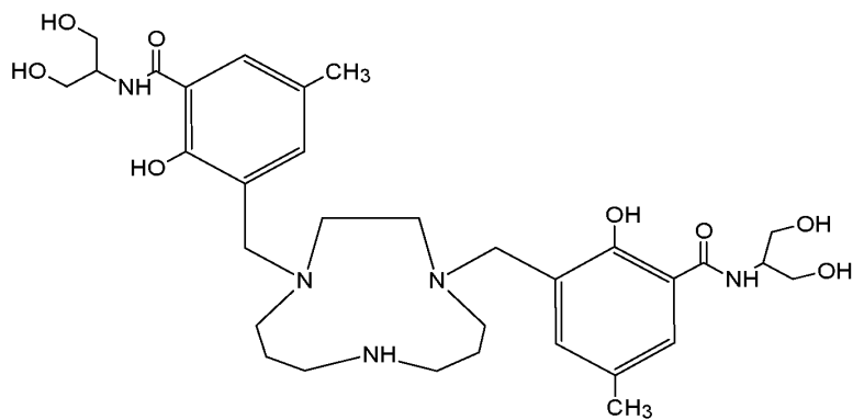
Compound 59 (3,3'-[1,4,8-triazacycloundecane-1,4-diylbis(methylene)]bis[ N -(1,3-dihydroxypropan-2-yl)-2-hydroxy-5-methylbenzamide]),
