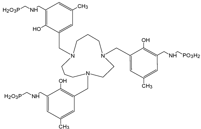
Compound 71 ({1,4,8-triazacycloundecane-1,4,8-triyltris[methylene(2-hydroxy-5-methyl-3,1-phenylene)methyleneazanedimethylene]}tris(phosphonic acid)),
