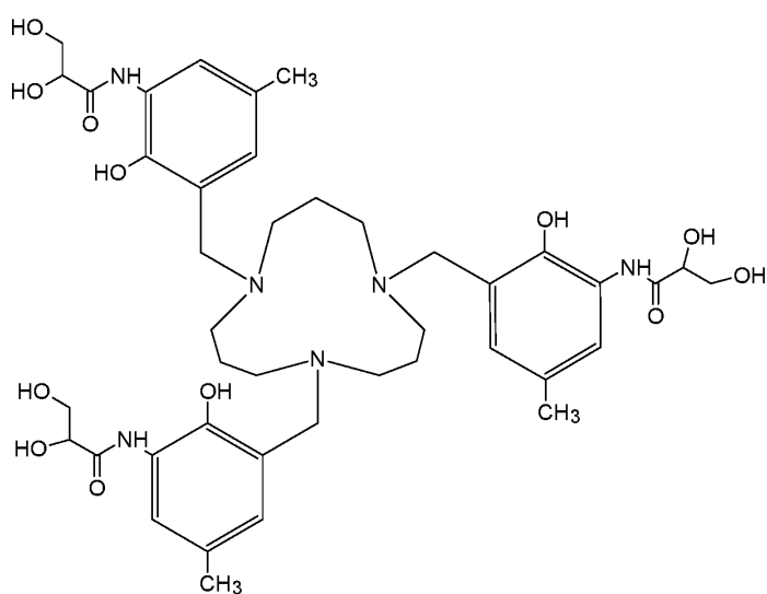
5 Compound 105 ( N,N,N' -{1,5,9-triazacyclododecane-1,5,9-triyltris[methylene(2-hydroxy-5-methyl-3,1-phenylene)]}tris(2,3-dihydroxypropanamide)),
