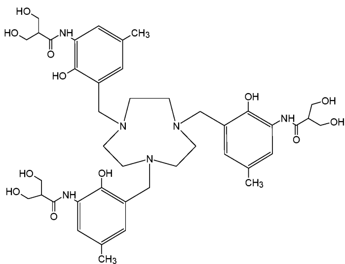
5 Compound 19 ( N,N,N' -{1,4,7-triazonane-1,4,7-triyltris[methylene(2-hydroxy-5-methyl-3,1-phenylene)]}tris[3-hydroxy-2-(hydroxymethyl)propanamide]),
