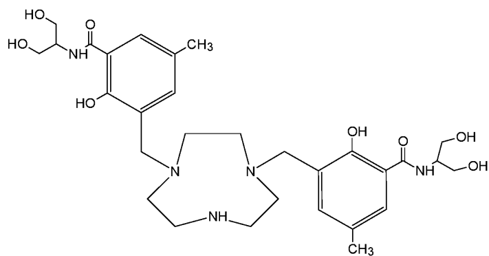
Compound 3 (3,3'-[1,4,7-triazonane-1,4-diylbis(methylene)]bis[ N -(1,3-dihydroxypropan-2-yl)-2-hydroxy-5-methylbenzamide]),
