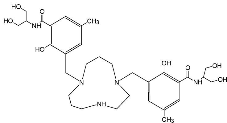
5 Compound 58 (3,3'-[1,4,8-triazacycloundecane-1,8-diylbis(methylene)]bis[ N -(1,3-dihydroxypropan-2-yl)-2-hydroxy-5-methylbenzamide]),
