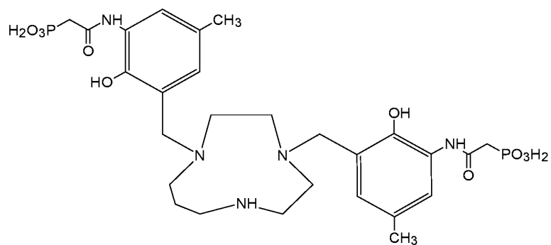
5 Compound 55 ({1,4,7-triazecane-1,4-diylbis[methylene(2-hydroxy-5-methyl-3,1-phenylene)azanediy](2-oxoethane-2,1-diyl)]}bis(phosphonic acid)),
