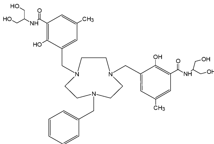
5 Compound 111 (3,3'-[(7-benzyl-1,4,7-triazonane-1,4-diyl)bis(methylene)]bis[ N -(1,3-dihydroxypropan-2-yl)-2-hydroxy-5-methylbenzamide]),
