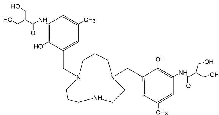
Compound 84 ( N,N' -{1,4,8-triazacycloundecane-1,8-diylbis[methylene(2-hydroxy-5-methyl-3,1-phenylene)]}bis[3-hydroxy-2-(hydroxymethyl)propanamide]),
