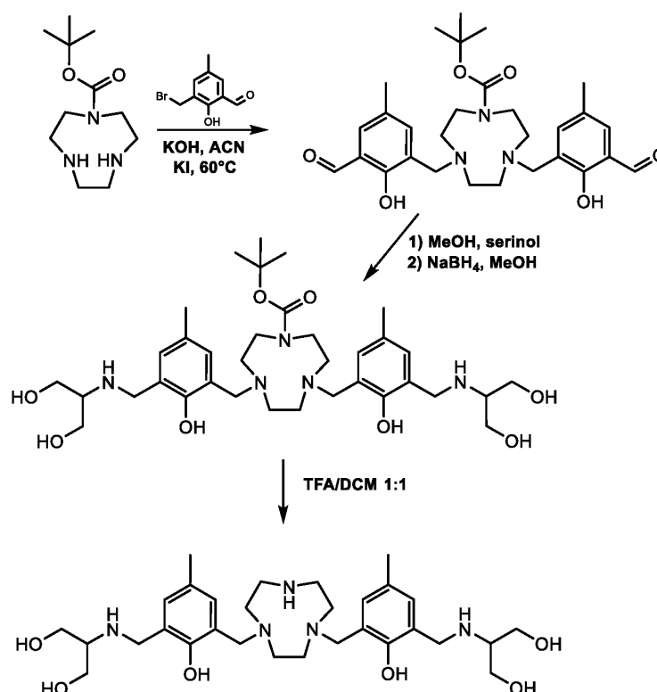
Scheme 10
