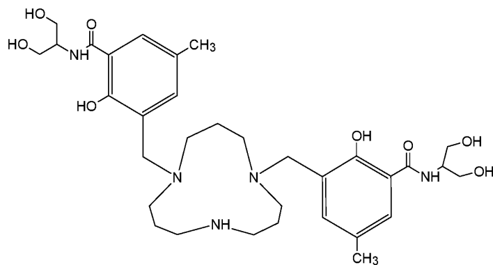
5 Compound 91 (3,3'-[1,5,9-triazacyclododecane-1,5-diylbis(methylene)]bis[ N -(1,3-dihydroxypropan-2-yl)-2-hydroxy-5-methylbenzamide]),
