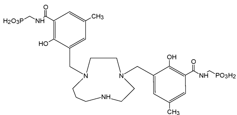
5 Compound 37 ({1,4,7-triazecane-1,4-diylbis[methylene(2-hydroxy-5-methyl-3,1-phenylene)carbonylazanediylmethylene]}bis(phosphonic acid)),
