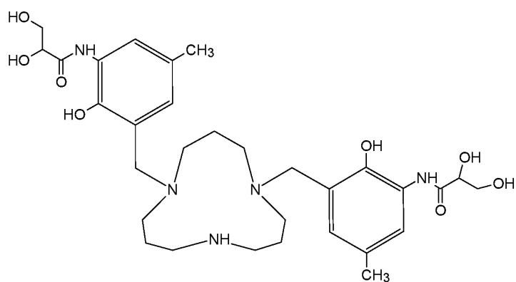
Compound 106 ( N,N' -{1,5,9-triazacyclododecane-1,5-diylbis[methylene(2-hydroxy-5-methyl-3,1-phenylene)]}bis(2,3-dihydroxypropanamide)),
