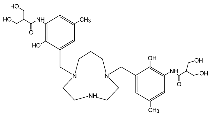
Compound 51 ( N,N' -{1,4,7-triazecane-1,7-diylbis[methylene(2-hydroxy-5-methyl-3,1-phenylene)]}bis[3-hydroxy-2-(hydroxymethyl)propanamide]),
