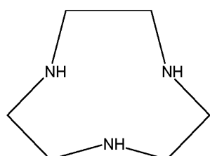
Triazacyclononane (TACN)
