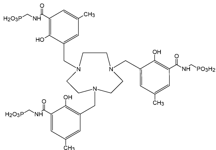
Compound 9 ({1,4,7-triazonane-1,4,7-triyltris[methylene(2-hydroxy-5-methyl-3,1-phenylene)carbonylazanedimethylene]}tris(phosphonic acid)),
