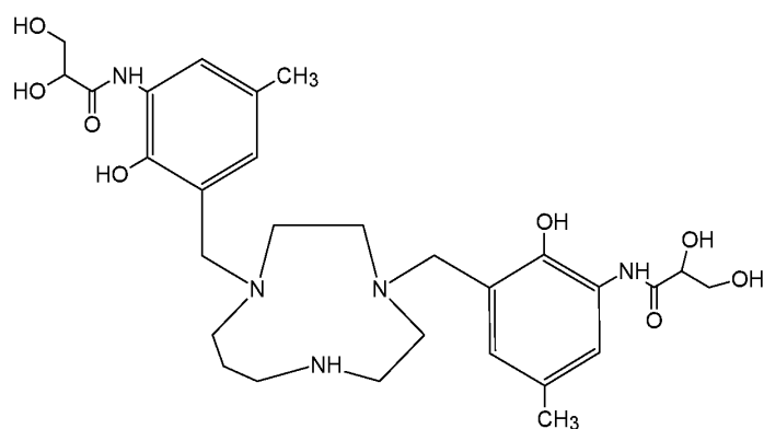
5 Compound 49 ( N,N' -{1,4,7-triazecane-1,4-diylbis[methylene(2-hydroxy-5-methyl-3,1-phenylene)]}bis(2,3-dihydroxypropanamide)),
