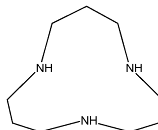
Triazacyclododecane (TADD)
