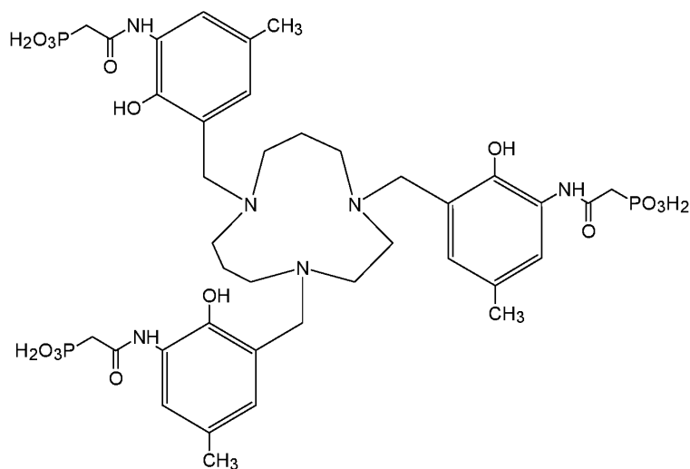
Compound 86 ({1,4,8-triazacycloundecane-1,4,8-triyltris[methylene(2-hydroxy-5-methyl-3,1-phenylene)azanediyl(2-oxoethane-2,1-diyl)]}tris(phosphonic acid)),
