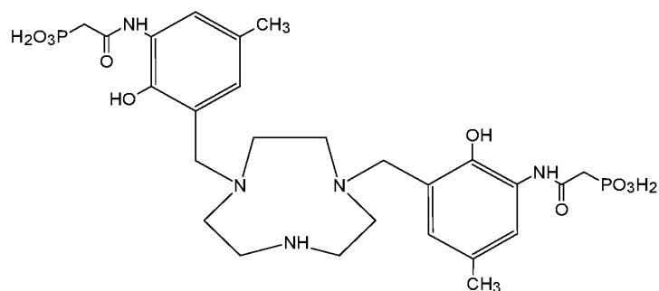
5 Compound 22 ({1,4,7-triazonane-1,4-diylbis[methylene(2-hydroxy-5-methyl-3,1-phenylene)azanediyl(2-oxoethane-2,1-diyl)]}bis(phosphonic acid)),
