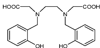
HBED
