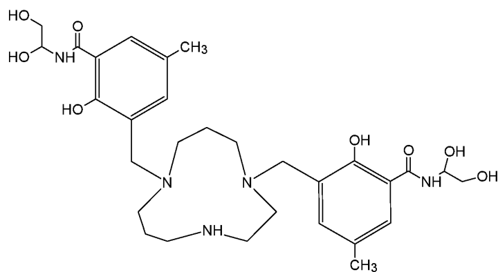
5 Compound 76 (3,3'-[1,4,8-triazacycloundecane-1,8-diylbis(methylene)]bis[ N -(1,2-dihydroxyethyl)-2-hydroxy-5-methylbenzamide]),
