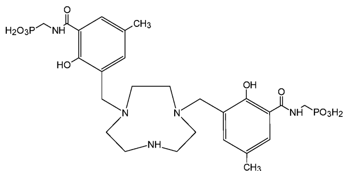
5 Compound 10 ({1,4,7-triazonane-1,4-diylbis[methylene(2-hydroxy-5-methyl-3,1-phenylene)carbonylazanedimethylene]}bis(phosphonic acid)),
