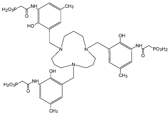
Compound 109 ({1,5,9-triazacyclododecane-1,5,9-triyltris[methylene(2-hydroxy-5-methyl-3,1-phenylene)azanediyl(2-oxoethane-2,1-diyl)]}tris(phosphonic acid)),
