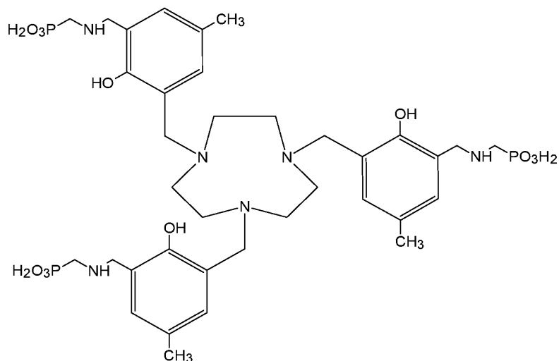
Compound 11 ({1,4,7-triazonane-1,4,7-triyltris[methylene(2-hydroxy-5-methyl-3,1-phenylene)methyleneazanedimethylene]}tris(phosphonic acid)),
