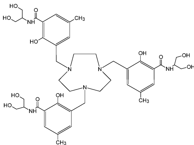
Compound 1 (3,3',3''-[1,4,7-triazonane-1,4,7-triyltris(methylene)]tris[ N -(1,3-dihydroxypropan-2-yl)-2-hydroxy-5-methylbenzamide]),
