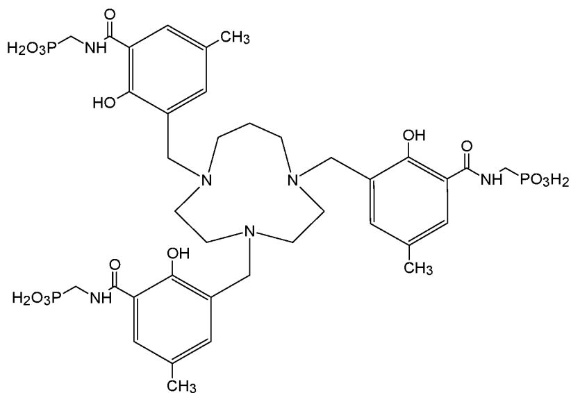
Compound 35 ({1,4,7-triazecane-1,4,7-triyltris[methylene(2-hydroxy-5-methyl-3,1-phenylene)carbonylazanedimethylene]}tris(phosphonic acid)),
