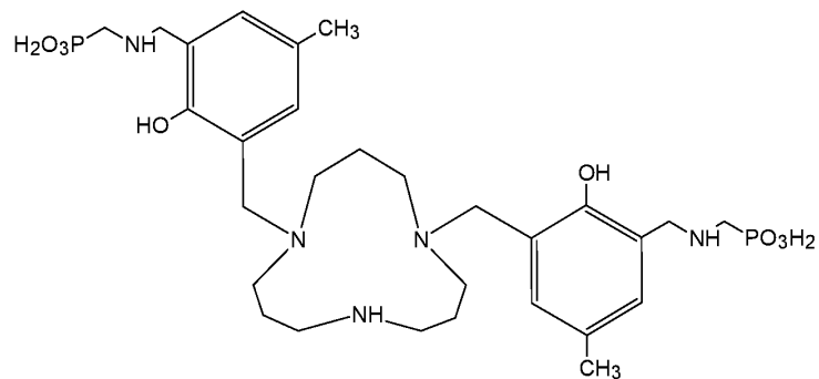
Compound 100 ({1,5,9-triazacyclododecane-1,5-diylbis[methylene(2-hydroxy-5-methyl-3,1-phenylene)methyleneazanedimethylene]}bis(phosphonic acid)),
