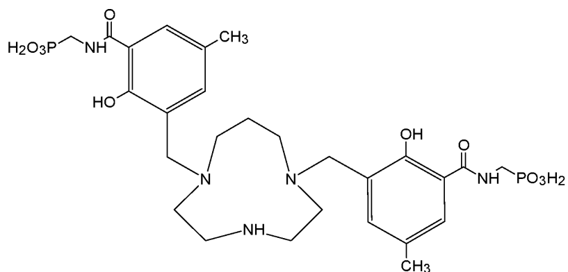
Compound 36 ({1,4,7-triazecane-1,7-diylbis[methylene(2-hydroxy-5-methyl-3,1-phenylene)carbonylazanediylmethylene]}bis(phosphonic acid)),
