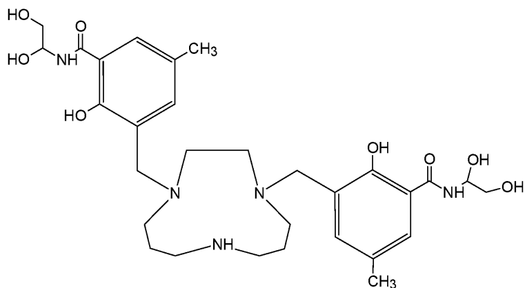
Compound 77 (3,3'-[1,4,8-triazacycloundecane-1,4-diylbis(methylene)]bis[ N -(1,2-dihydroxyethyl)-2-hydroxy-5-methylbenzamide]),
