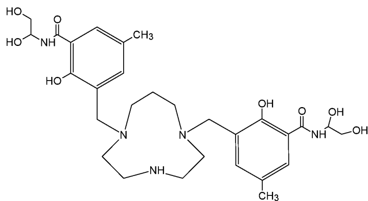
5 Compound 43 (3,3'-[1,4,7-triazecane-1,7-diylbis(methylene)]bis[ N -(1,2-dihydroxyethyl)-2-hydroxy-5-methylbenzamide]),
