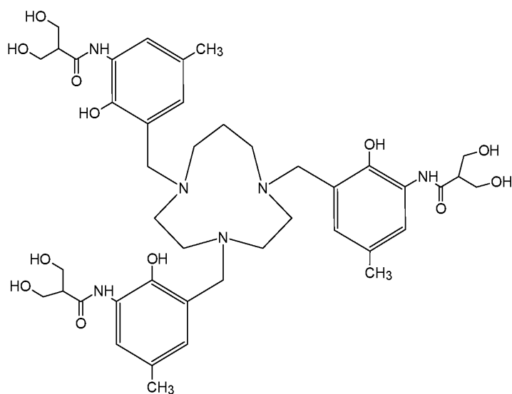
Compound 50 ( N,N',N'' -{1,4,7-triazecane-1,4,7-triyltris[methylene(2-hydroxy-5-methyl-3,1-phenylene)]}tris[3-hydroxy-2-(hydroxymethyl)propanamide]),
