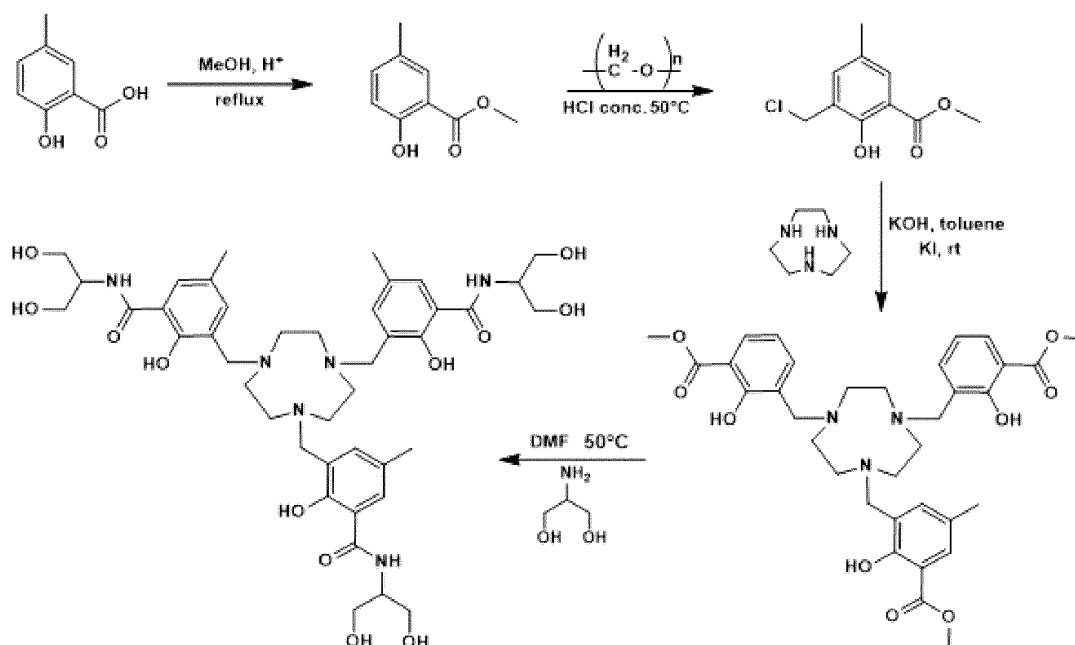
Scheme 8.
