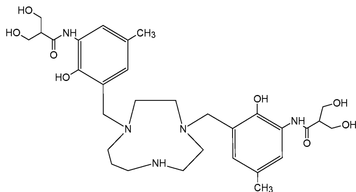
5 Compound 52 ( N,N' -{1,4,7-triazecane-1,4-diylbis[methylene(2-hydroxy-5-methyl-3,1-phenylene)]}bis[3-hydroxy-2-(hydroxymethyl)propanamide]),
