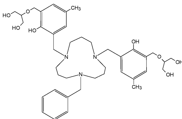
Compound 224 (2,2'-{(8-benzyl-1,4,8-triazacycloundecane-1,4-diyl)bis[methylene(2-hydroxy-5-methyl-3,1-phenylene)methyleneoxy]}di(propane-1,3-diol)), and
