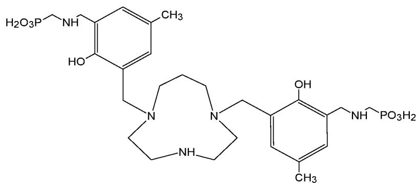
Compound 39 ({1,4,7-triazecane-1,7-diylbis[methylene(2-hydroxy-5-methyl-3,1-phenylene)methyleneazanediy lmethylene]}bis(phosphonic acid)),
