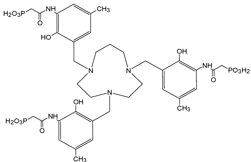
Compound 53 ({1,4,7-triazecane-1,4,7-triyltris[methylene(2-hydroxy-5-methyl-3,1-phenylene)azanediyl(2-oxoethane-2,1-diyl)]}tris(phosphonic acid)),
