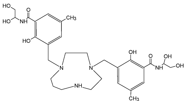
Compound 44 (3,3'-[1,4,7-triazecane-1,4-diylbis(methylene)]bis[ N -(1,2-dihydroxyethyl)-2-hydroxy-5-methylbenzamide]),
