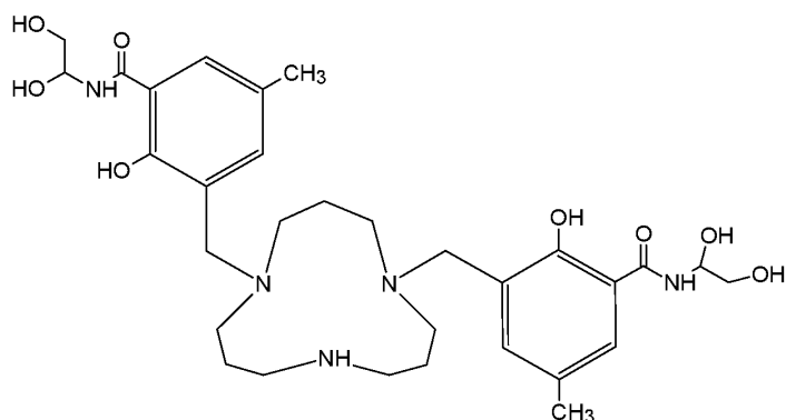
Compound 103 (3,3'-[1,5,9-triazacyclododecane-1,5-diylbis(methylene)]bis[ N -(1,2-dihydroxyethyl)-2-hydroxy-5-methylbenzamide]),
