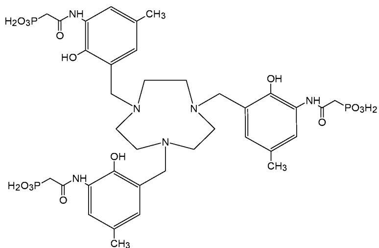
Compound 21 ({1,4,7-triazonane-1,4,7-triyltris[methylene(2-hydroxy-5-methyl-3,1-phenylene)azanediyl(2-oxoethane-2,1-diyl)]}tris(phosphonic acid)),
