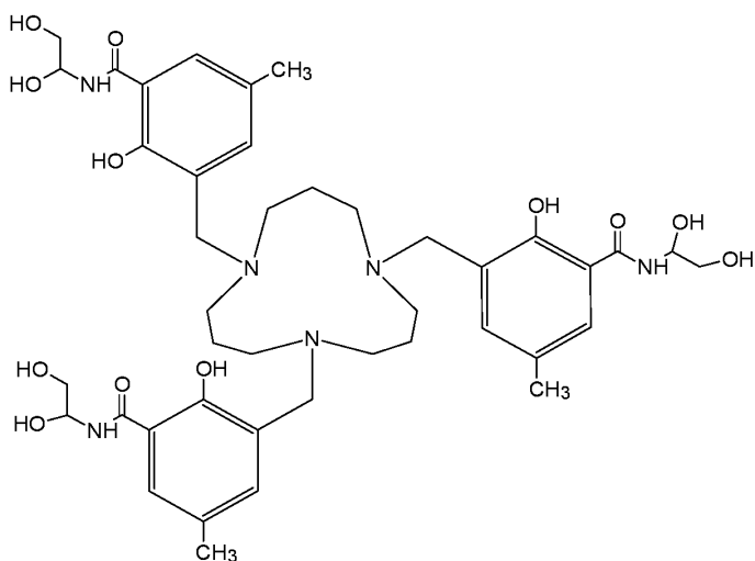
Compound 101 (3,3',3''-[1,5,9-triazacyclododecane-1,5,9-triyltris(methylene)]tris[ N -(1,2-dihydroxyethyl)-2-hydroxy-5-methylbenzamide]),
