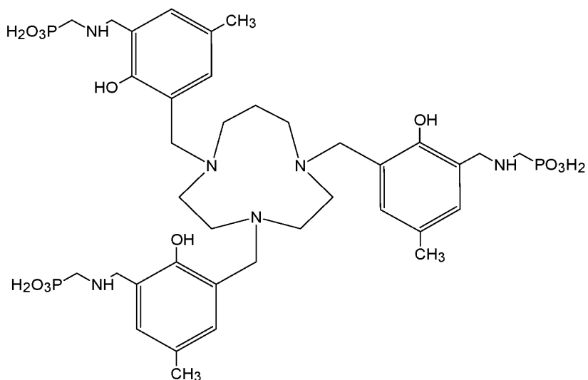
Compound 38 ({1,4,7-triazecane-1,4,7-triyltris[methylene(2-hydroxy-5-methyl-3,1-phenylene)methyleneazanediylmethylene]}tris(phosphonic acid)),
