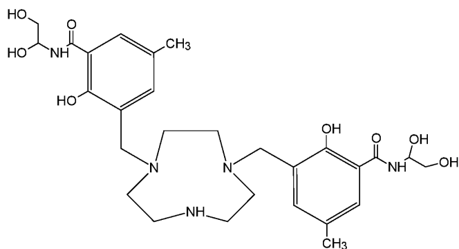
Compound 15 (3,3'-[1,4,7-triazonane-1,4-diylbis(methylene)]bis[ N -(1,2-dihydroxyethyl)-2-hydroxy-5-methylbenzamide]),
