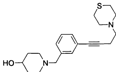
1-[3-(4-Thiomorpholin-4-yl-but-1-ynyl)-benzyl]-piperidin-4-ol
