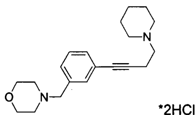
4-[3-(4-Piperidin-1-yl-but-1-ynyl)-benzyl]-morpholine dihydrochloride
