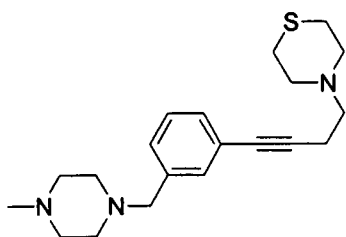
4-{4-[3-(4-Methyl-piperazin-1-ylmethyl)-phenyl]-but-3-ynyl}-thiomorpholine
