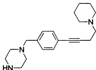
1-[4-(4-Piperidin-1-yl-but-1-ynyl)-benzyl]-piperazine
