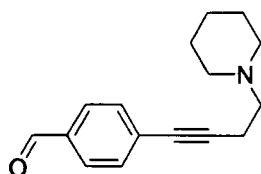
4-(4-Piperidin-1-yl-but-1-ynyl)-benzaldehyde
