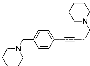
1-[4-(4-Piperidin-1-ylmethyl-phenyl)-but-3-ynyl]-piperidine K_i = 1.6 \text{ nM}
