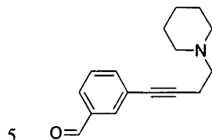
3-(4-Piperidin-1-yl-but-1-ynyl)-benzaldehyde
