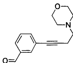
3-(4-Morpholin-4-yl-but-1-ynyl)-benzaldehyde
