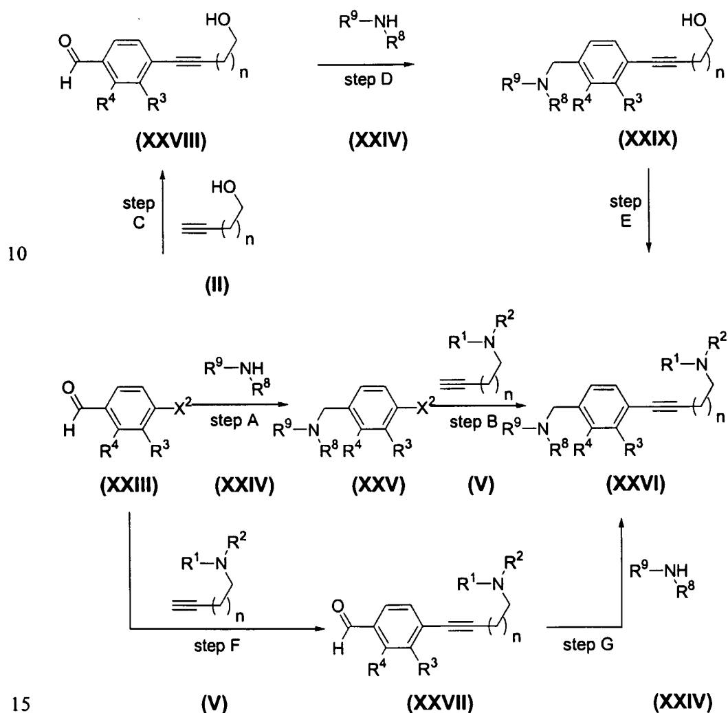
Scheme 5
