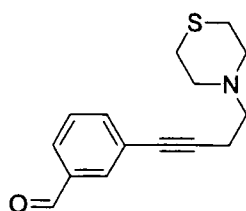
3-(4-Thiomorpholin-4-yl-but-1-ynyl)-benzaldehyde
