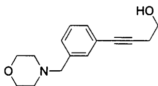
4-(3-Morpholin-4-ylmethyl-phenyl)-but-3-yn-1-ol
