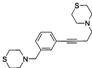
4-[3-(4-Thiomorpholin-4-yl-but-1-ynyl)-benzyl]-thiomorpholine
