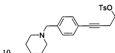
Toluene-4-sulfonic acid 4-(4-piperidin-1-ylmethyl-phenyl)-but-3-ynyl ester
