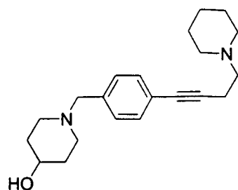
1-[4-(4-Piperidin-1-yl-but-1-ynyl)-benzyl]-piperidin-4-ol
