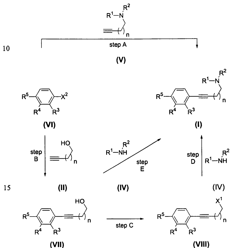
Scheme 2.
