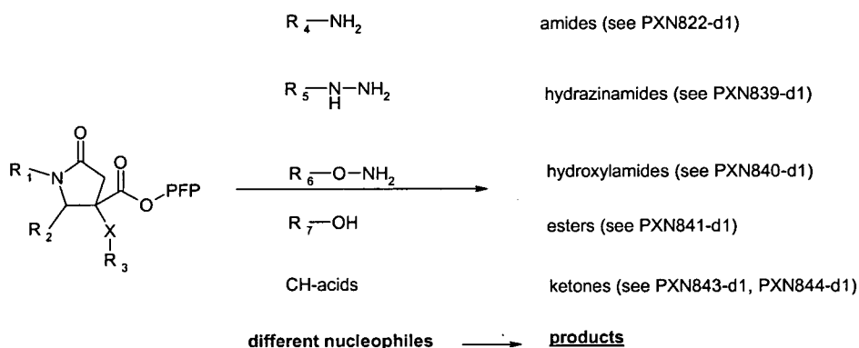
Scheme 4
