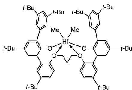
Procatalyst 2
