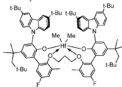
Procatalyst 3
