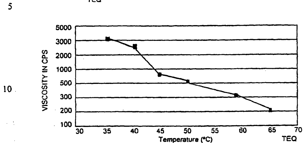
Viscosity vs Temperature Profile TEQ
