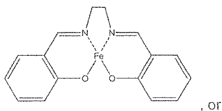
Formula (IV):
