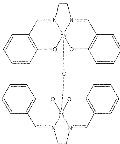
Formula (IV):
