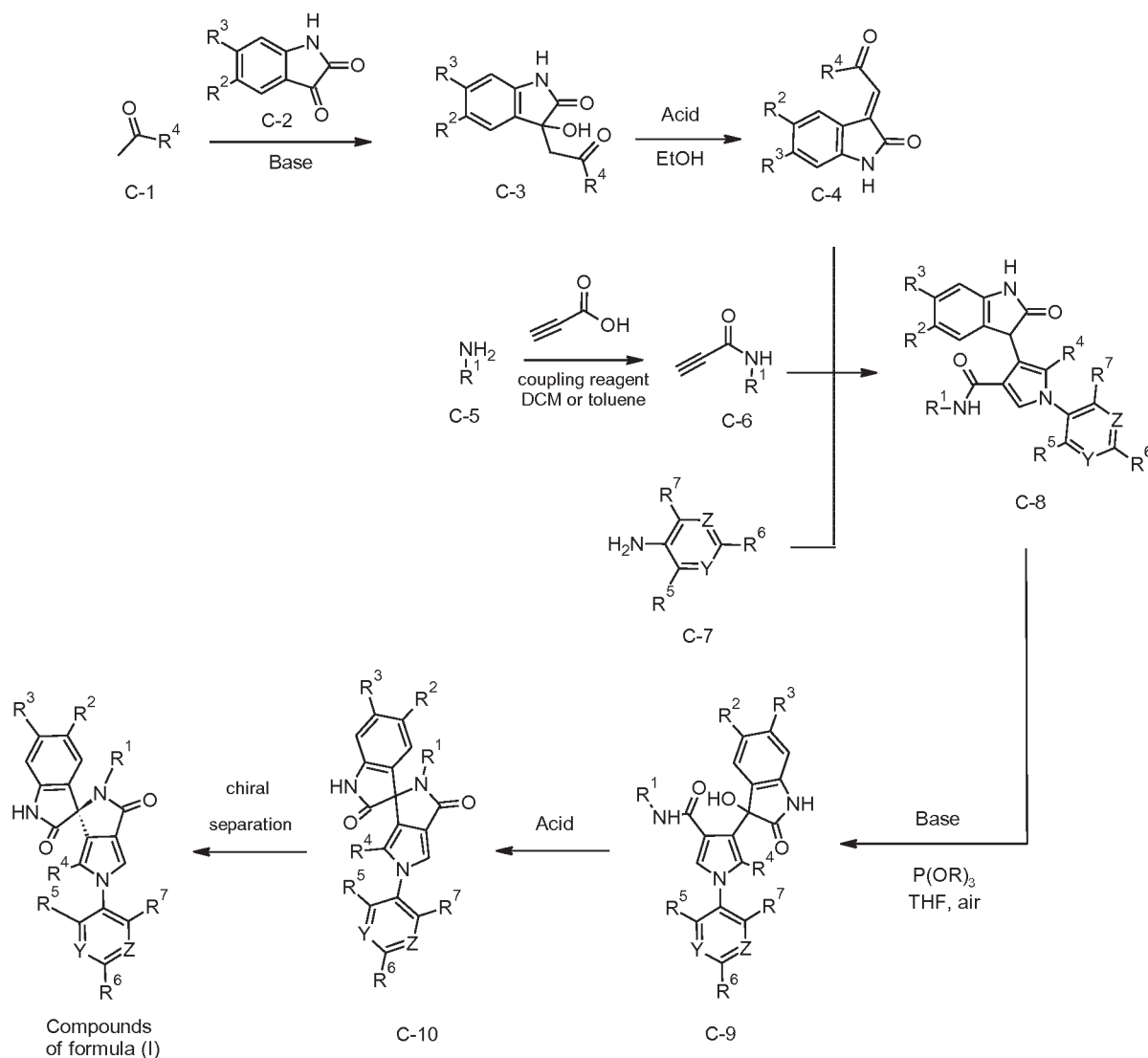
Reaction Scheme 1.
