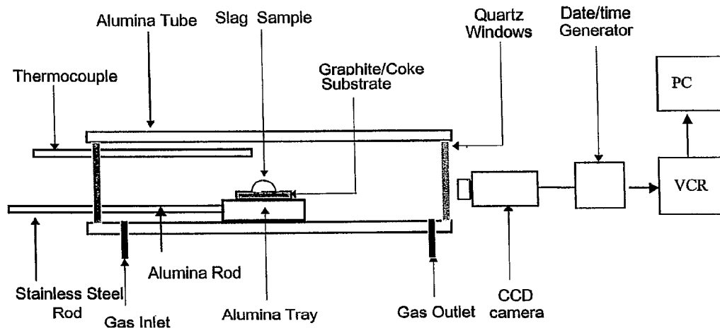
Schematic diagram of the experimental set-up
