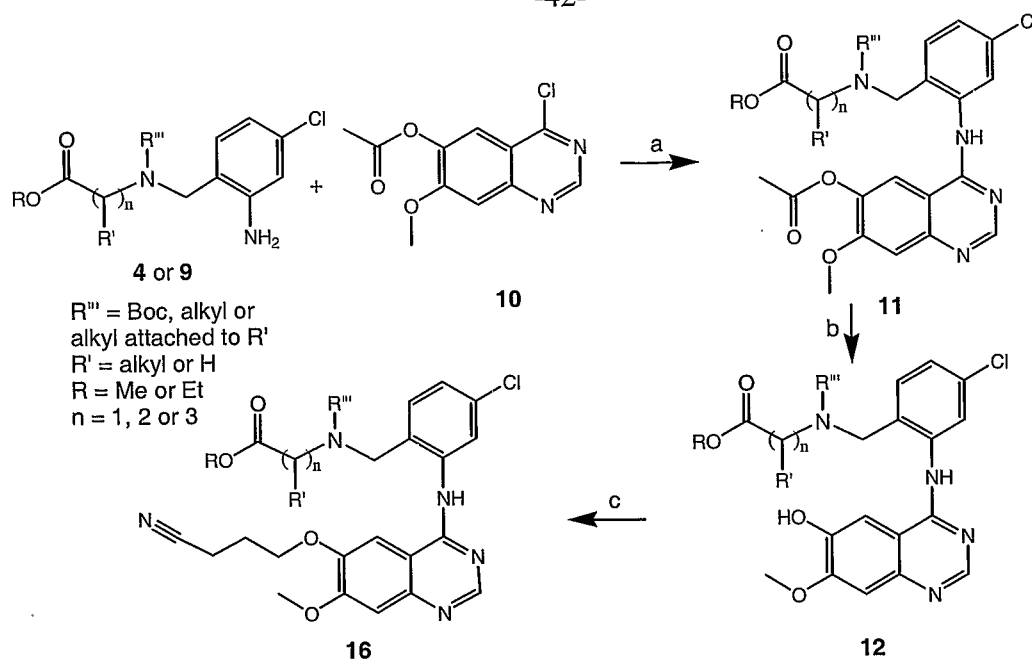
Scheme 10a. a) iPrOH, 80 °C, 2-24 h b) 6 N \text{NH}_3 / MeOH, RT, 1 h c) \text{Br}(\text{CH}_2)_3\text{CN} , \text{Cs}_2\text{CO}_3 , DMF, RT, overnight
