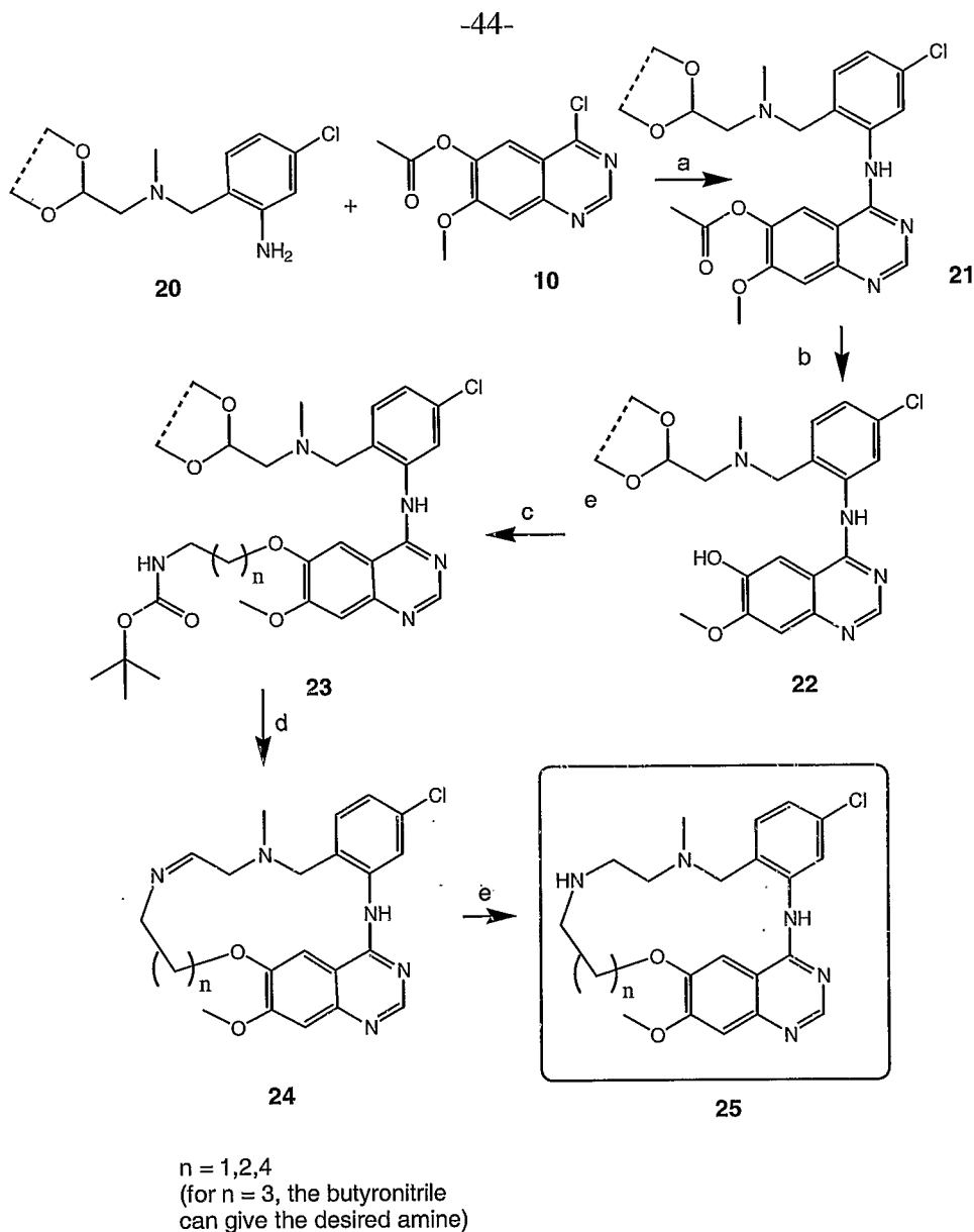
Scheme 11. a) iPrOH, 80 °C, 7-8 h b) NH 3 / MeOH, 1 h c) BrCH 2 (CH 2 ) n NHBoc ( n = 1, 2, 4 ),* Cs 2 CO 3 , DMF, overnight. *Br(CH 2 ) 3 CN used instead of n = 3 d) 6 N HCl, dioxane, 60 °C, 24 h e) NaBH(OAc) 3 , CH 2 Cl 2 , RT, 1h.
