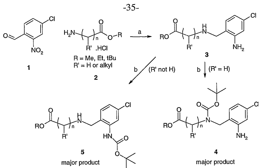
Scheme 5a. a) 1 atm \text{H}_2 , Pt/C, KF, thiophene, MeOH, 50 °C, 1-2 days b) \text{Boc}_2\text{O} , MeOH, RT, 1-3 h.
