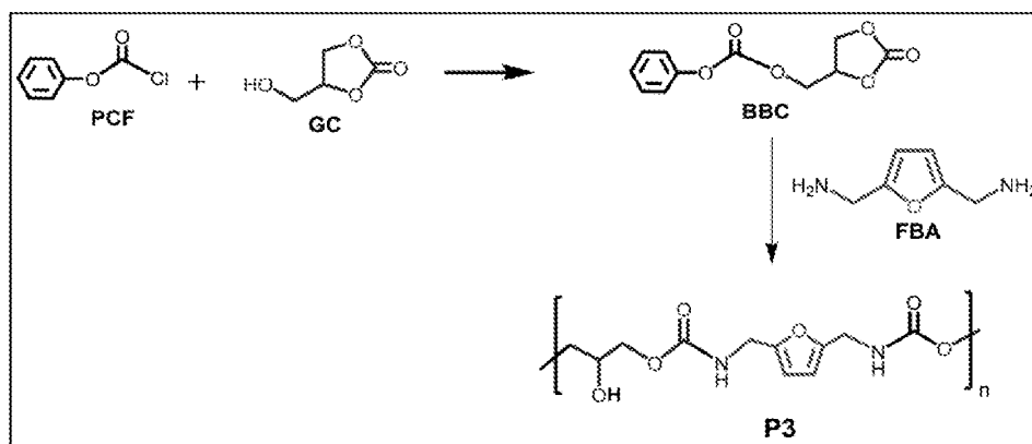
5 Scheme 3.3. Synthesis of polyhydrourethane P3 starting from phenyl chloroformate (PCF) and glycerol carbonate (GC) as starting materials
