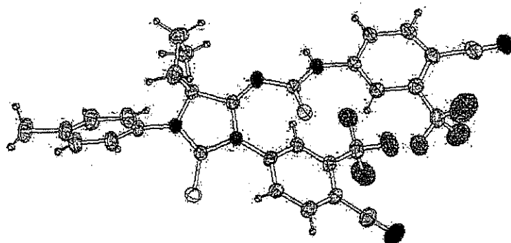
X-ray structure of 35a
