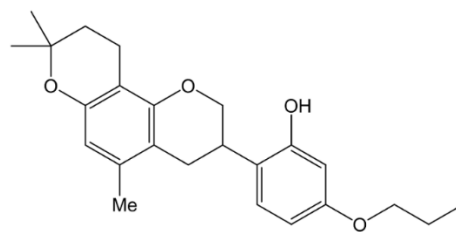
<Compound I -24>
