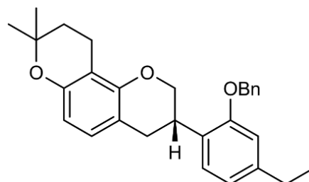
<Compound 6-13b>
