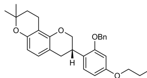
<Compound 6-3b>
