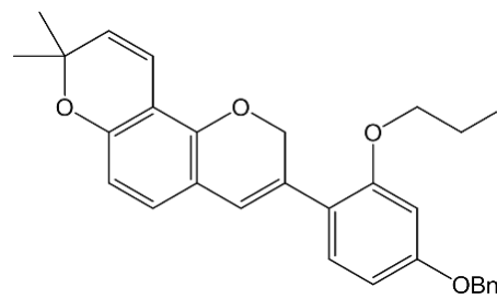
<Compound 5-14>
