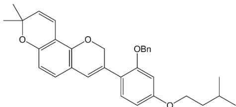
<Compound 5-9>
