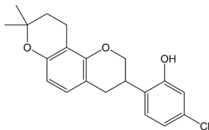
<Compound I -22>
