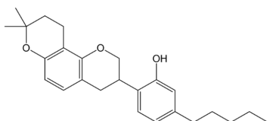
<Compound I -17>
