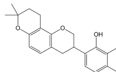
<Compound I -18>
