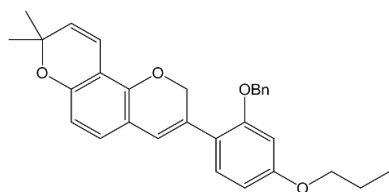
<Compound 5-3>
