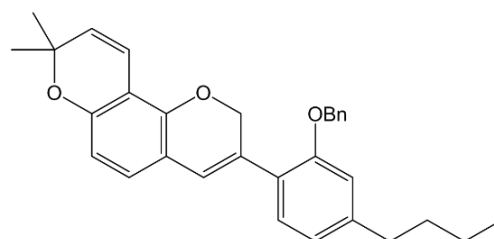
<Compound 5-28>
