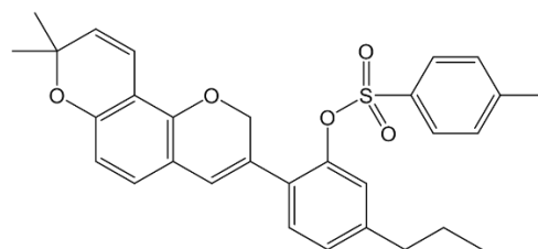
<Compound 5-40>
