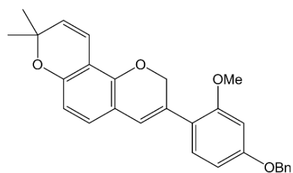
<Compound 5-12>
