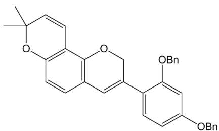
<Compound 5-11>
