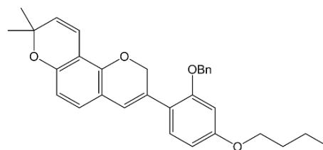
<Compound 5-6>
