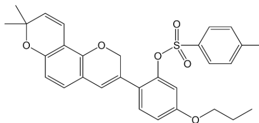
<Compound 5-42>
