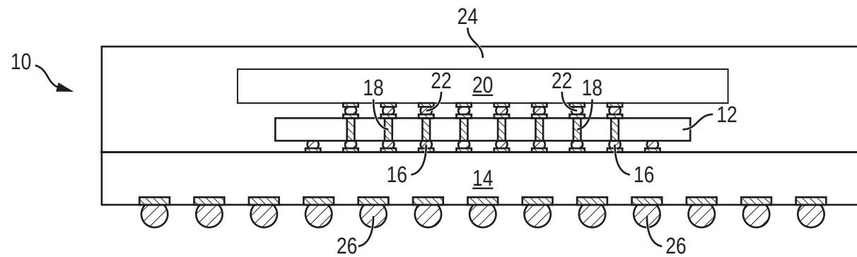
FIG. 1 (PRIOR ART)
